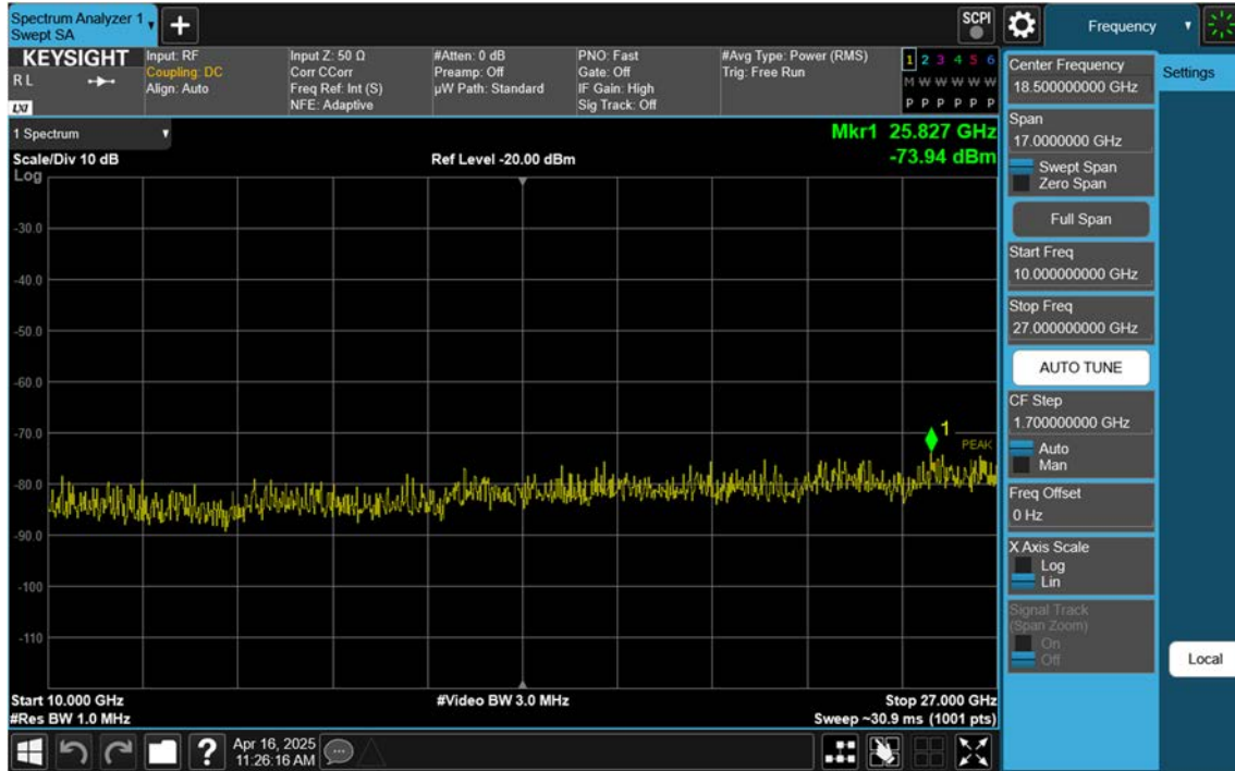
NR41_90 M_Conducted Spurious(Above10 G)_Low_BPSK_1RB
