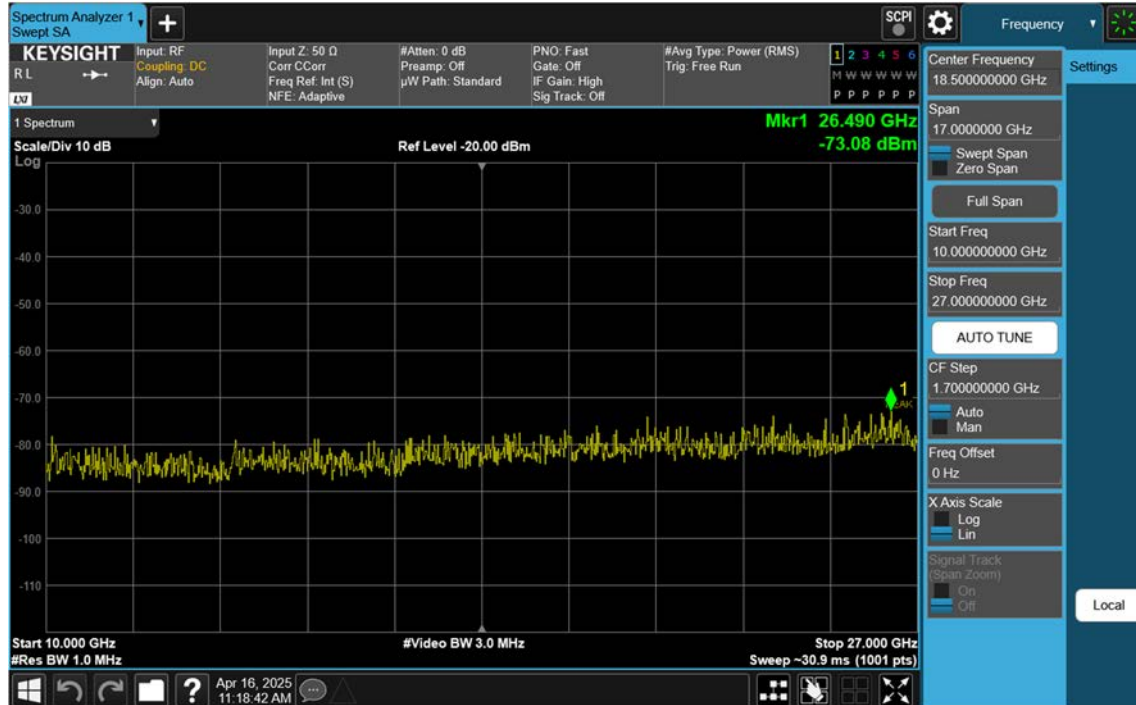
NR41_80 M_Conducted Spurious(Above10 G)_High_BPSK_1RB
