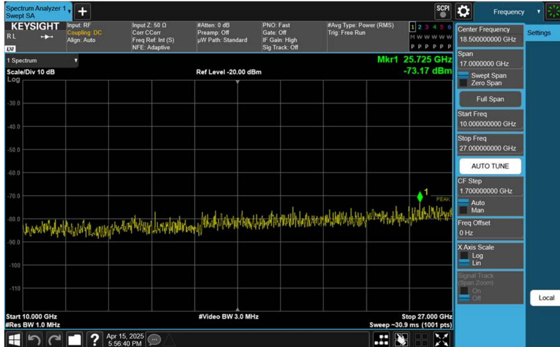
NR41_30 M_Conducted Spurious(Above10 G)_High_BPSK_1RB
