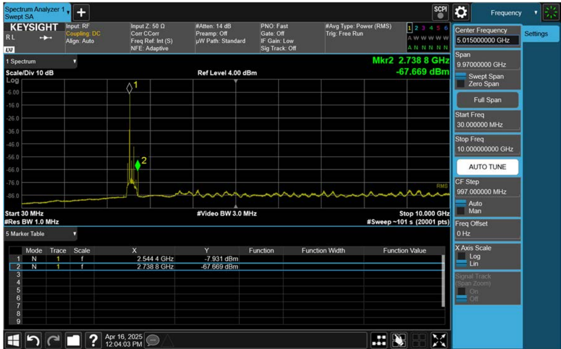
NR41_100 M_Conducted Spurious(30 M-10 G)_Mid_BPSK_1RB
