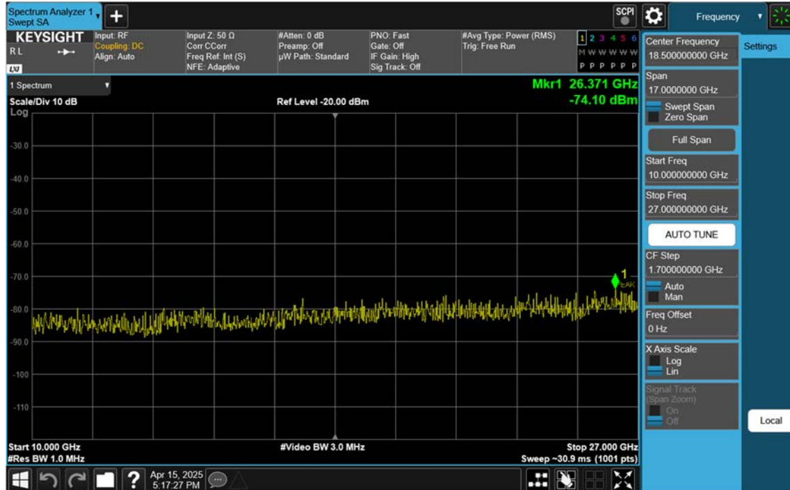
NR41_20 M_Conducted Spurious(Above10 G)_High_BPSK_1RB
