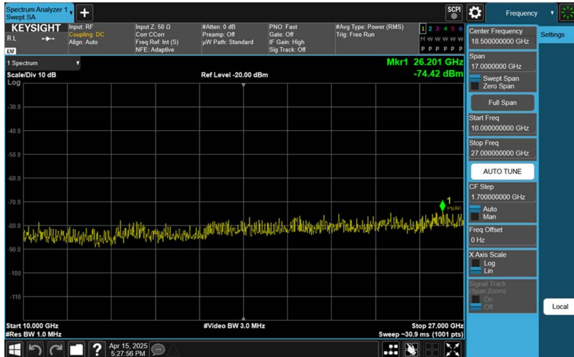
NR41_25 M_Conducted Spurious(Above10 G)_High_BPSK_1RB
