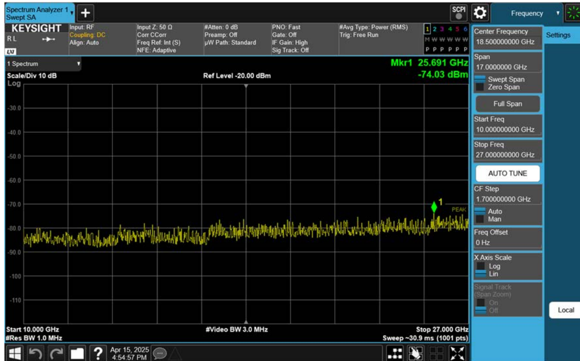
NR41_10 M_Conducted Spurious(Above10 G)_High_BPSK_1RB
