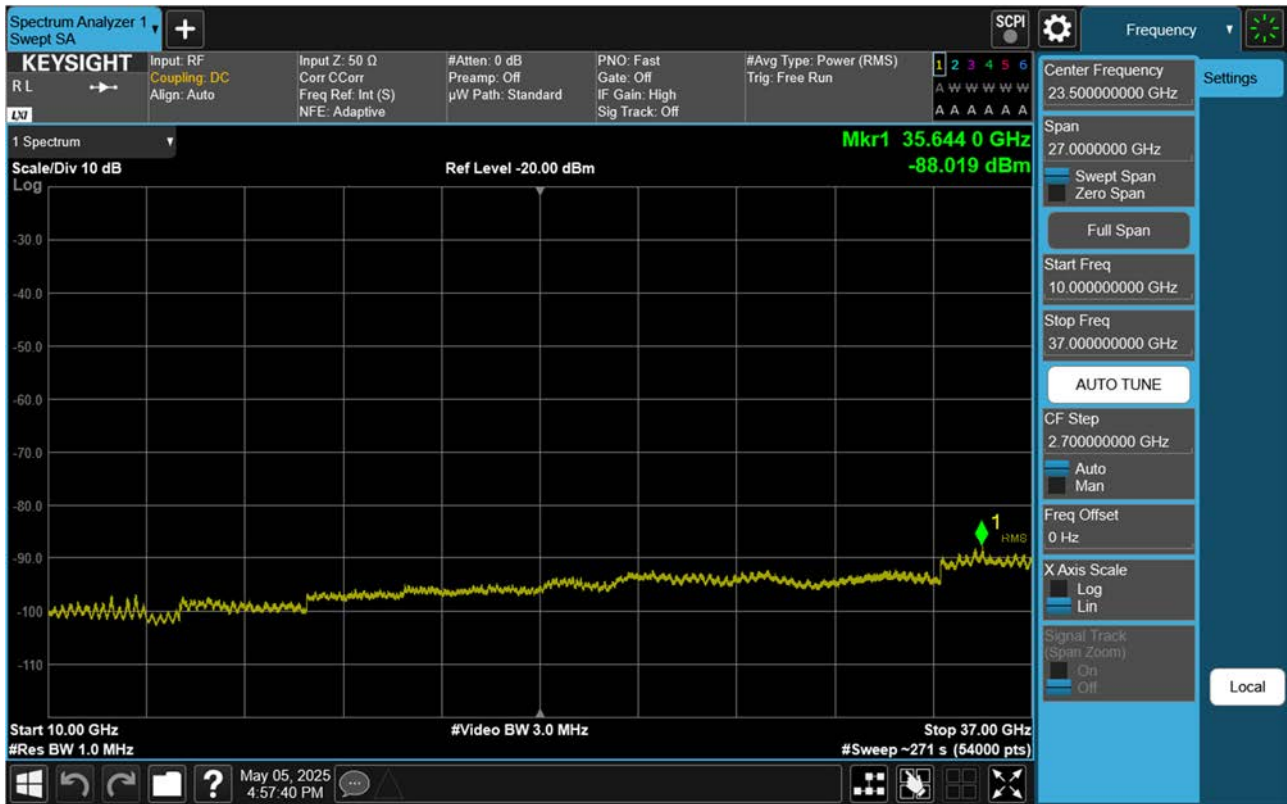
Sub6 n48. Conducted Spurious Plot 2 (20 MHz Ch. 646000 BPSK RB 1, Offset 1)
