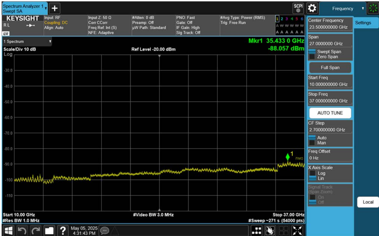
Sub6 n48. Conducted Spurious Plot 2 (20 MHz Ch. 637334 BPSK RB 1, Offset 1)
