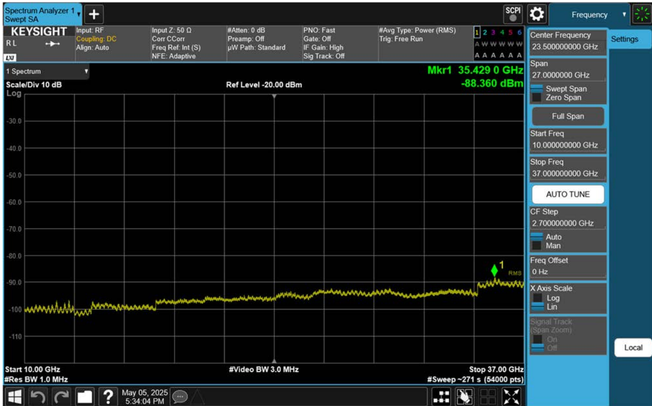
Sub6 n48. Conducted Spurious Plot 2 (30 MHz Ch. 645666 BPSK RB 1, Offset 1)
