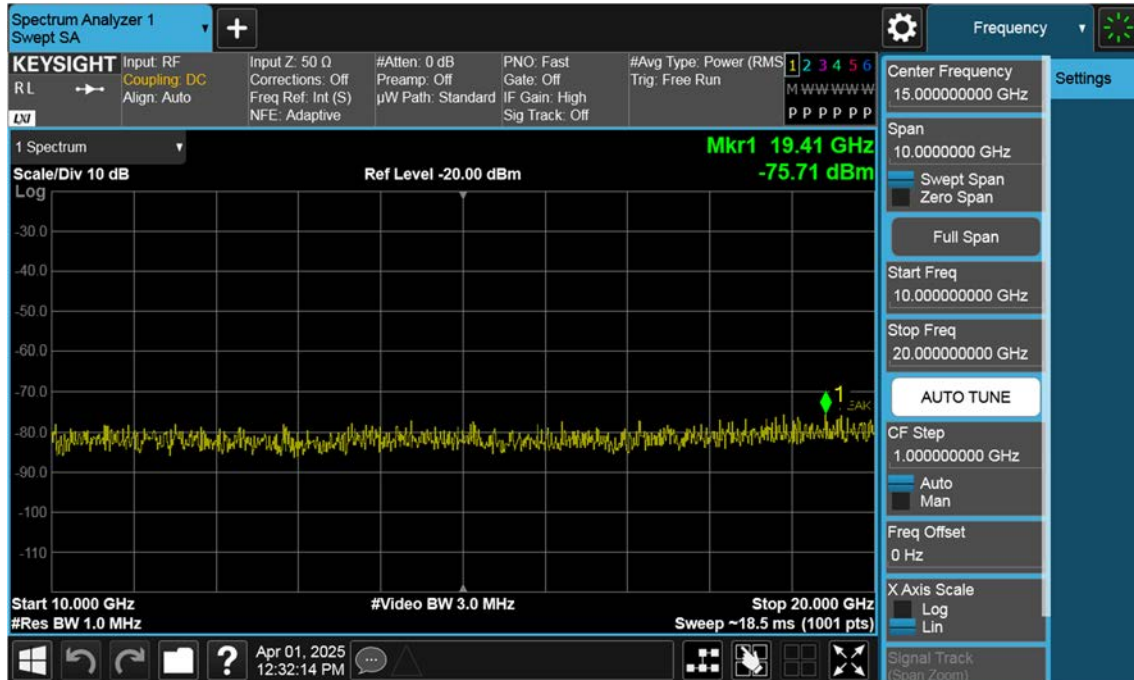
Sub_NR66_30 M_Conducted Spurious(Above10 G)_High_BPSK_1RB
