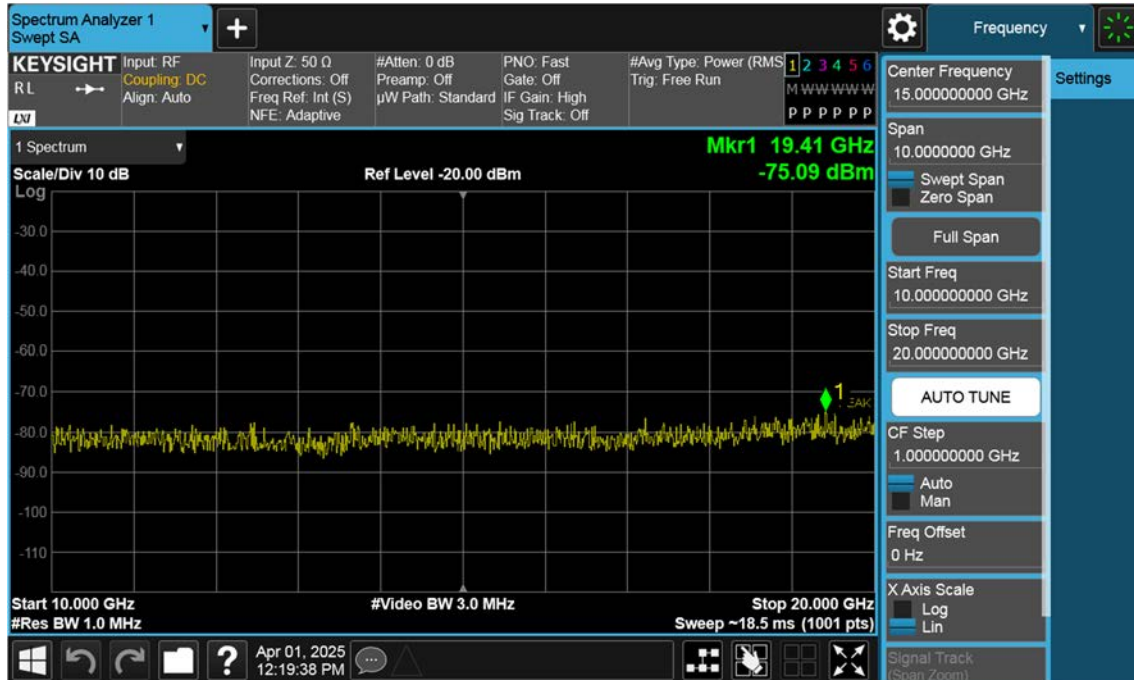
Sub_NR66_25 M_Conducted Spurious(Above10 G)_Low_BPSK_1RB
