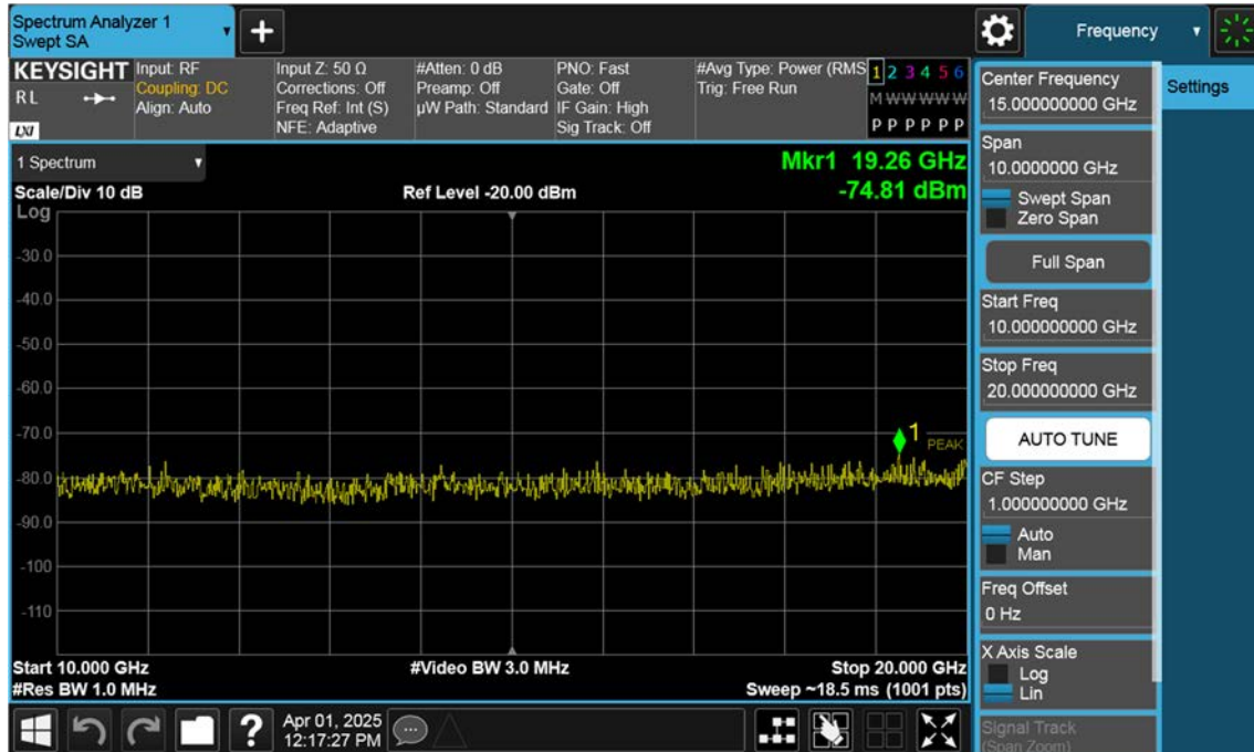
Sub_NR66_20 M_Conducted Spurious(Above10 G)_High_BPSK_1RB
