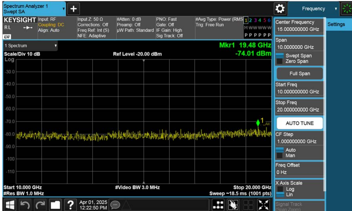
Sub_NR66_25 M_Conducted Spurious(Above10 G)_Mid_BPSK_1RB
