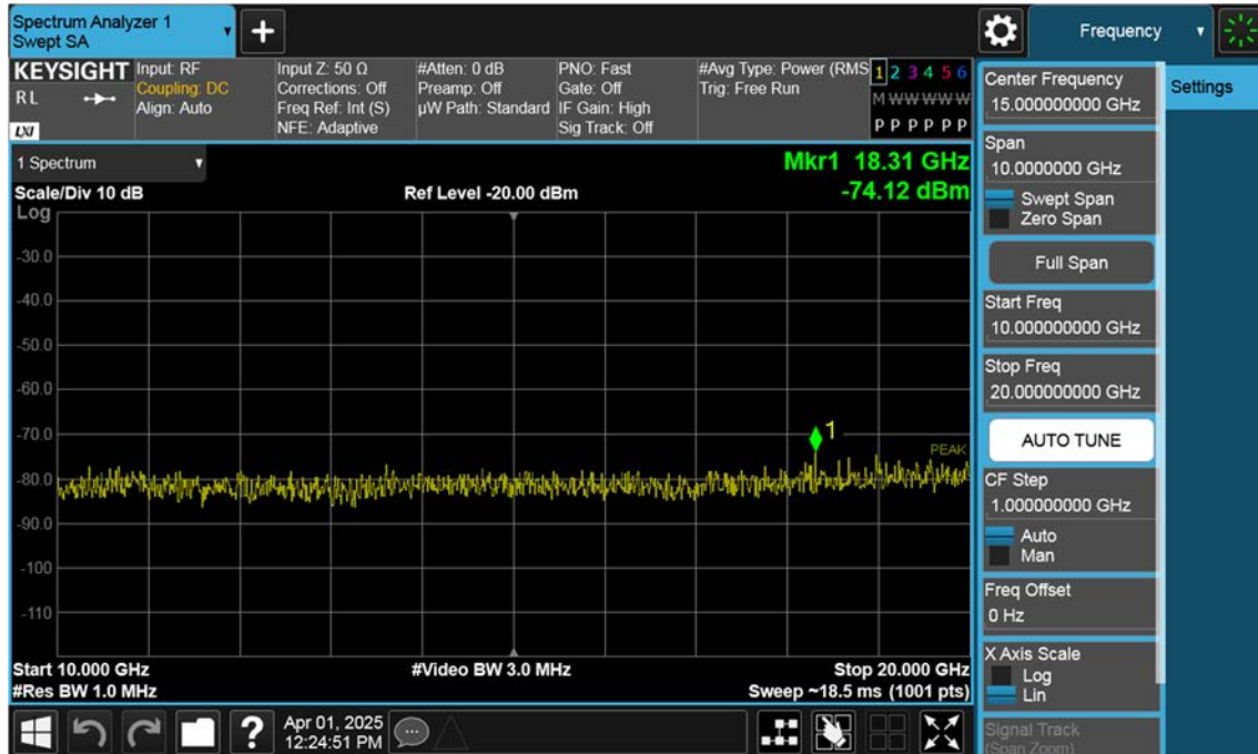
Sub_NR66_25 M_Conducted Spurious(Above10 G)_High_BPSK_1RB
