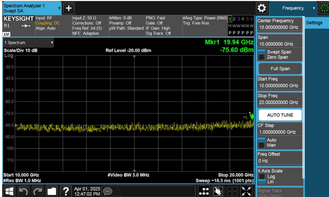
Sub_NR66_40 M_Conducted Spurious(Above10 G)_High_BPSK_1RB
