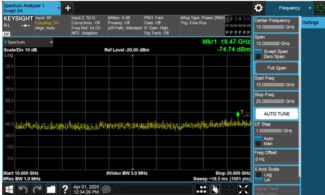
Sub_NR66_35 M_Conducted Spurious(Above10 G)_Low_BPSK_1RB
