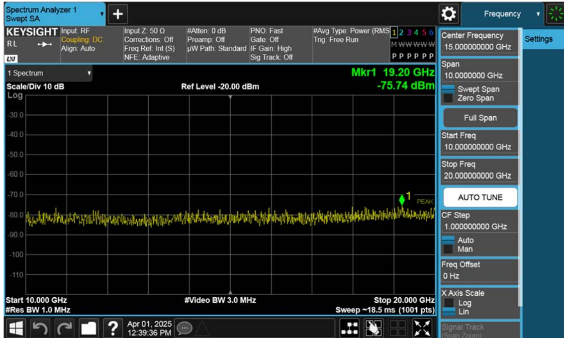
Sub_NR66_35 M_Conducted Spurious(Above10 G)_High_BPSK_1RB
