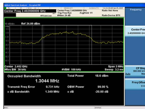
Dual ANT. 1 \pi/4 DQPSK 20 dB BW & 99% OBW (Ch. 0)
