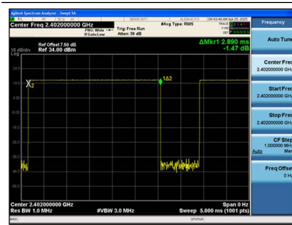
ANT.1 8DPSK : Dwell Time(Ch. 0)
