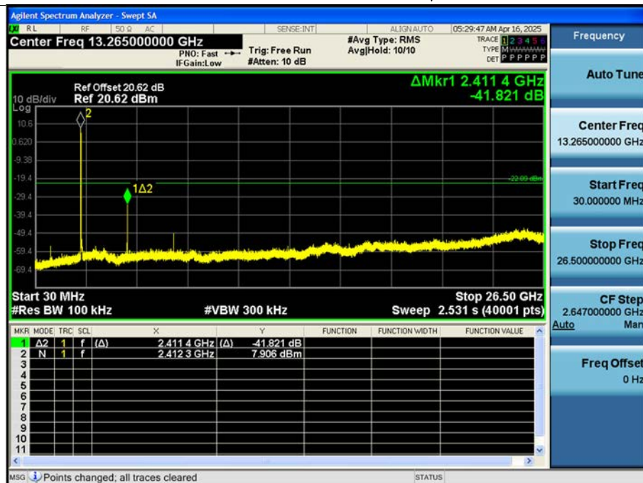
[ANT. 2] 802.11b_Ch.1, 1 Mbps
