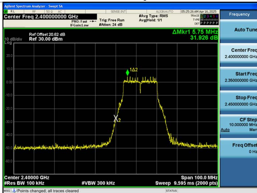
[ANT. 2] 802.11g - CH 1
