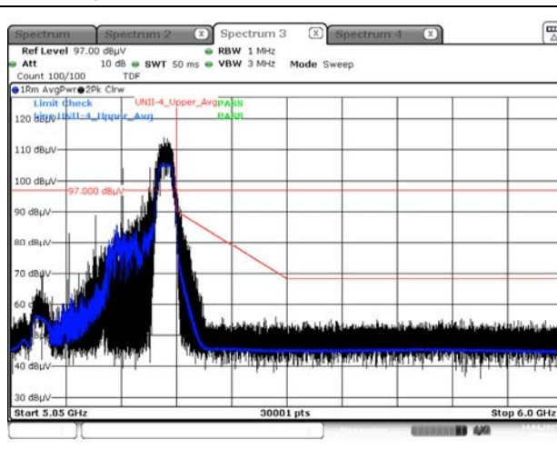
Average result (802.11ax(HE40) Ch.175, 52T RU 44)
