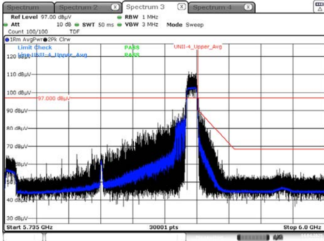
Average result (802.11ax(HE160_80U) Ch.163, 106T RU 60)
