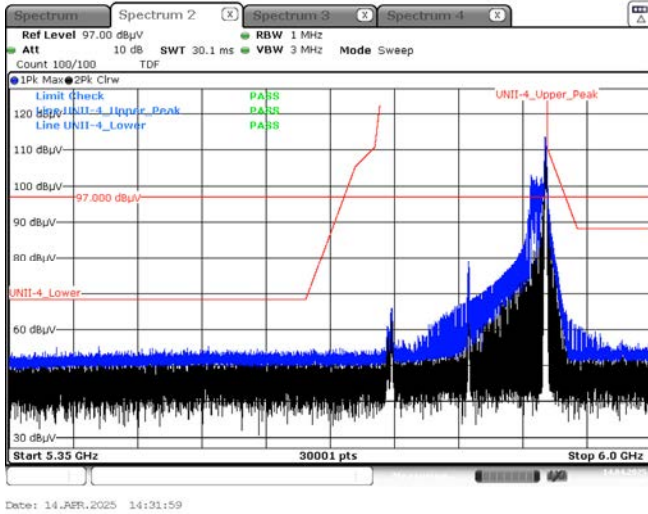
Peak result (802.11ax(HE160_80U) Ch.163, 106T RU 60)
