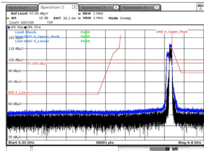
Peak result (802.11ax(HE20) Ch.177, 106T RU 54)
