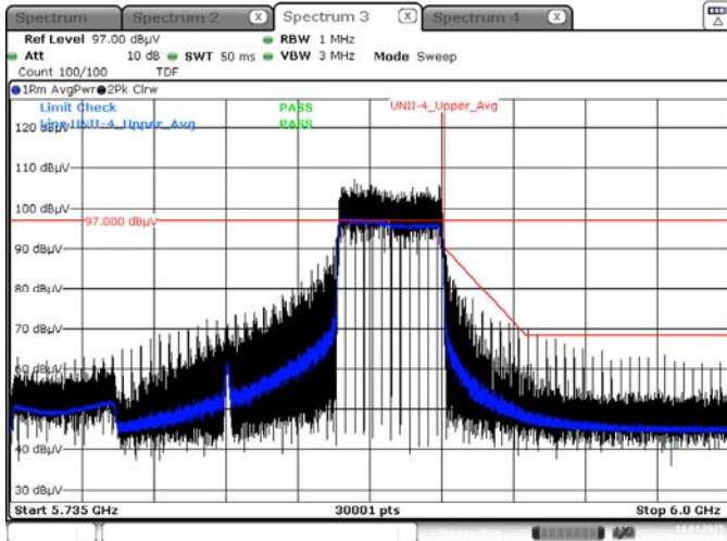
Average result (802.11ax(HE160_80U) Ch.163, 484T RU 66)
