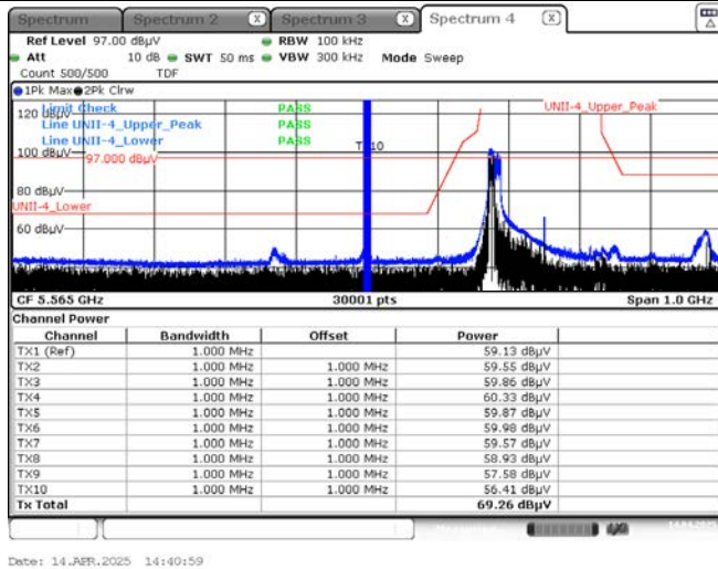
Peak result (802.11ax(HE160_80L) Ch.163, 484T RU 65)
