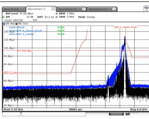
Peak result (802.11ax(HE80) Ch.171, 52T RU 52)
