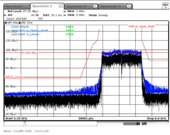
Peak result (802.11ax(HE160) Ch.163, SU)
