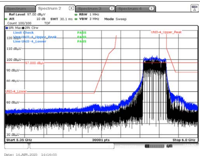
Peak result (802.11ax(HE160_80U) Ch.163, 996T RU 67)
