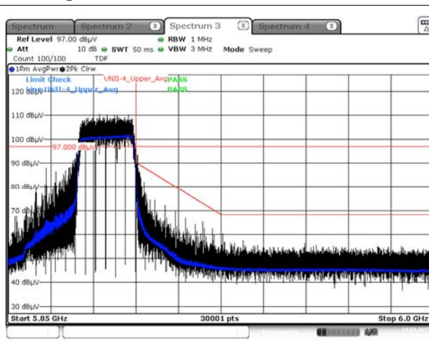
Average result (802.11ax(HE40) Ch.175, 242T RU 62)
