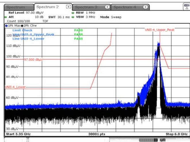
Peak result (802.11ax(HE80) Ch.171, 106T RU 60)
