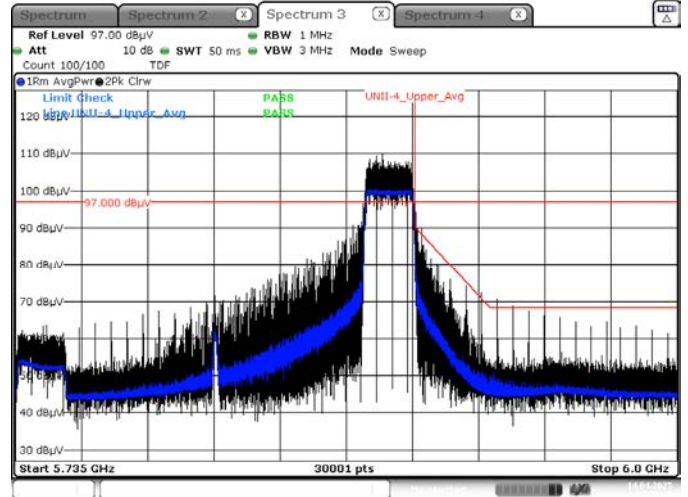
Average result (802.11ax(HE160_80U) Ch.163, 242T RU 64)
