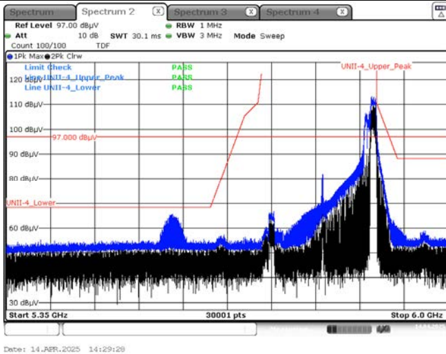
Peak result (802.11ax(HE160_80U) Ch.163, 484T RU 66)
