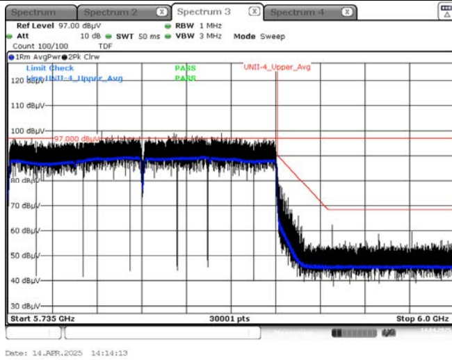
Average result (802.11ax(HE160) Ch.163, 2x996T RU 68)
