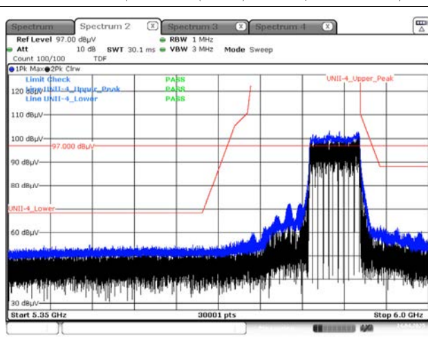
Peak result (802.11ax(HE80) Ch.171, 996T RU 67)
