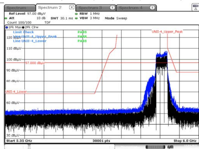
Peak result (802.11ax(HE80) Ch.171, 484T RU 66)
