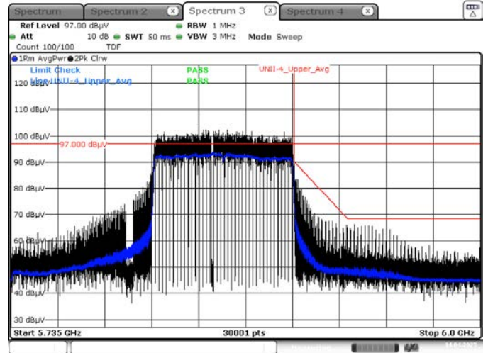
Average result (802.11ax(HE160_80U) Ch.163, 996T RU 67)
