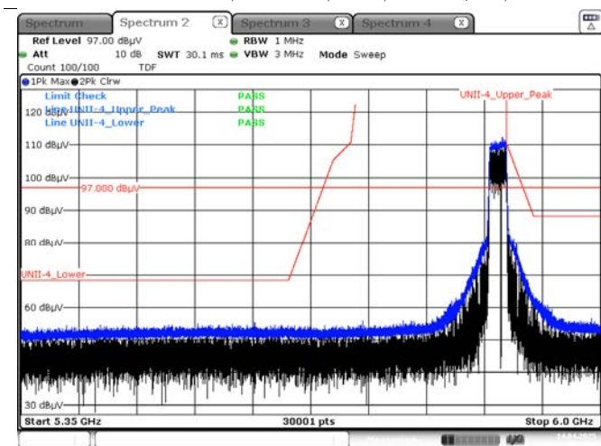
Peak result (802.11ax(HE20) Ch.177, SU)
