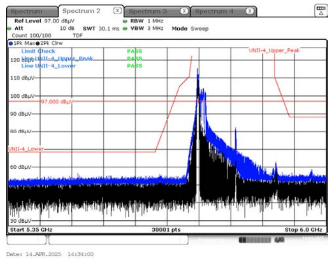
Peak result (802.11ax(HE160_80L) Ch.163, 242T RU 61)
