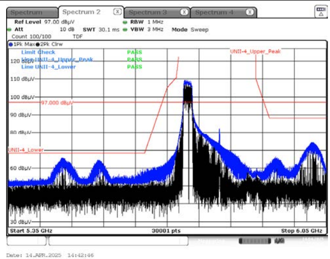
Peak result (802.11ax(HE160_80L) Ch.163, 996T RU 67)
