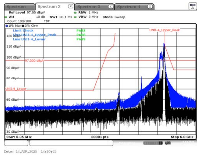
Peak result (802.11ax(HE160_80U) Ch.163, 242T RU 64)
