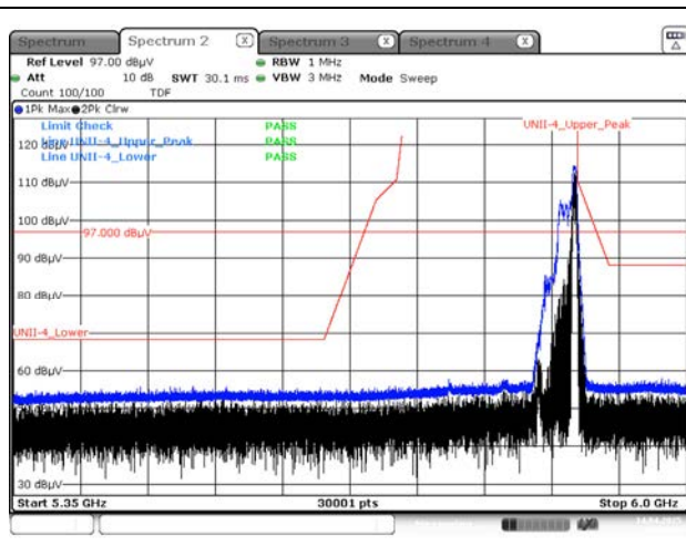
Peak result (802.11ax(HE40) Ch.175, 52T RU 44)
