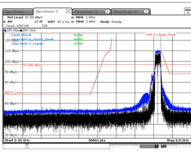
Peak result (802.11ax(HE40) Ch.175, 242T RU 62)
