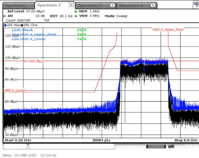
Peak result (802.11ax(HE160) Ch.163, 2x996T RU 68)
