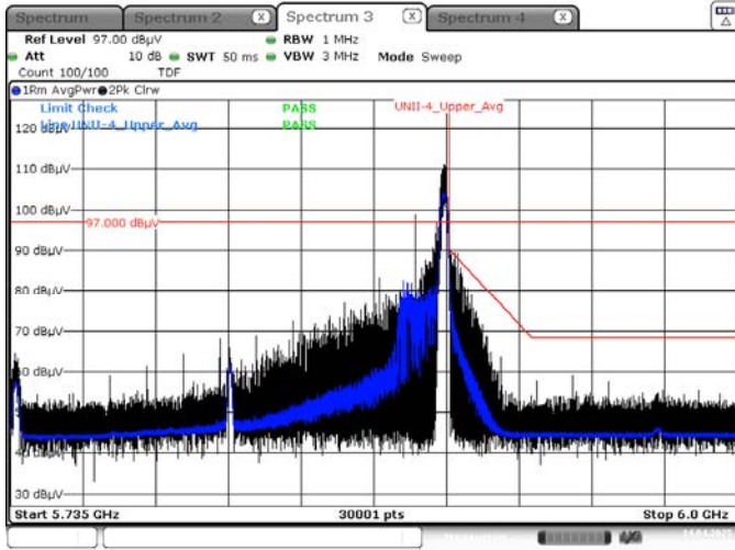
Average result (802.11ax(HE160_80U) Ch.163, 26T RU 36)
