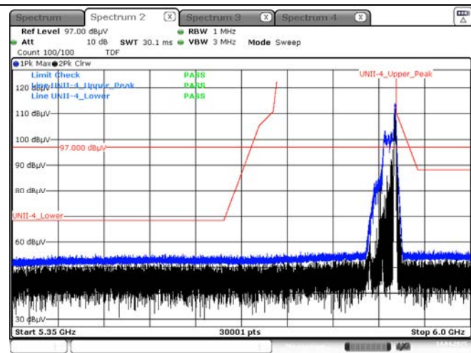
Peak result (802.11ax(HE40) Ch.175, 26T RU 17)
