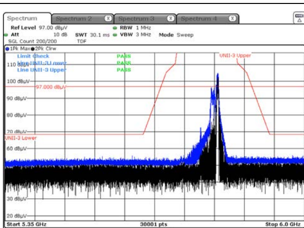
Peak result (802.11ax(HE80) Ch.155, 52T RU 52)
