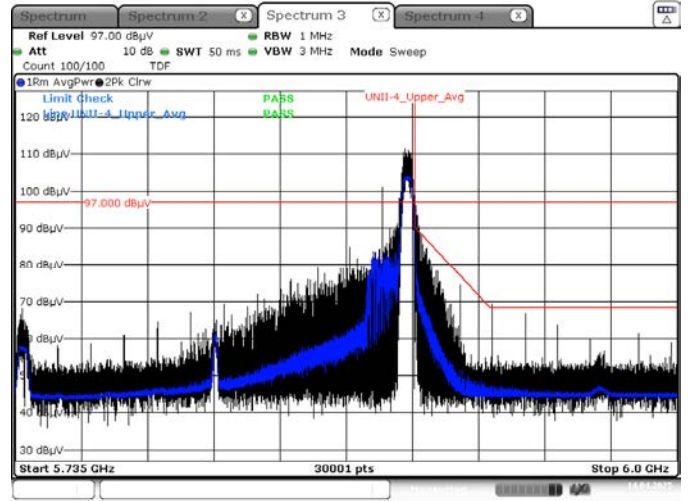
Average result (802.11ax(HE160_80U) Ch.163, 52T RU 52)
