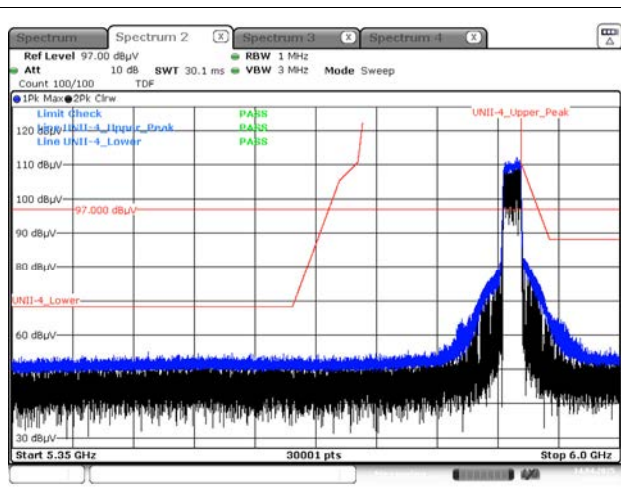
Peak result (802.11ax(HE20) Ch.177, 242T RU 61)
