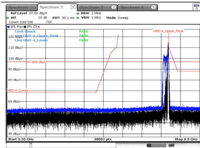
Peak result (802.11ax(HE20) Ch.177, 26T RU 8)
