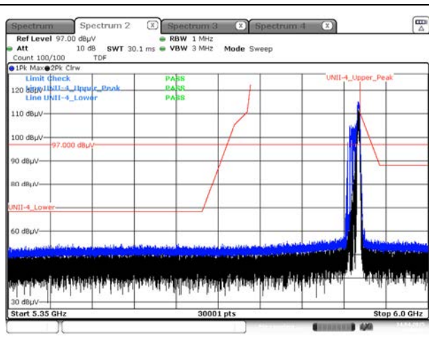
Peak result (802.11ax(HE20) Ch.177, 52T RU 40)
