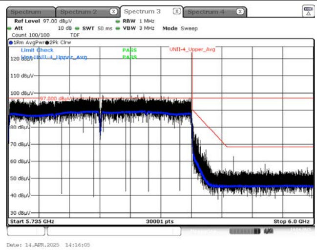
Average result (802.11ax(HE160) Ch.163, SU)
