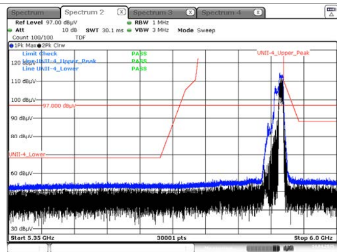
Peak result (802.11ax(HE40) Ch.175, 106T RU 56)
