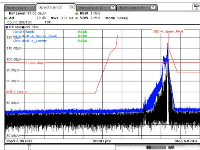
Peak result (802.11ax(HE80) Ch.171, 26T RU 36)
