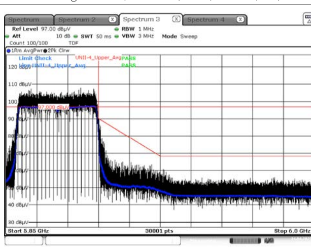
Average result (802.11ax(HE40) Ch.175, SU)
