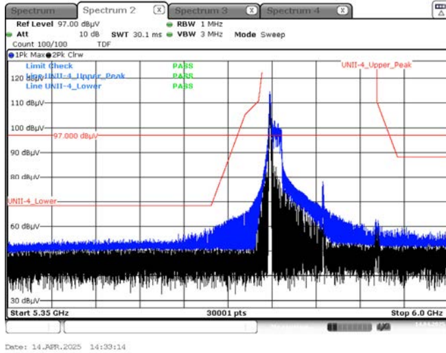
Peak result (802.11ax(HE160_80L) Ch.163, 106T RU 53)
