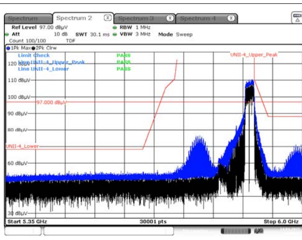
Peak result (802.11ax(HE80) Ch.171, 242T RU 64)
