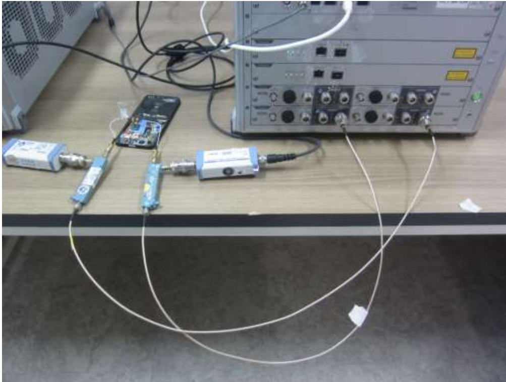
Test setup photo-8 TC16
