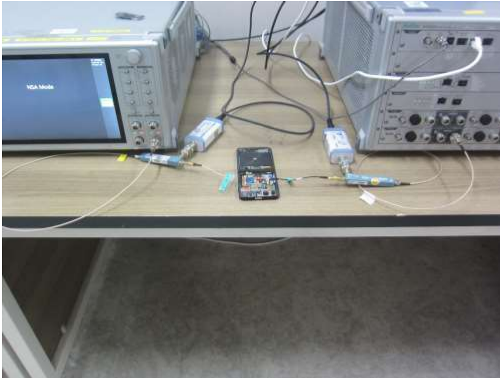
Test setup photo-9 TC17
