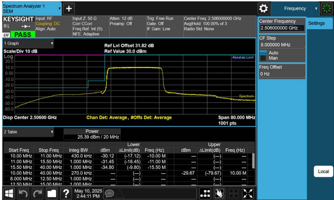
LTE B41_20 M_Channel Edge_Lower_Low_QPSK_FullRB
