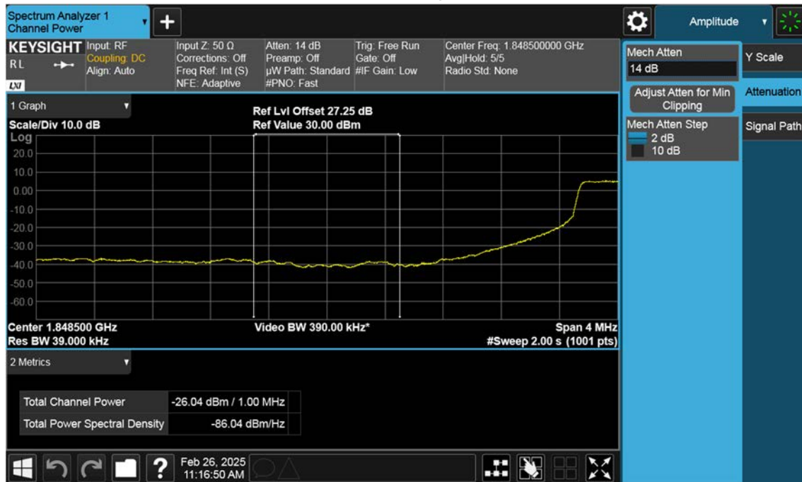
NR25_5 M_Extended Band Edge_Low_BPSK_FullRB
