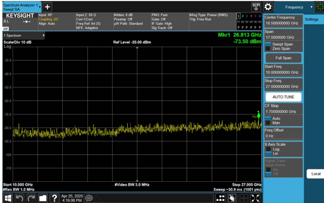
NR41_70 M_Conducted Spurious(Above10 G)_High_BPSK_1RB
