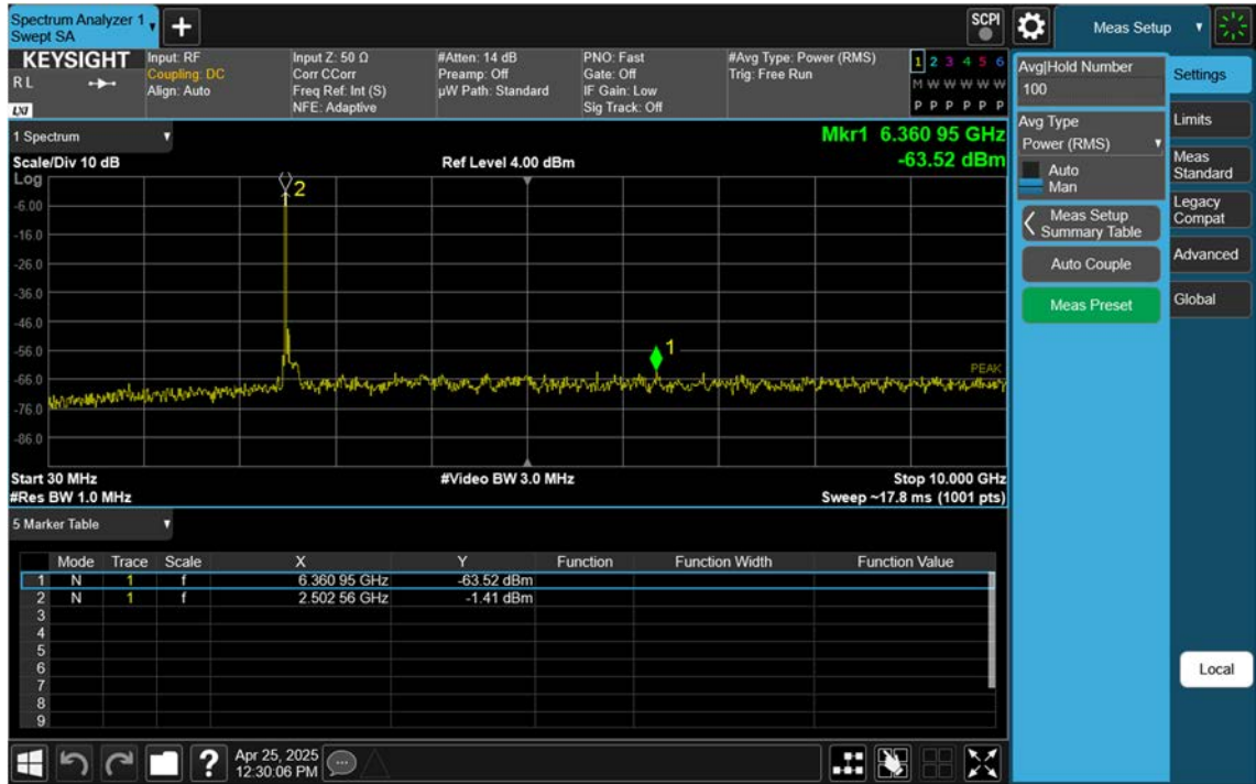
NR41_50 M_Conducted Spurious(30 M-10 G)_Low_BPSK_1RB
