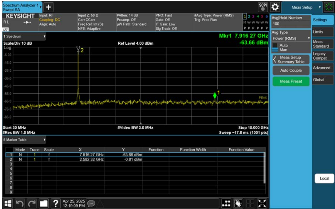
NR41_30 M_Conducted Spurious(30 M-10 G)_Mid_BPSK_1RB
