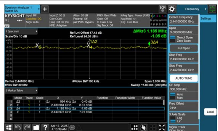
Dual ANT. 2 \pi /4DQPSK : Channel Separation
