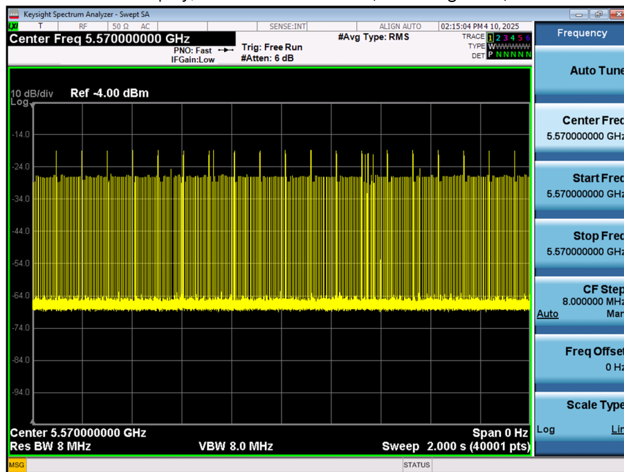
Time Display, WLAN Channel Traffic (Streaming Video)
