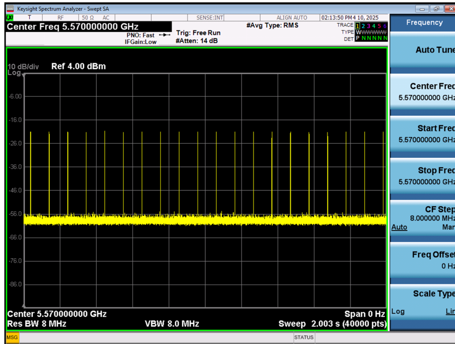
Time Display, Non WLAN Channel Traffic
