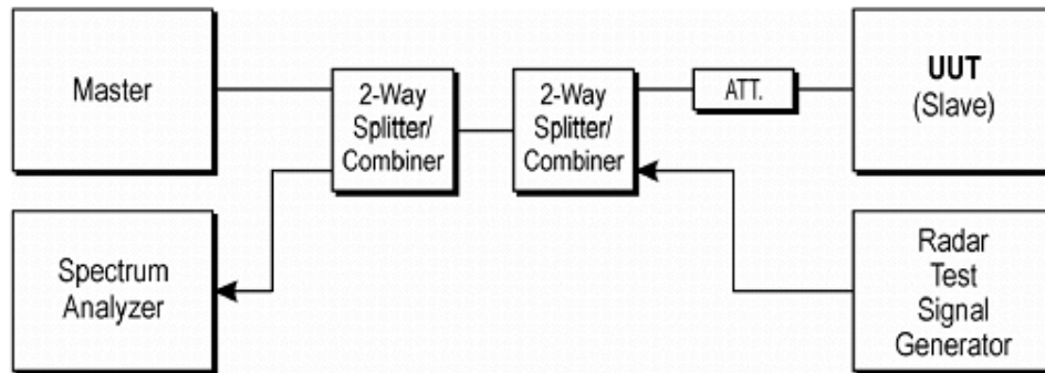
Figure 7-1. Test Setup
