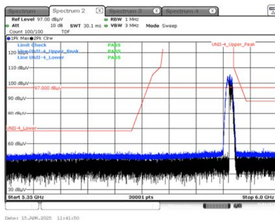
Peak Result (802.11ac_VHT20, Ch.177, X-H)
