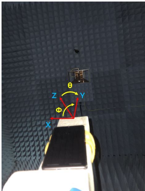
Figure 1: Geometry for SM-F766B for Radiation patterns.
