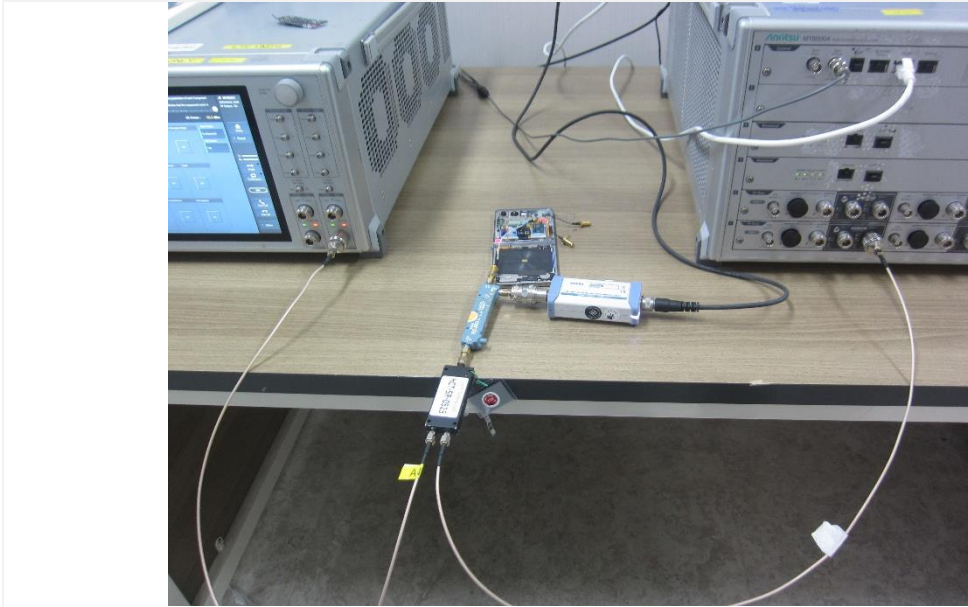
Test setup photo-3 TC 10
