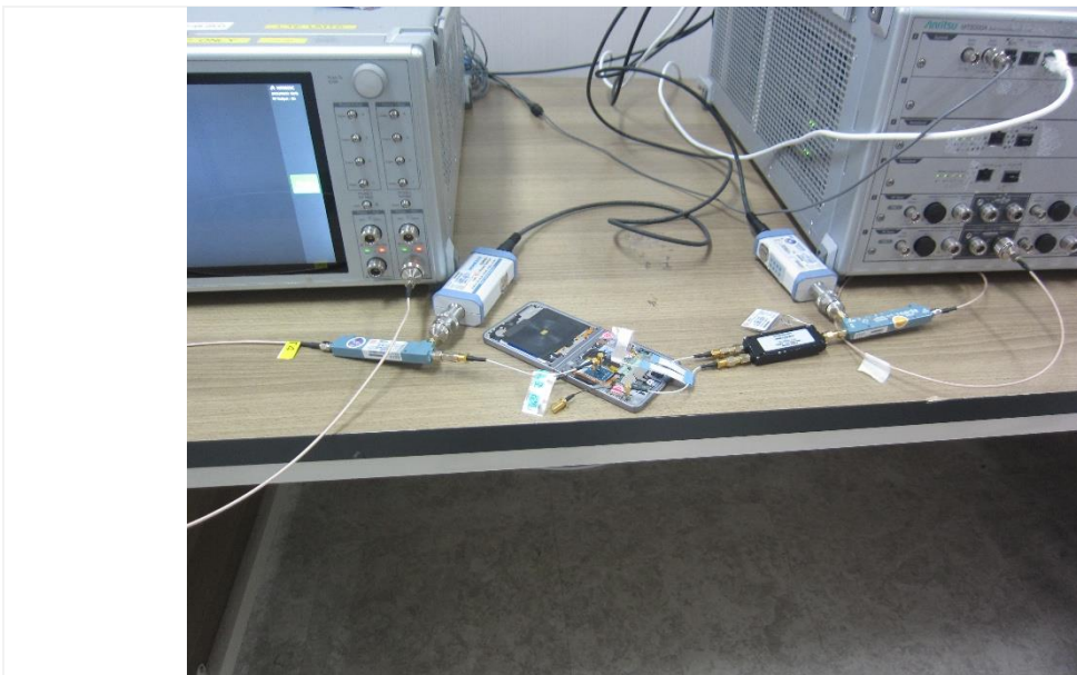
Test setup photo-5 TC16
