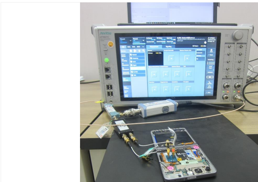
Test setup photo-4 TC11
