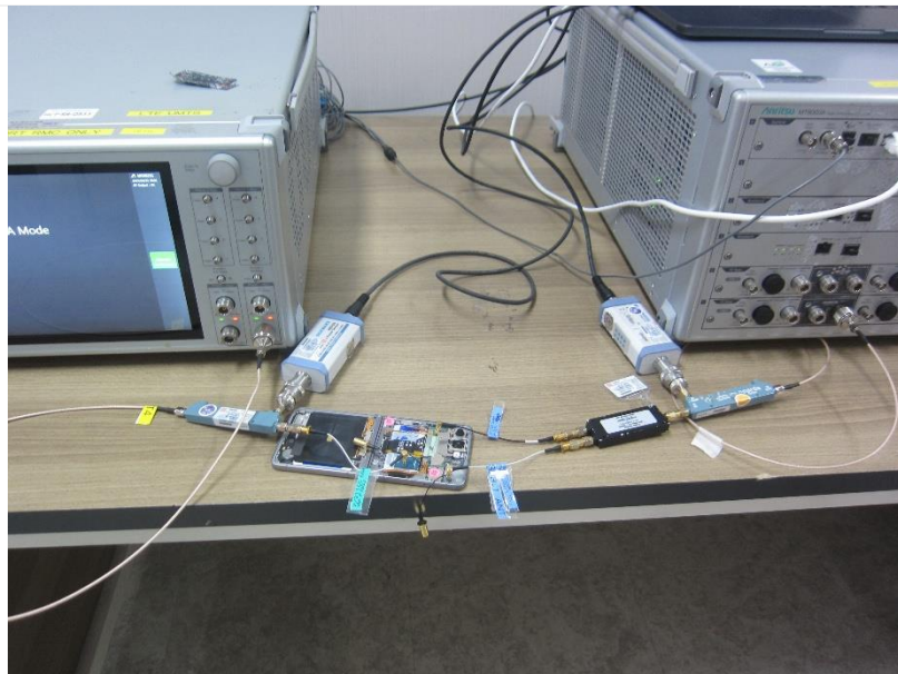
Test setup photo-5 TC14
