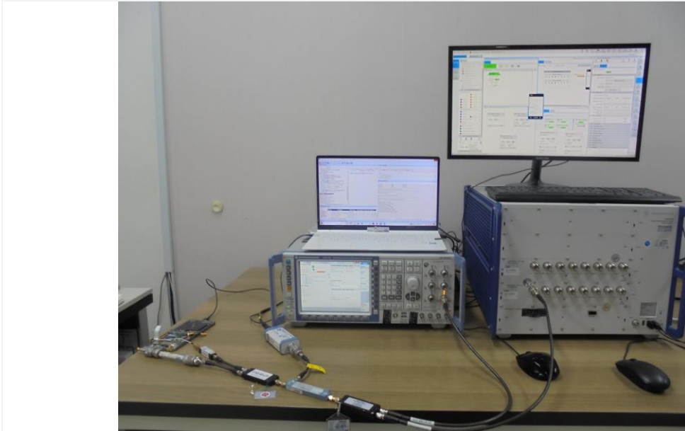
Test setup photo-3 (7-2(b) WLAN Change in Antenna/Band)
