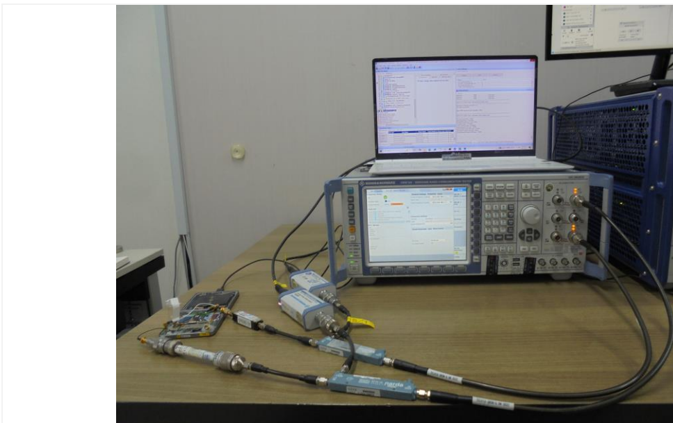
Test setup photo-2 (7-1(c) WLAN SAR1 vs SAR2 (DBS)/ WLAN Ant Switch)
