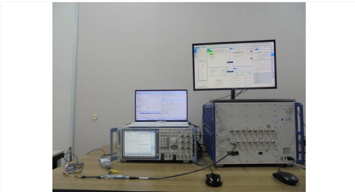
Test setup photo-2 (7-1(a) WLAN Time-varying Tx Power Transmission)
