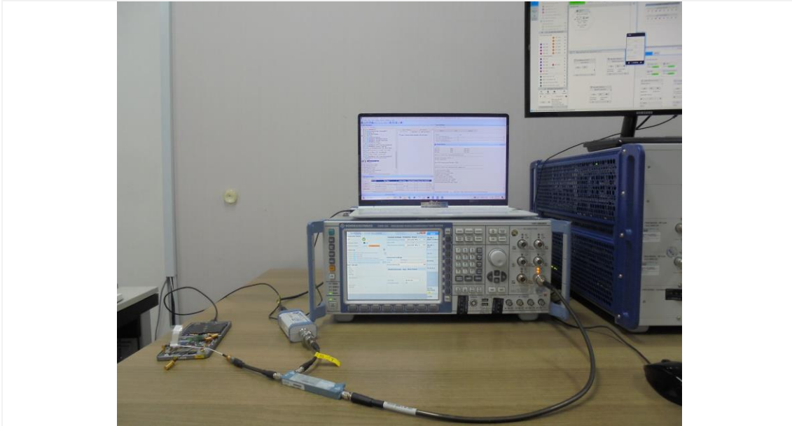
Test setup photo-1 (7-1(a) WLAN Time-varying Tx Power Transmission, Change in DSI)
