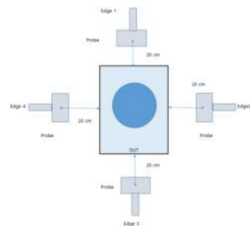
DUT to phone test Configuration 3 & 4
