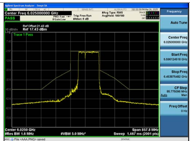
Bandwidth EHT160M, Ch.15(6025 MHz) 996T+484T RU94
