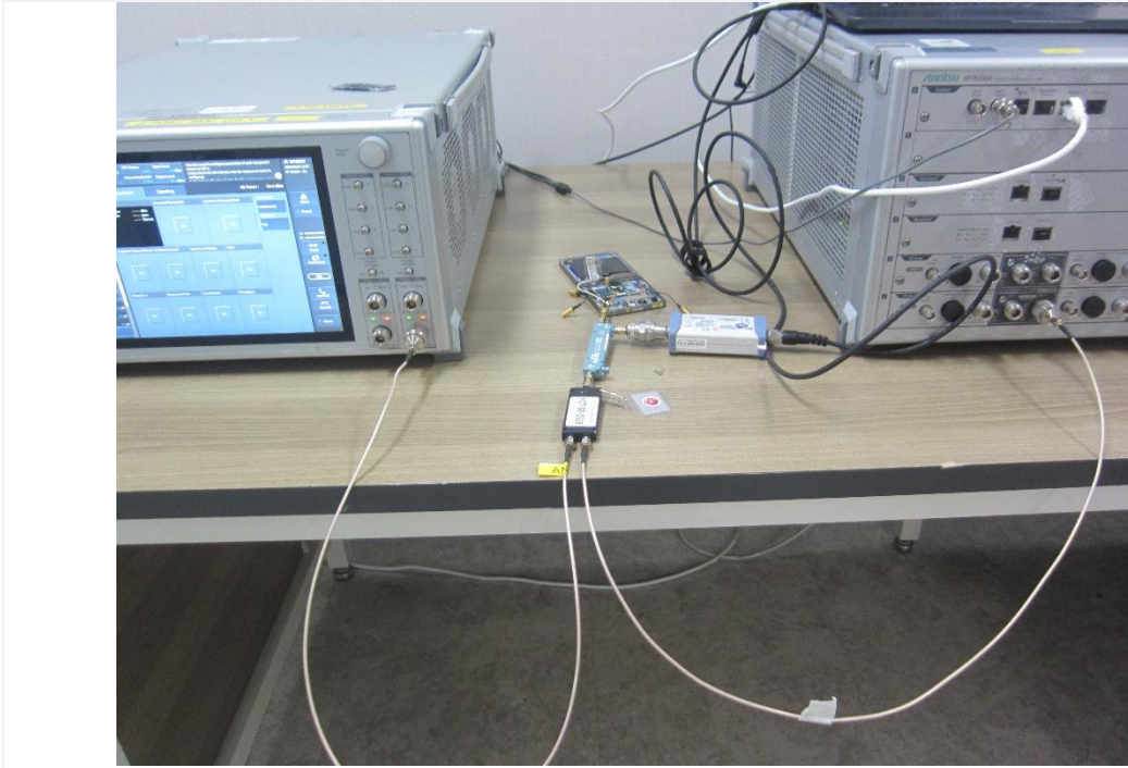
Test setup photo-3 TC10
