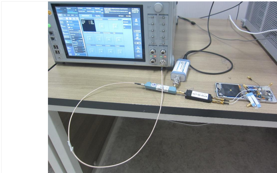
Test setup photo-4 TC11
