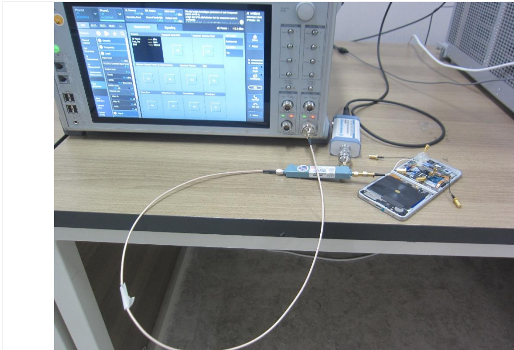
Test setup photo-1 TC01,03,04,05,07,08,09,15
