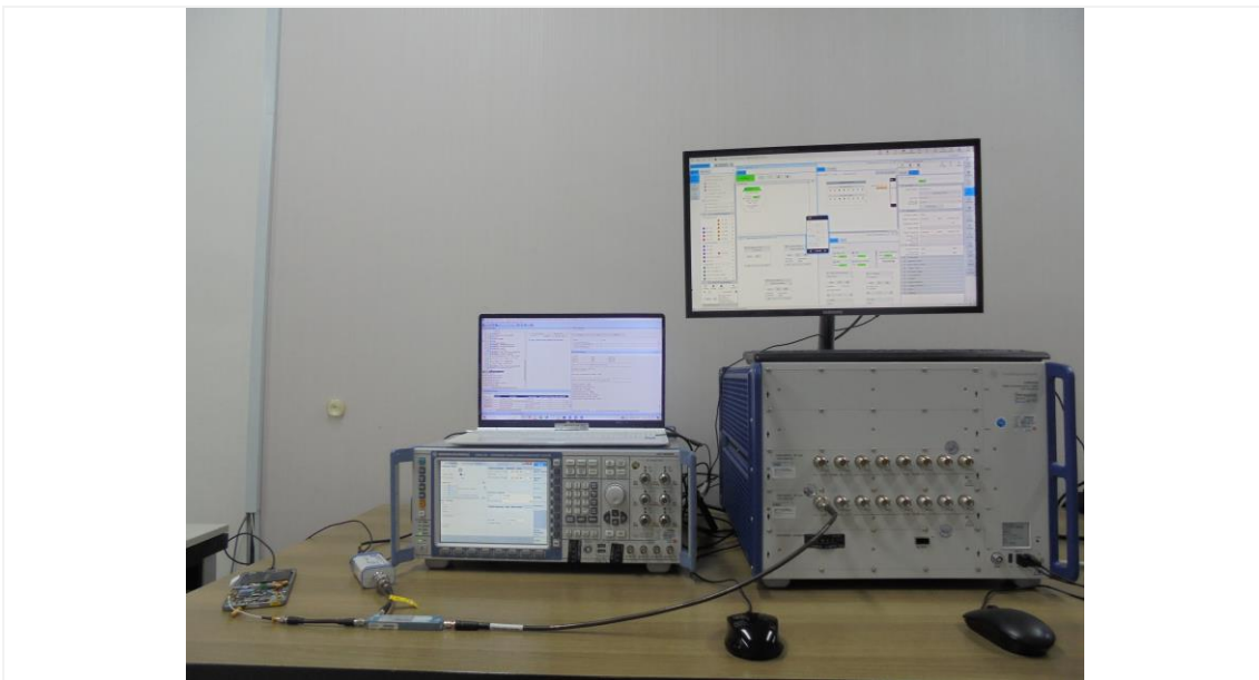
Test setup photo-2 (7-1(a) WLAN 6GHz Time-varying Tx Power Transmission)
