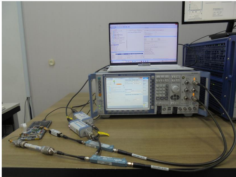
Test setup photo-4 (7-3(c) WLAN SAR1 vs SAR2 (DBS))
