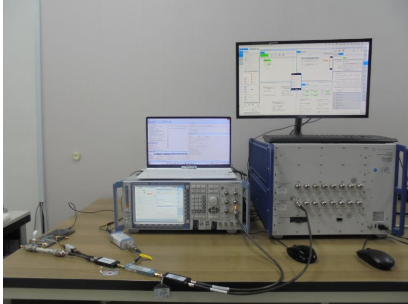
Test setup photo-3 (7-2(b) WLAN Change in Antenna/Band)
