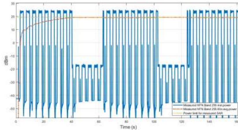
Figure 11.1-1 Conducted Tx power in NTN in test TC 1
