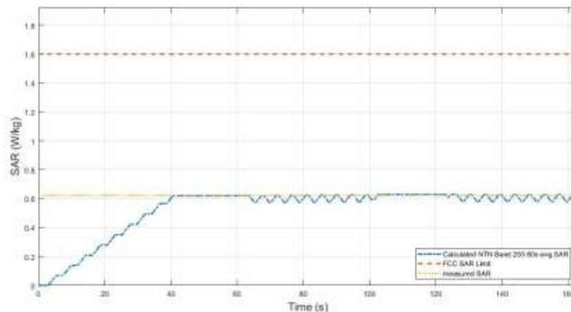
Figure 11.1-2 Total time-averaged SAR in TC17
