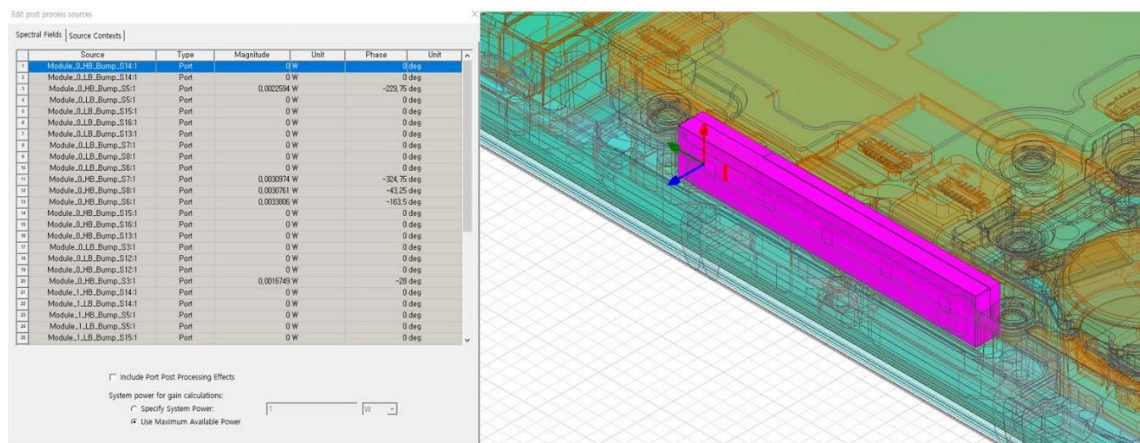
Figure 6. An example of port excitation (ANT K)
