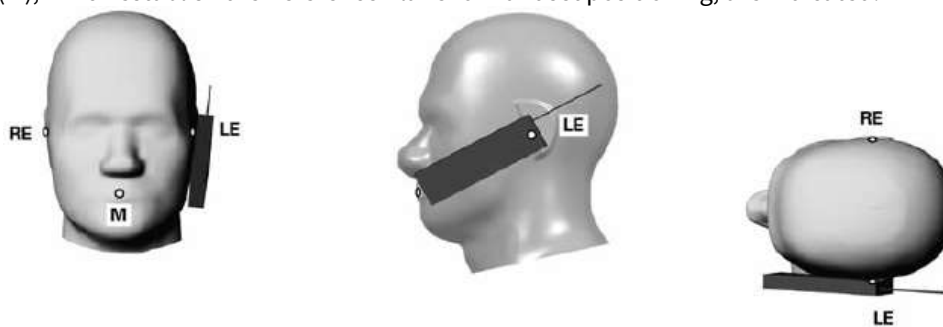
Figure 8.4 Touch/ Touch position of the wireless device
