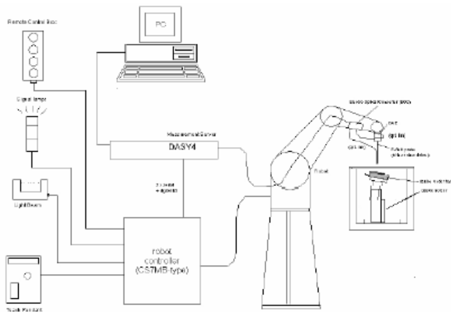
Figure 1. HAC Test Measurement Set-up
