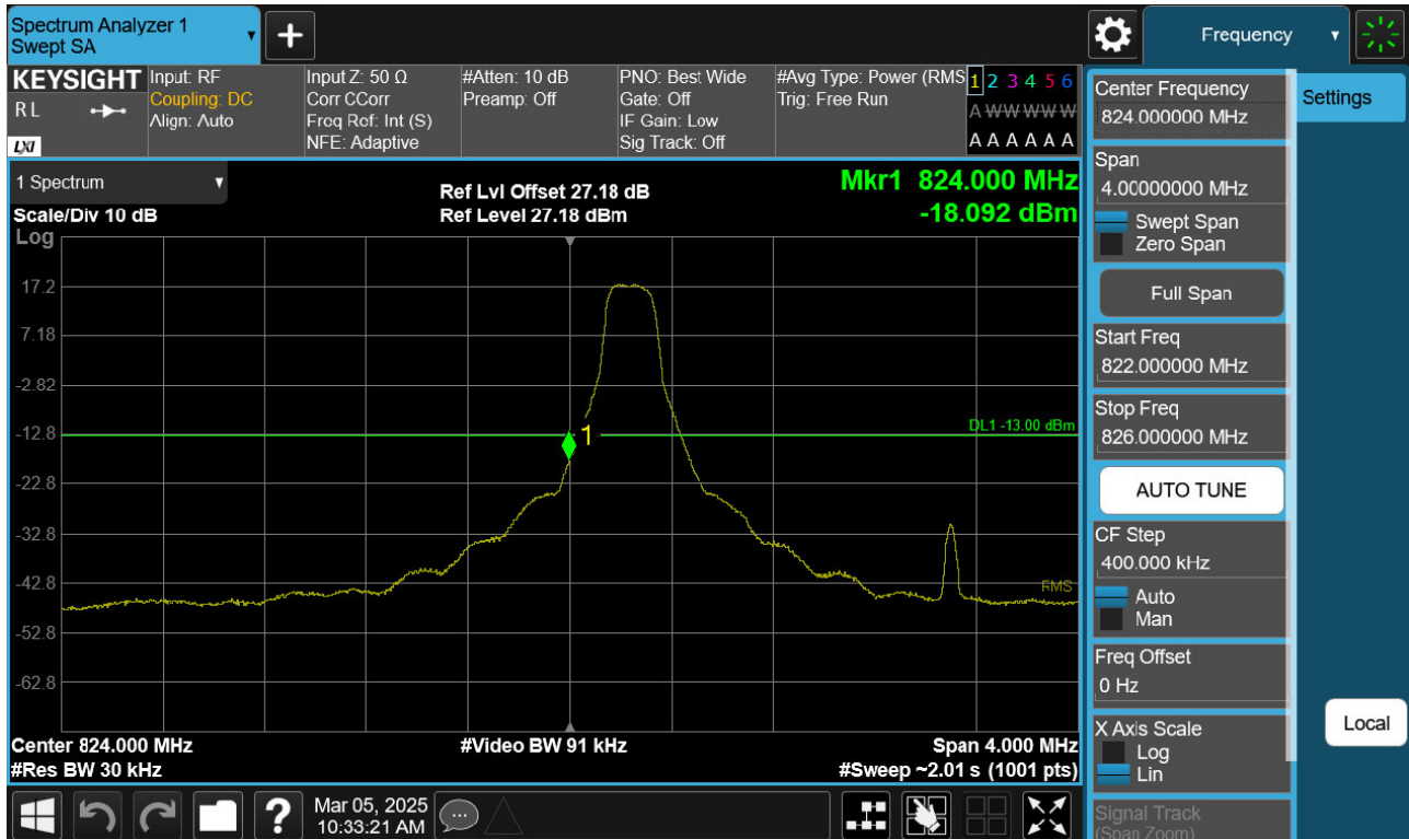
BAND 26. Lower Band Edge Plot (3 M BW Ch.26805 QPSK_RB1_Offset 0)
