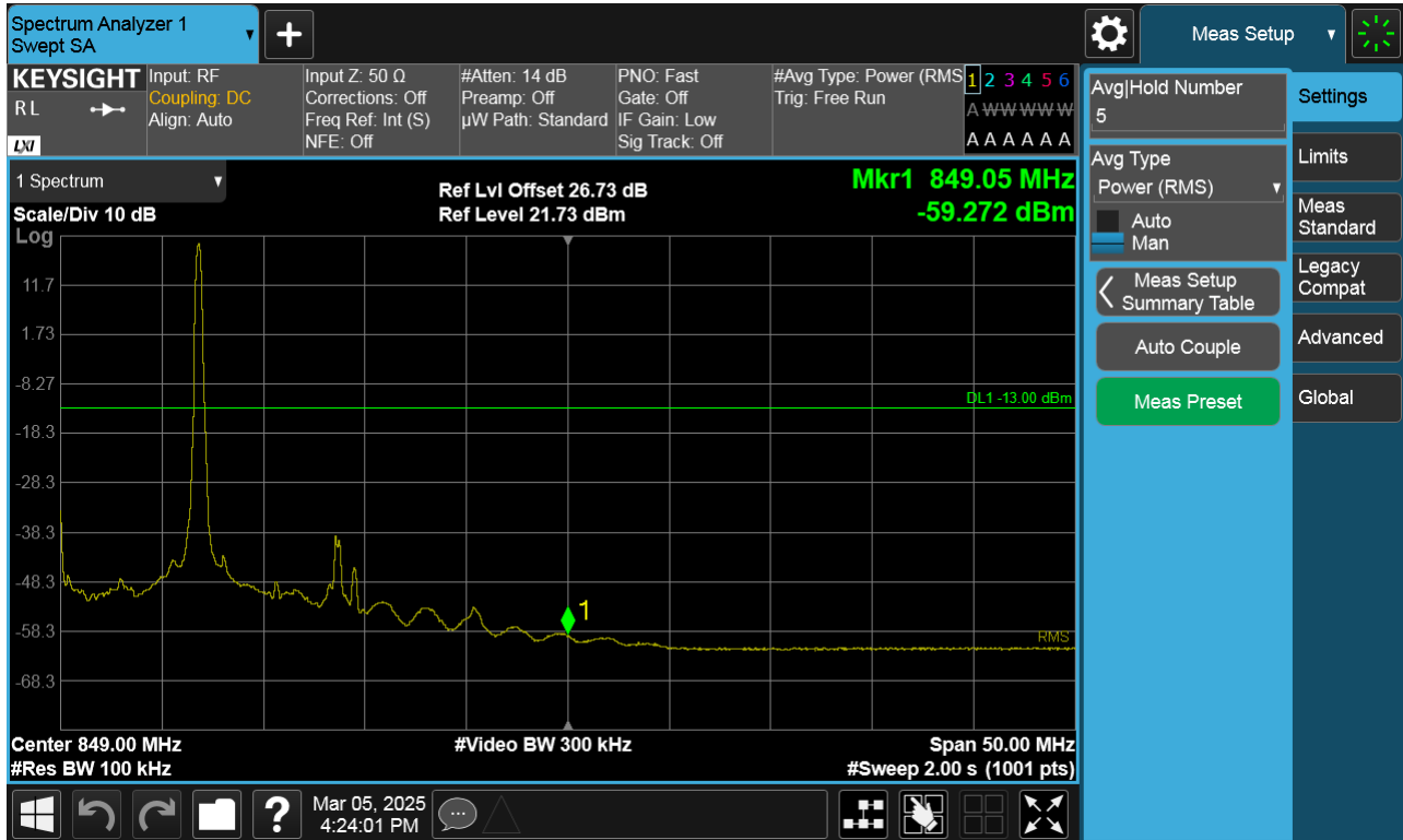
Sub6 n26. Upper Band Edge Plot (15 M BW Ch.164800 BPSK_RB1_Offset 78)
