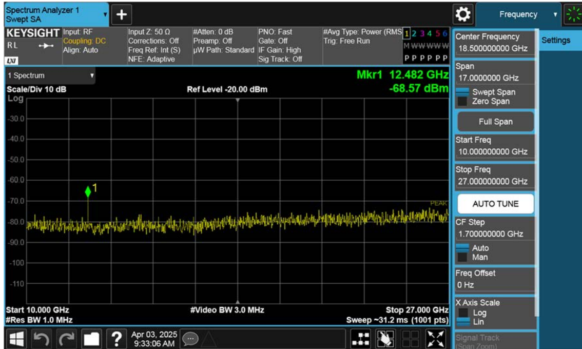
NR41_80 M_Conducted Spurious(Above10 G)_Low_BPSK_1RB
