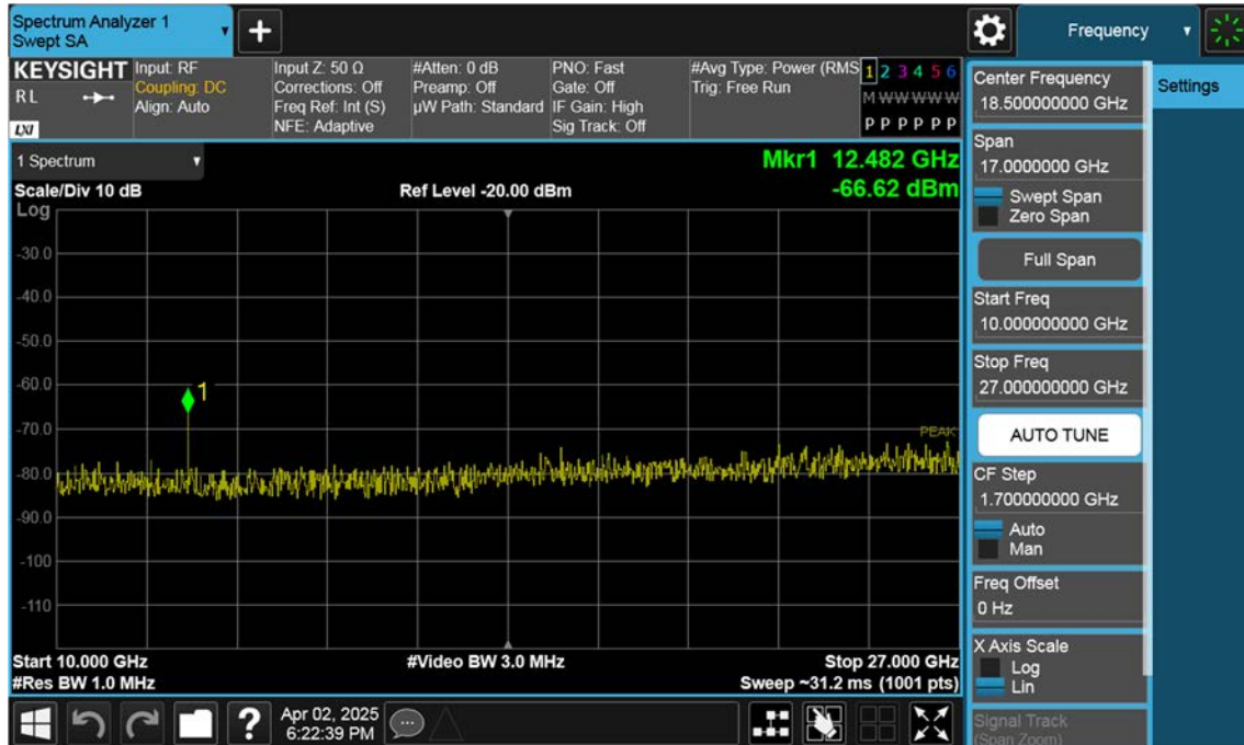
NR41_30 M_Conducted Spurious(Above10 G)_Low_BPSK_1RB
