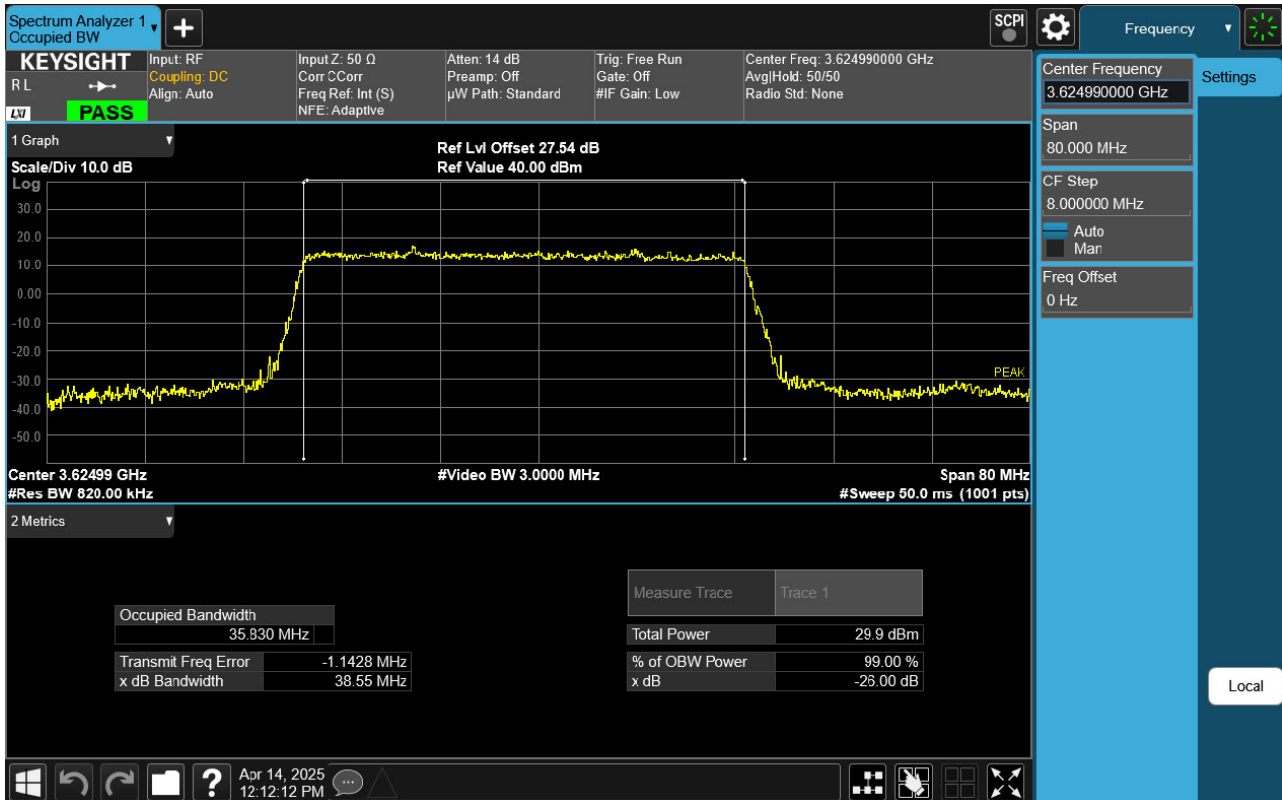
Sub6 n48. Occupied Bandwidth Plot (40 MHz Ch. 641666 BPSK RB 100)
