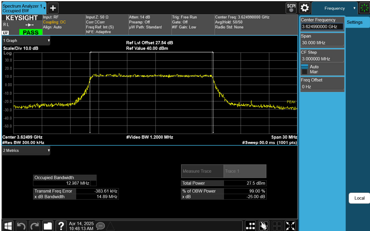
Sub6 n48. Occupied Bandwidth Plot (15 MHz Ch.641666 64-QAM RB 36)
