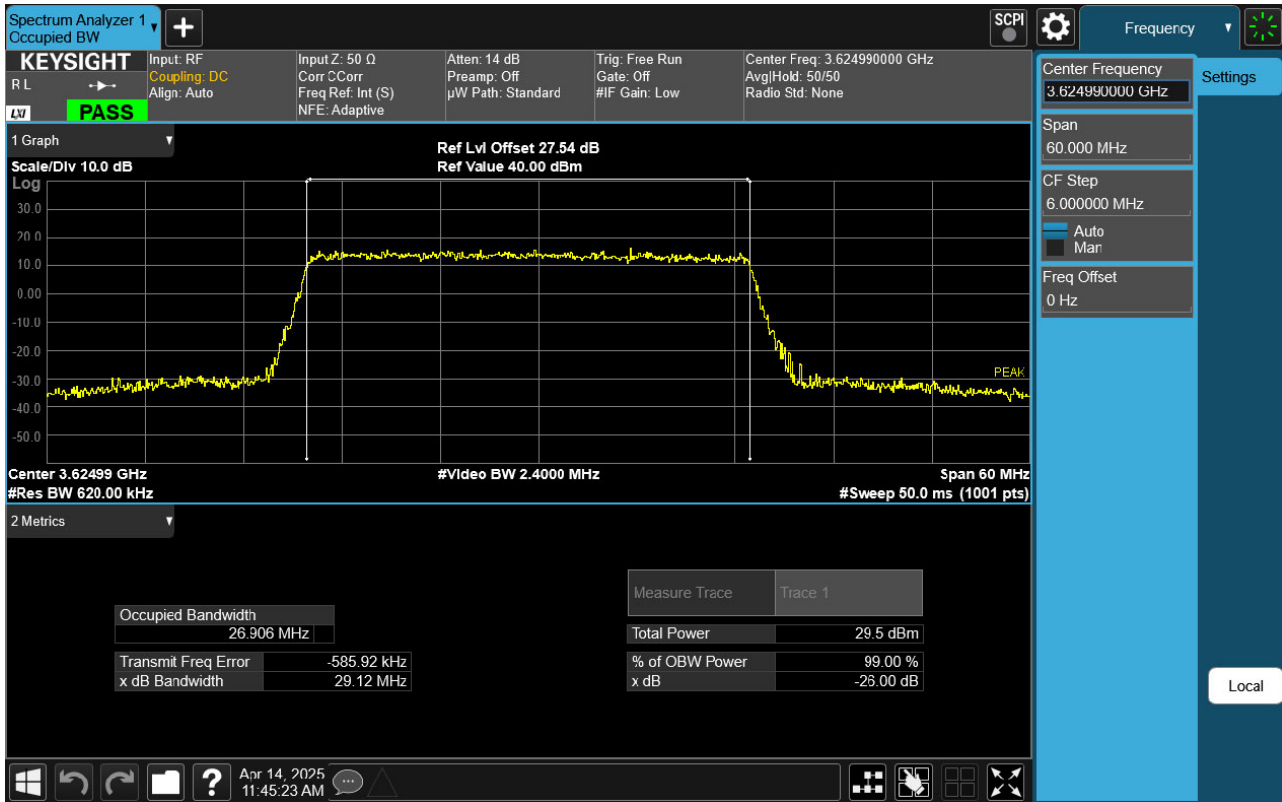
Sub6 n48. Occupied Bandwidth Plot (30 MHz Ch. 641666 QPSK RB 75)
