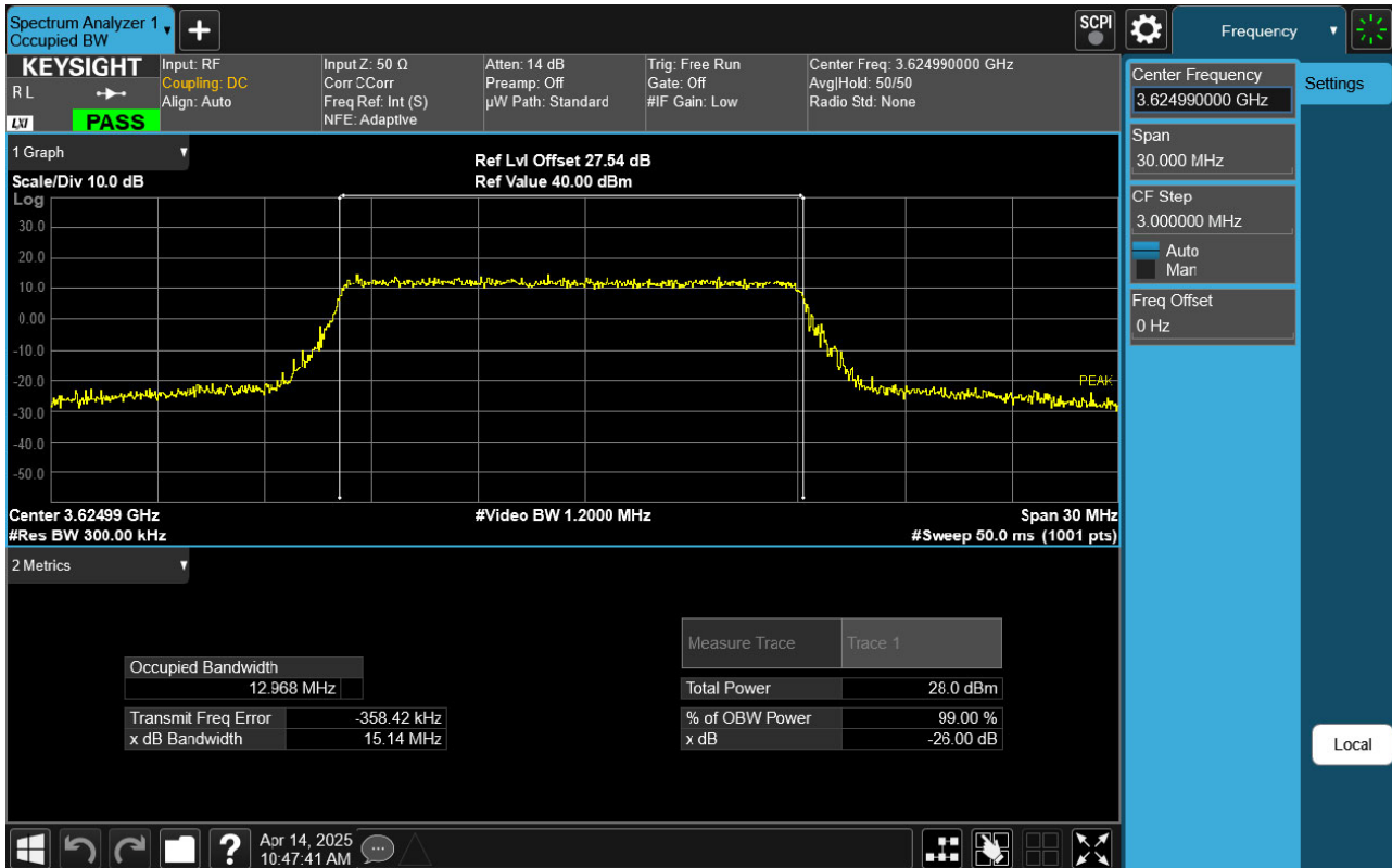
Sub6 n48. Occupied Bandwidth Plot (15 MHz Ch.641666 16-QAM RB 36)
