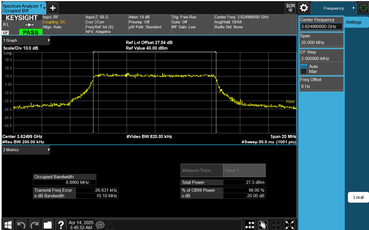
Sub6 n48. Occupied Bandwidth Plot (10 MHz Ch.641666 64-QAM RB 24)
