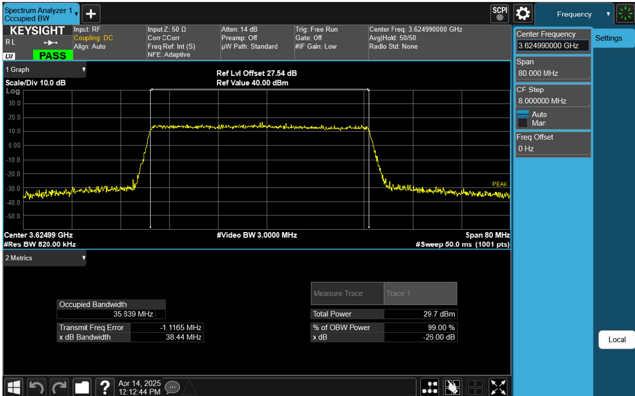
Sub6 n48. Occupied Bandwidth Plot (40 MHz Ch. 641666 QPSK RB 100)
