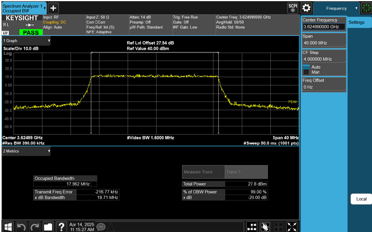
Sub6 n48. Occupied Bandwidth Plot (20 MHz Ch.641666 64-QAM RB 50)
