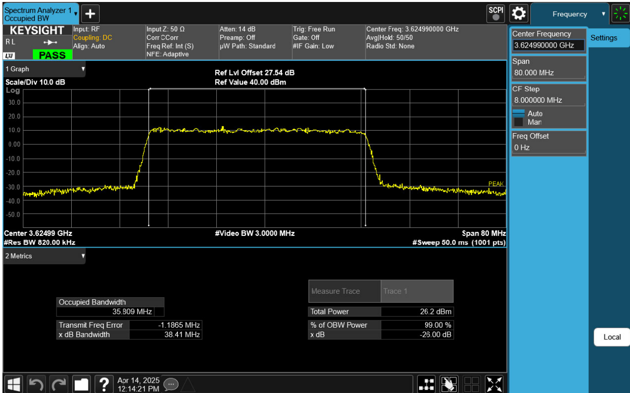
Sub6 n48. Occupied Bandwidth Plot (40 MHz Ch.641666 256-QAM RB 100)
