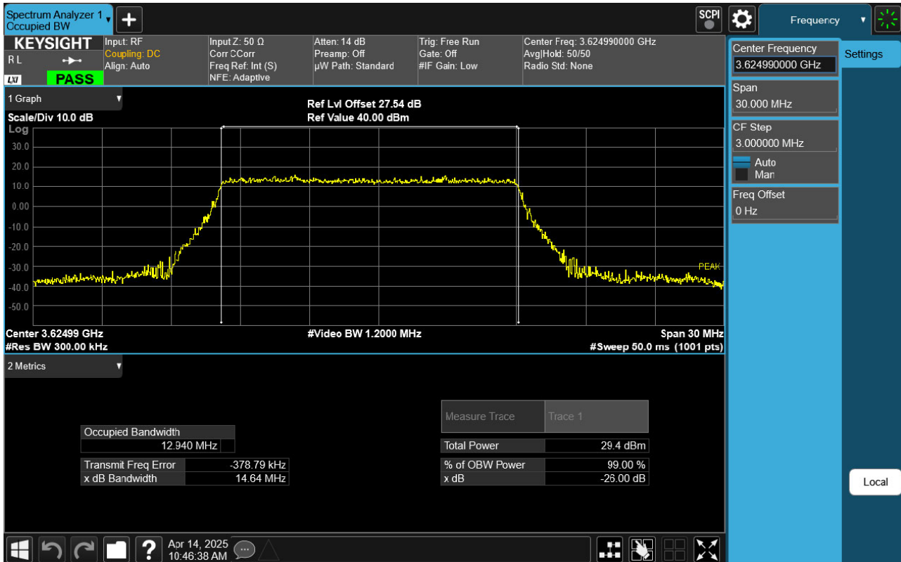
Sub6 n48. Occupied Bandwidth Plot (15 MHz Ch. 641666 BPSK RB 36)
