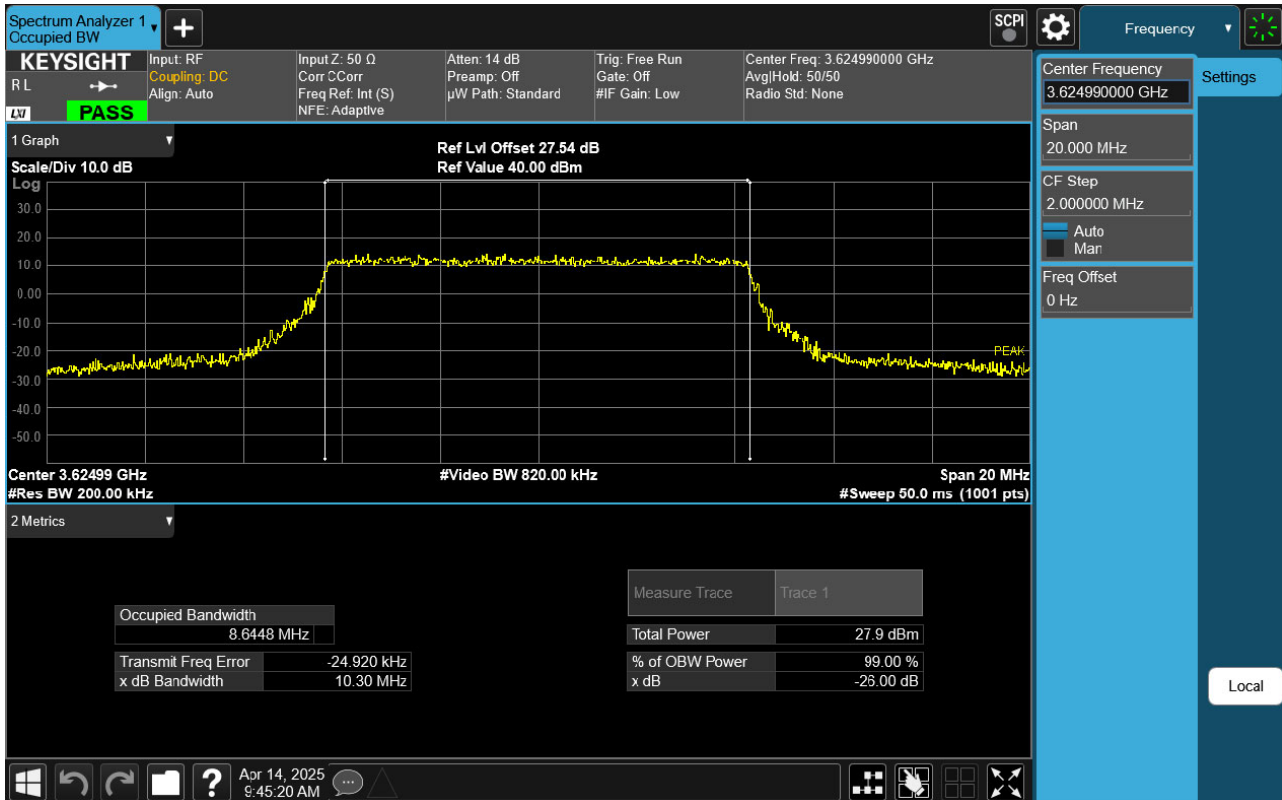
Sub6 n48. Occupied Bandwidth Plot (10 MHz Ch.641666 16-QAM RB 24)
