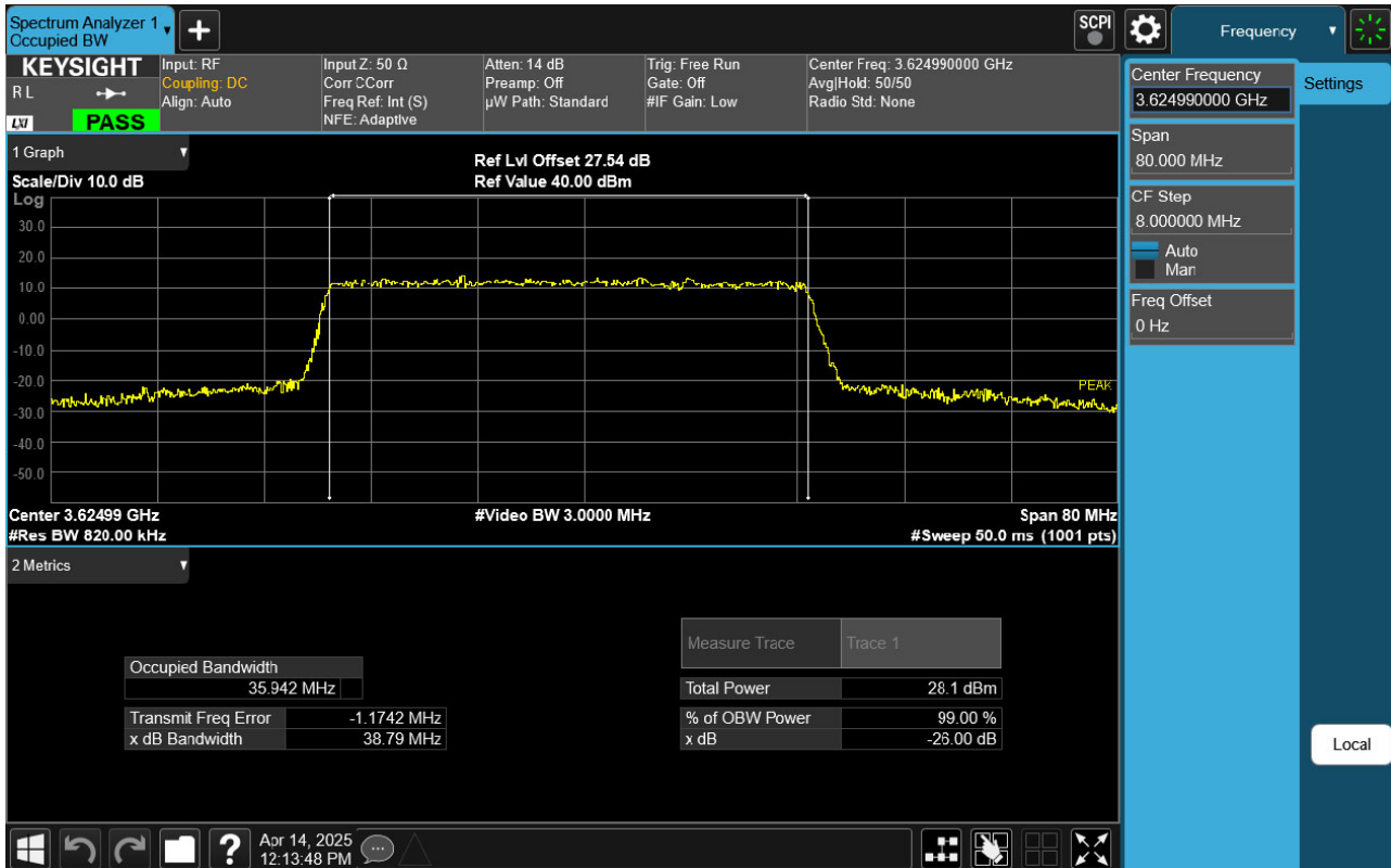
Sub6 n48. Occupied Bandwidth Plot (40 MHz Ch.641666 64-QAM RB 100)
