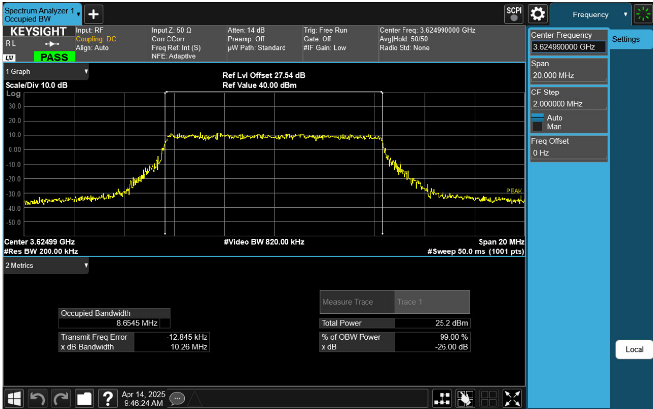
Sub6 n48. Occupied Bandwidth Plot (10 MHz Ch.641666 256-QAM RB 24)
