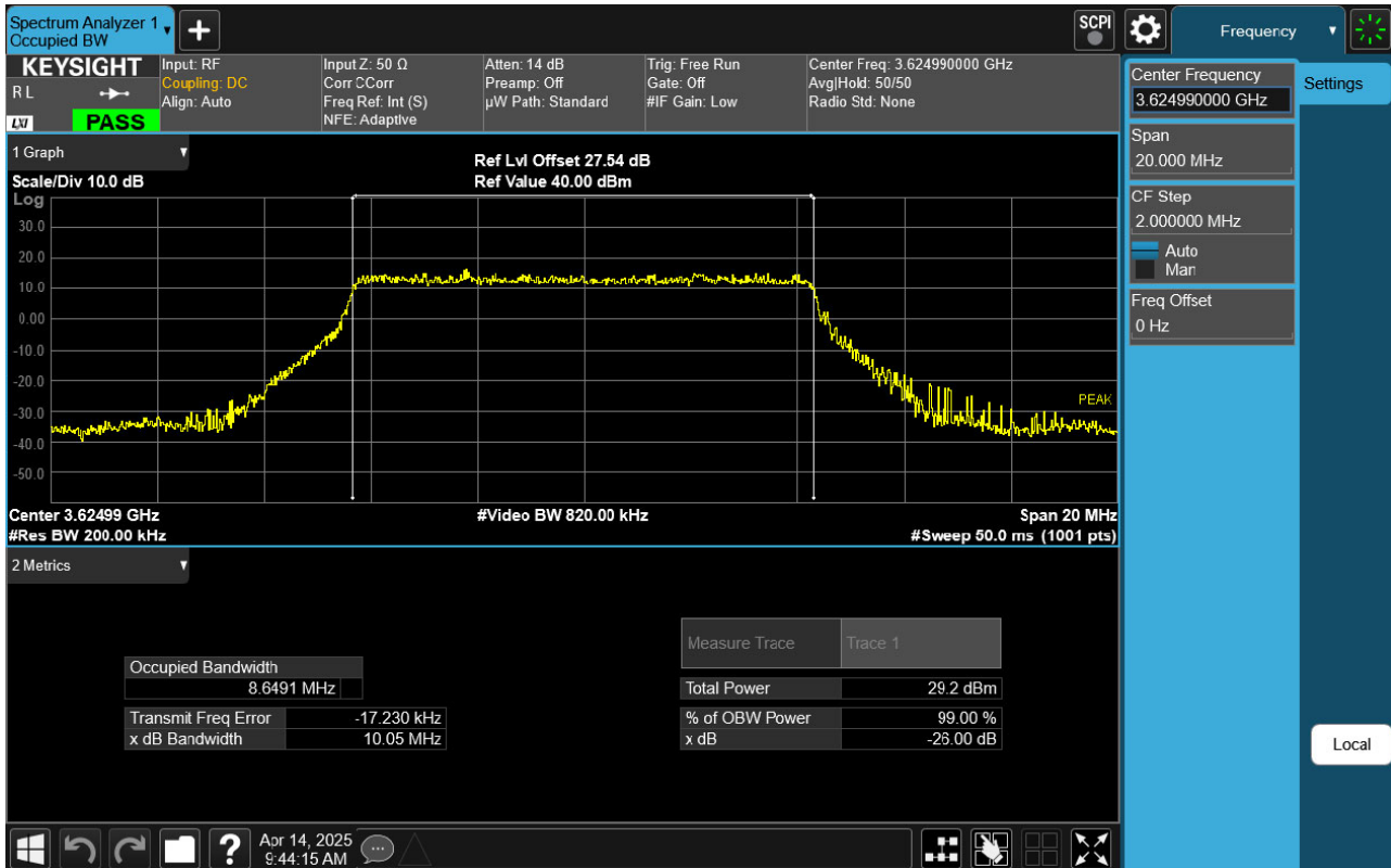
Sub6 n48. Occupied Bandwidth Plot (10 MHz Ch. 641666 BPSK RB 24)
