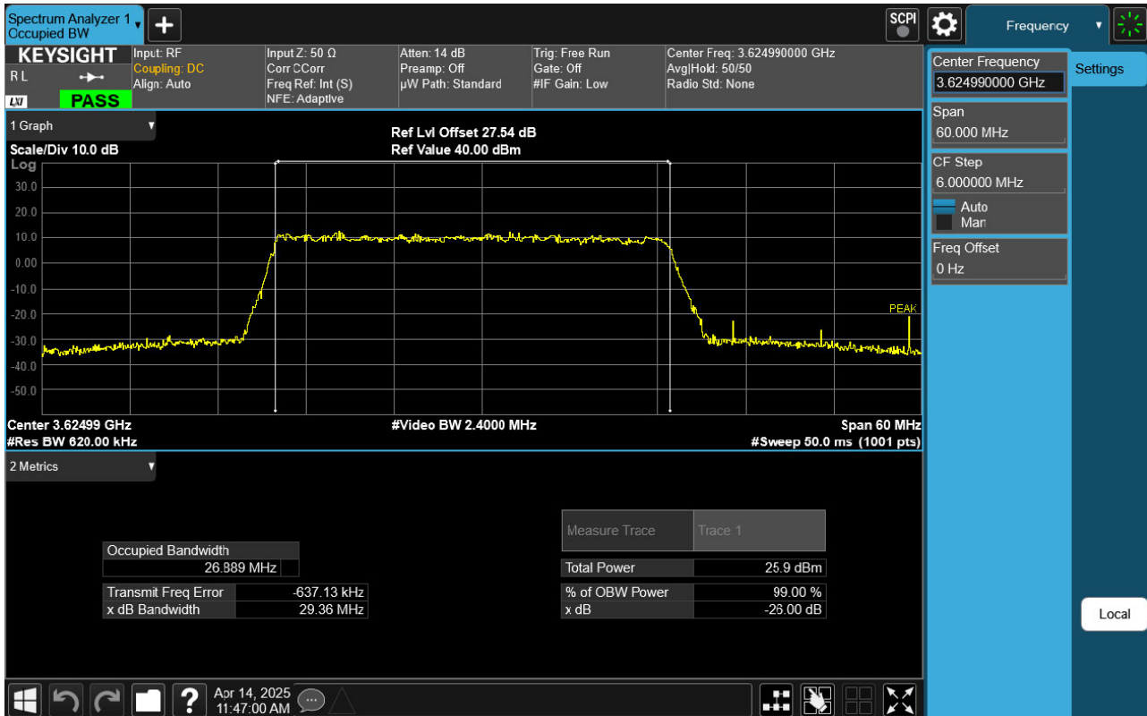
Sub6 n48. Occupied Bandwidth Plot (30 MHz Ch.641666 256-QAM RB 75)
