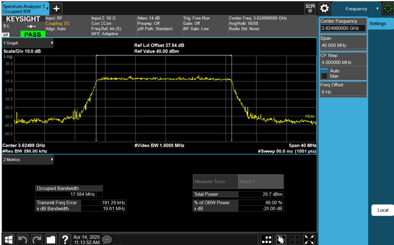
Sub6 n48. Occupied Bandwidth Plot (20 MHz Ch. 641666 BPSK RB 50)
