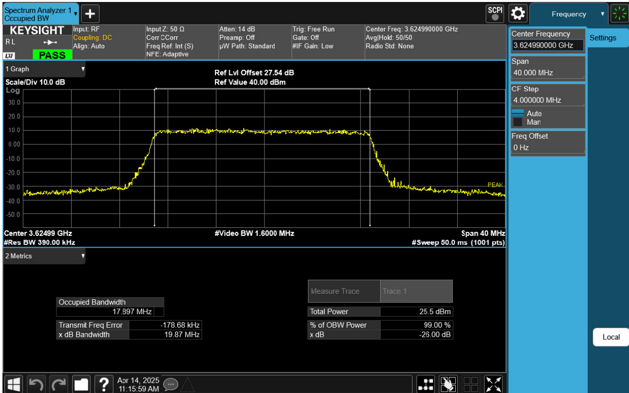
Sub6 n48. Occupied Bandwidth Plot (20 MHz Ch.641666 256-QAM RB 50)
