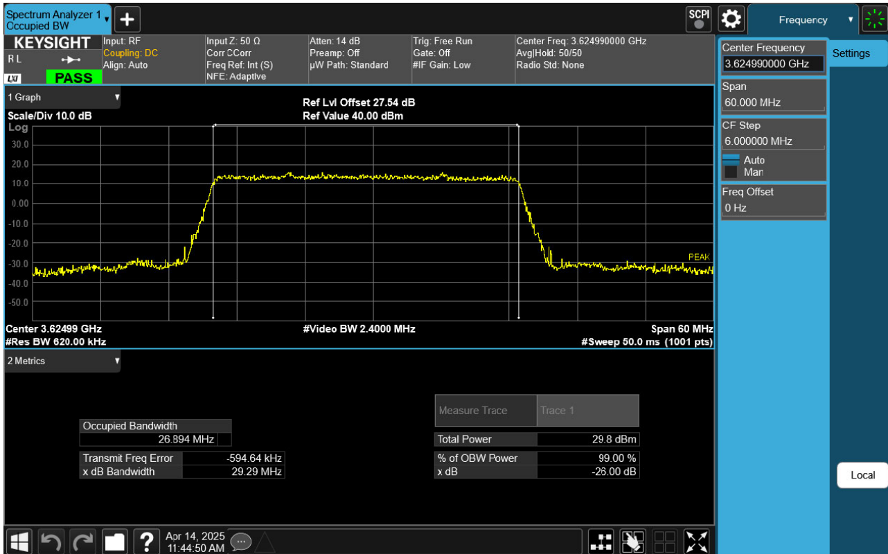
Sub6 n48. Occupied Bandwidth Plot (30 MHz Ch. 641666 BPSK RB 75)
