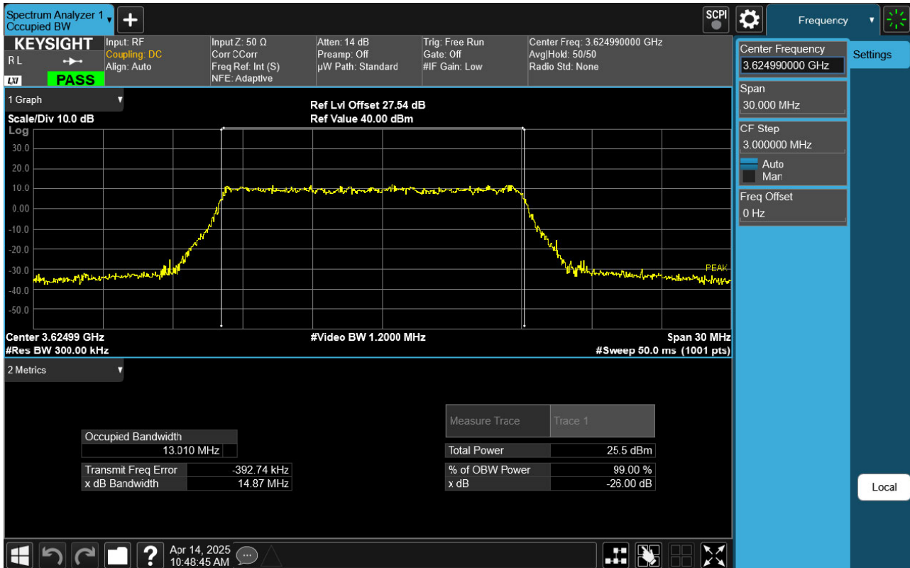
Sub6 n48. Occupied Bandwidth Plot (15 MHz Ch.641666 256-QAM RB 36)
