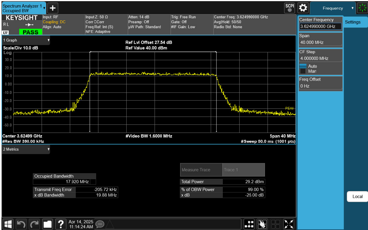
Sub6 n48. Occupied Bandwidth Plot (20 MHz Ch. 641666 QPSK RB 50)
