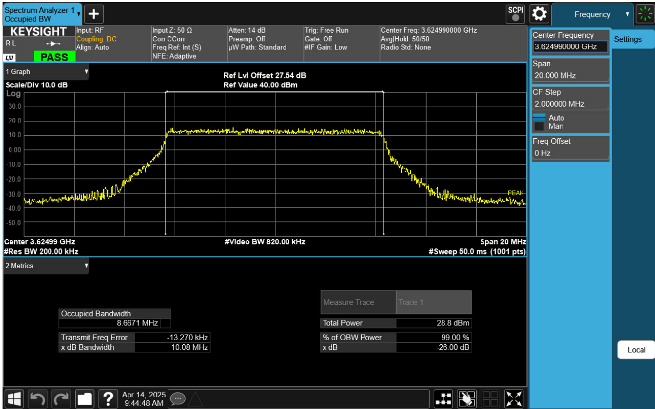
Sub6 n48. Occupied Bandwidth Plot (10 MHz Ch. 641666 QPSK RB 24)
