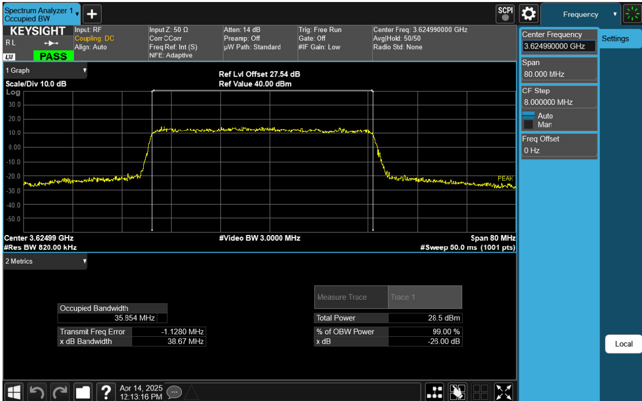
Sub6 n48. Occupied Bandwidth Plot (40 MHz Ch.641666 16-QAM RB 100)
