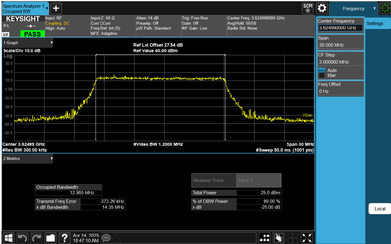
Sub6 n48. Occupied Bandwidth Plot (15 MHz Ch. 641666 QPSK RB 36)
