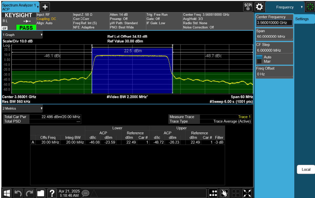
Sub6 n48. Adjacent Channel Leakage Ratio(ACLR) Plot (20 MHz Ch.637334 BPSK RB 50, Offset 0)
