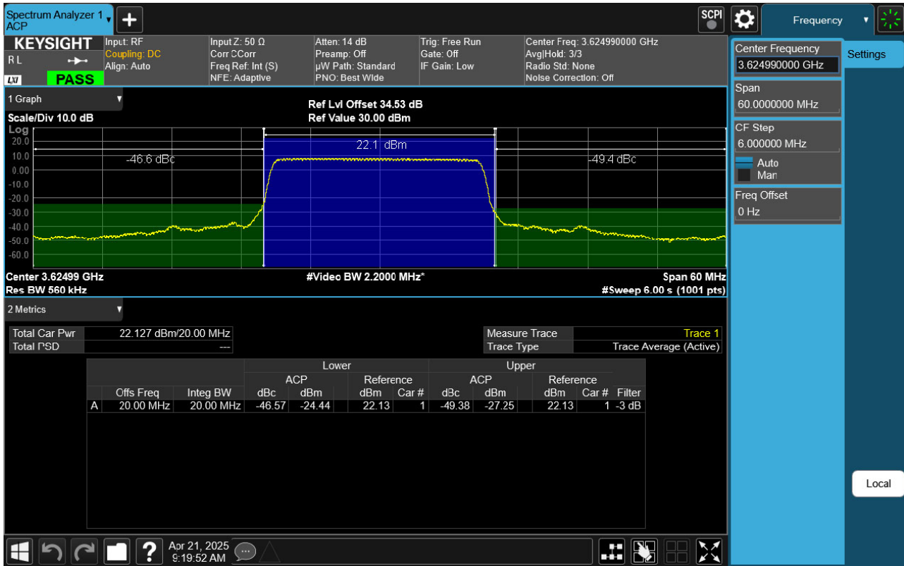
Sub6 n48. Adjacent Channel Leakage Ratio(ACLR) Plot (20 MHz Ch.641666 BPSK RB 50, Offset 0)
