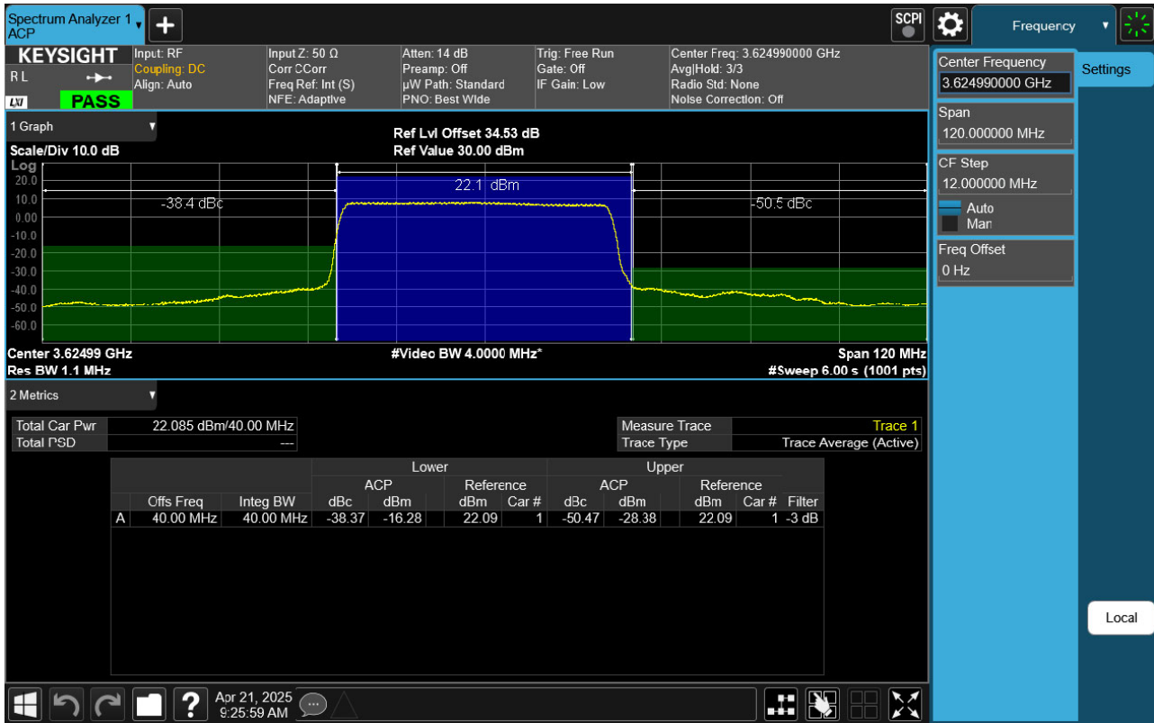
Sub6 n48. Adjacent Channel Leakage Ratio(ACLR) Plot (40 MHz Ch.641666 BPSK RB 100, Offset 0)
