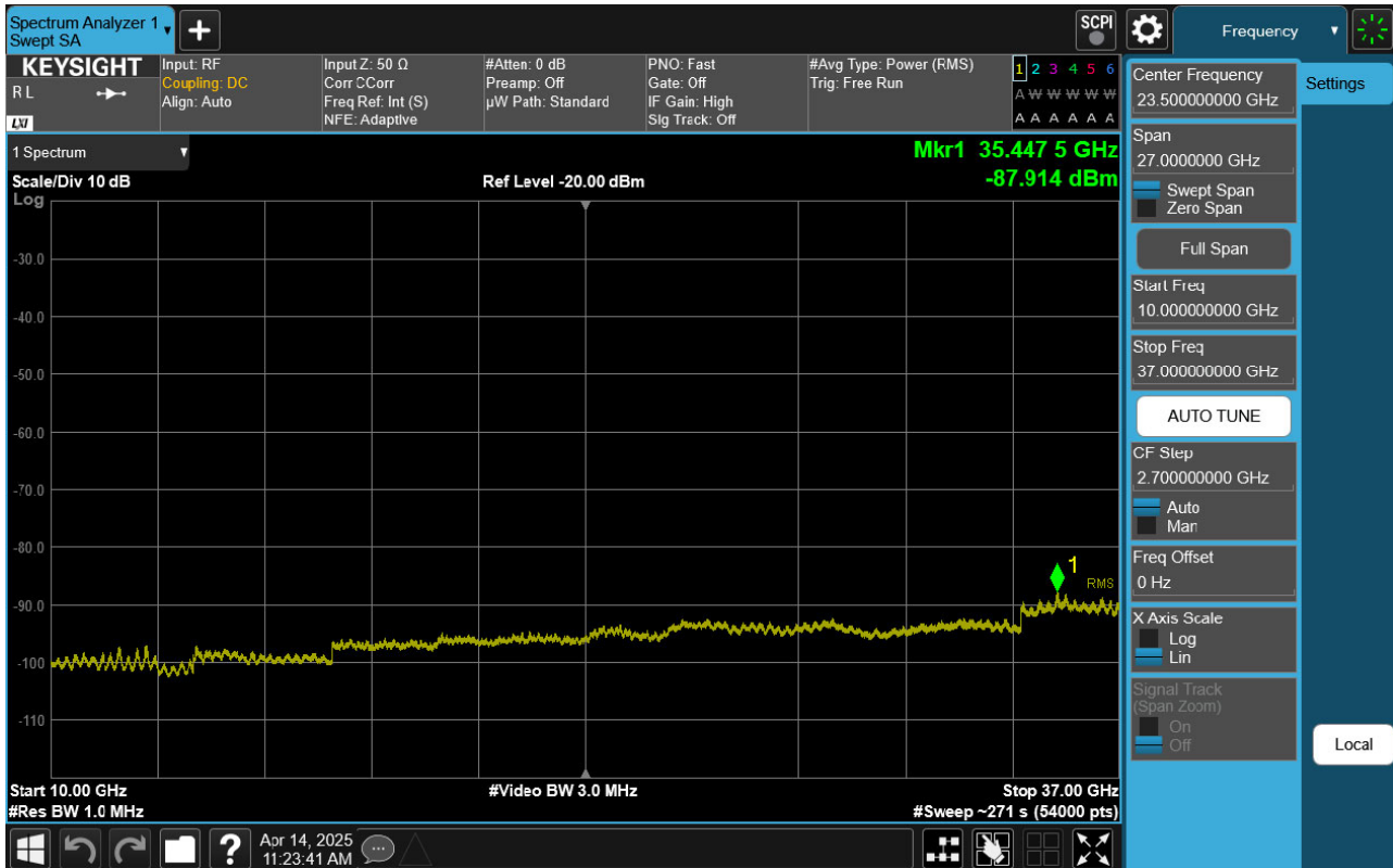
Sub6 n48. Conducted Spurious Plot 2 (20 MHz Ch. 641666 BPSK RB 1, Offset 1)
