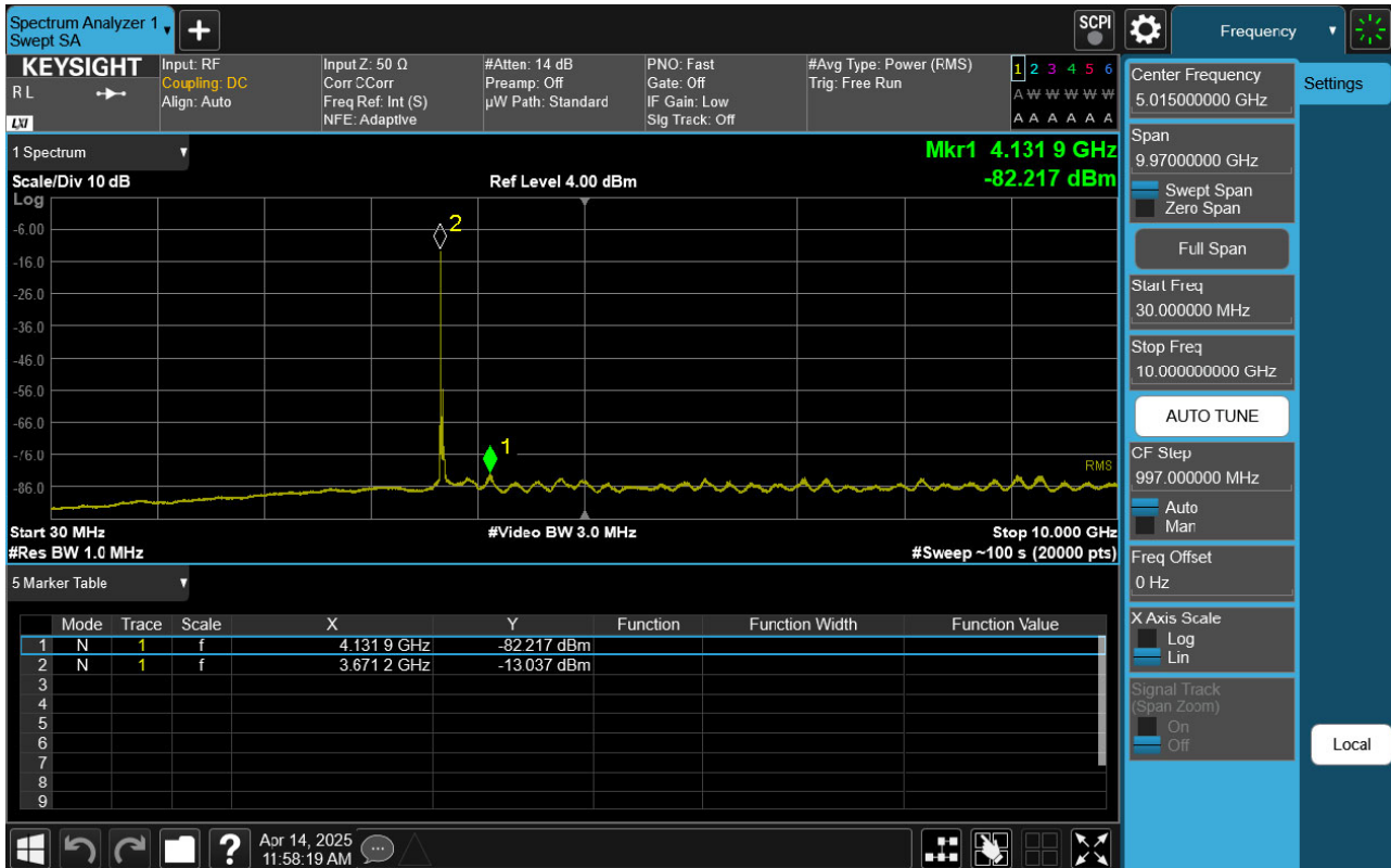
Sub6 n48. Conducted Spurious Plot 1 (30 MHz Ch. 645666 BPSK RB 1, Offset 1)
