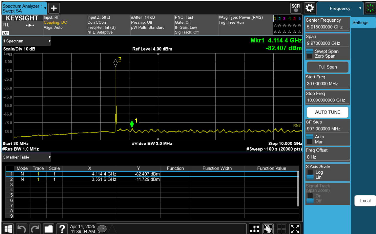
Sub6 n48. Conducted Spurious Plot 1 (30 MHz Ch. 637668 BPSK RB 1, Offset 1)
