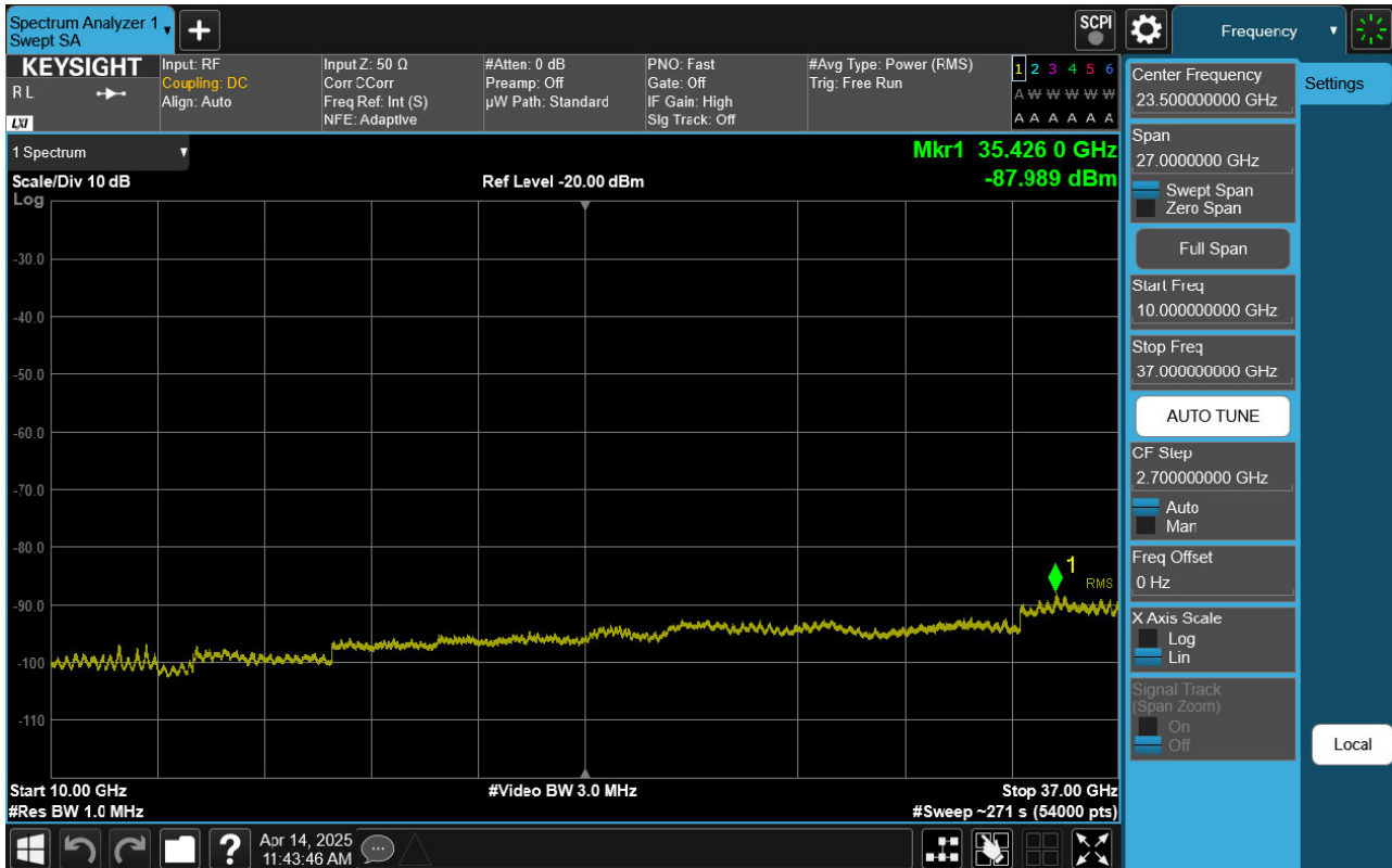
Sub6 n48. Conducted Spurious Plot 2 (30 MHz Ch. 637668 BPSK RB 1, Offset 1)
