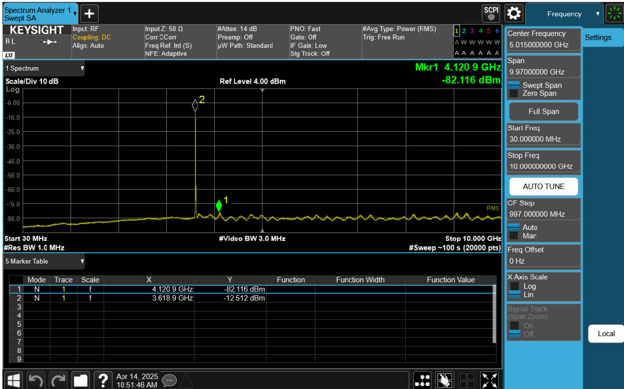
Sub6 n48. Conducted Spurious Plot 1 (15 MHz Ch. 641666 BPSK RB 1, Offset 1)
