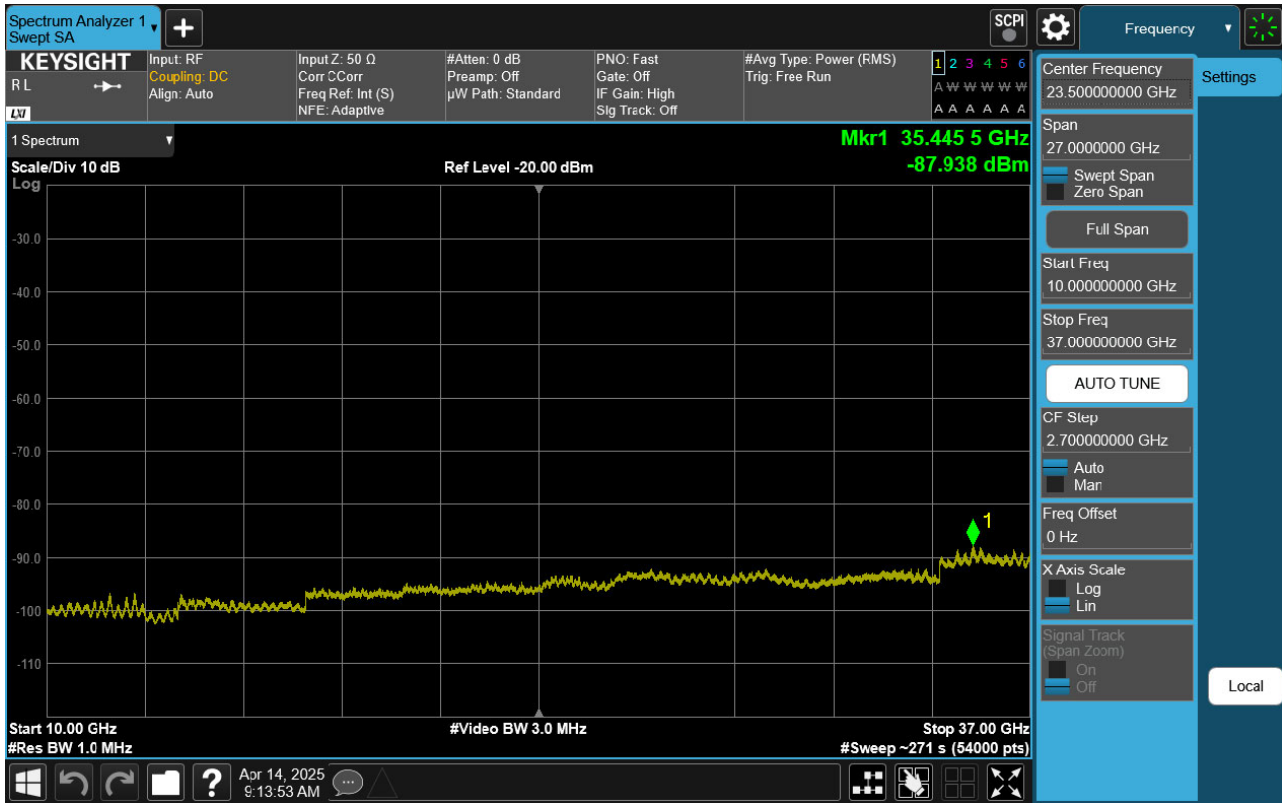
Sub6 n48. Conducted Spurious Plot 2 (10 MHz Ch. 637000 BPSK RB 1, Offset 1)
