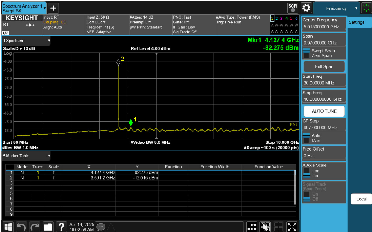
Sub6 n48. Conducted Spurious Plot 1 (10 MHz Ch. 646332 BPSK RB 1, Offset 1)
