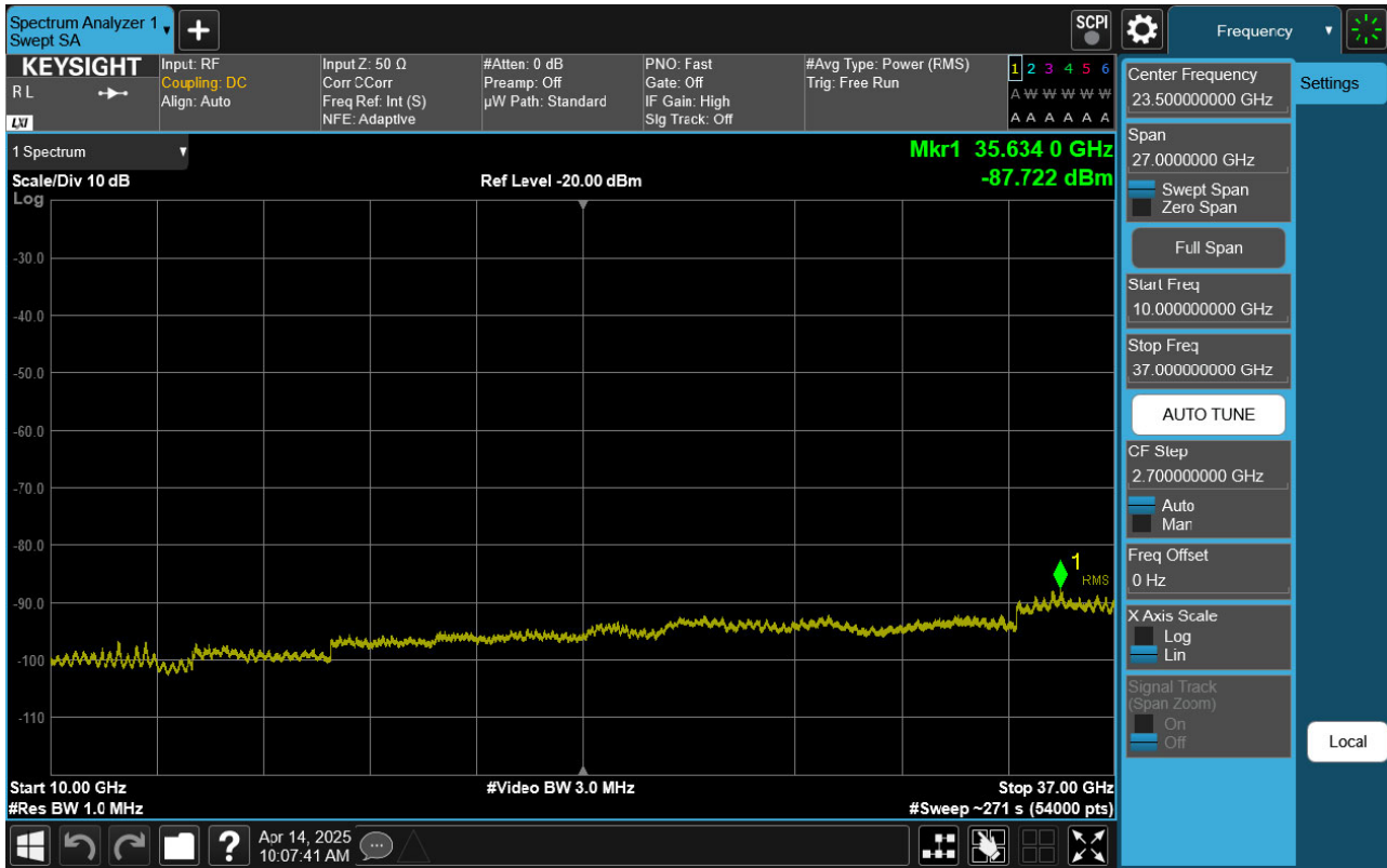
Sub6 n48. Conducted Spurious Plot 2 (10 MHz Ch. 646332 BPSK RB 1, Offset 1)
