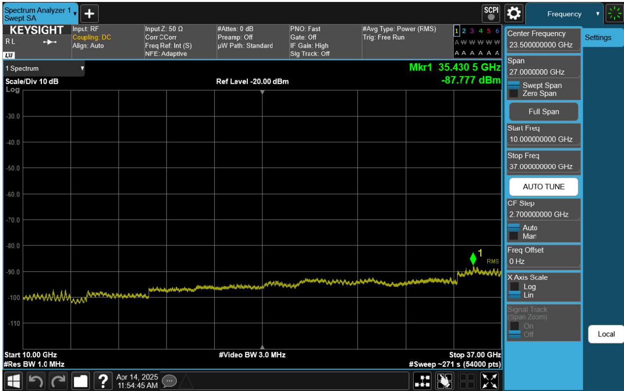
Sub6 n48. Conducted Spurious Plot 2 (30 MHz Ch. 641666 BPSK RB 1, Offset 1)
