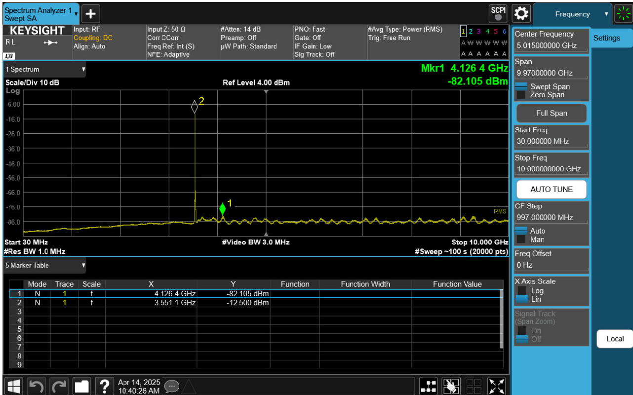
Sub6 n48. Conducted Spurious Plot 1 (15 MHz Ch. 637168 BPSK RB 1, Offset 1)
