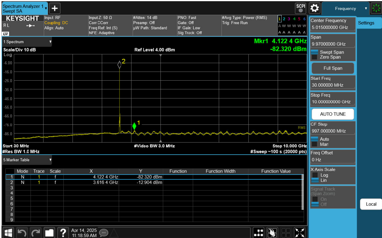
Sub6 n48. Conducted Spurious Plot 1 (20 MHz Ch. 641666 BPSK RB 1, Offset 1)
