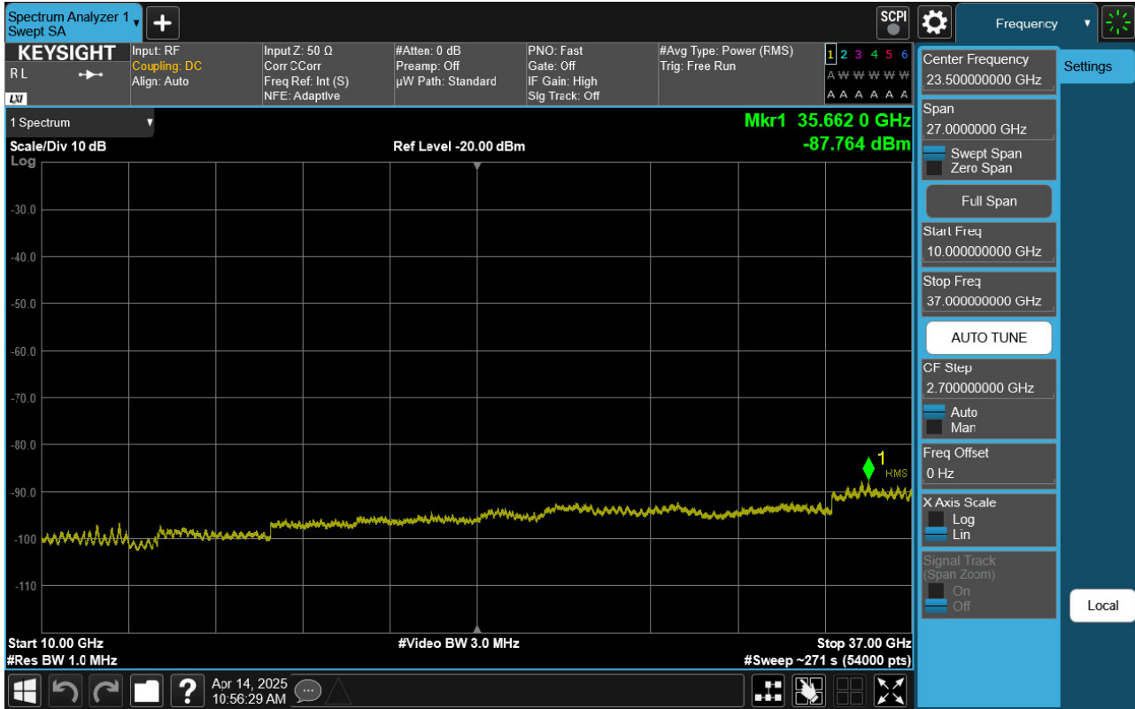
Sub6 n48. Conducted Spurious Plot 2 (15 MHz Ch. 641666 BPSK RB 1, Offset 1)
