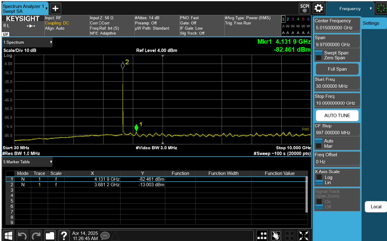
Sub6 n48. Conducted Spurious Plot 1 (20 MHz Ch. 646000 BPSK RB 1, Offset 1)
