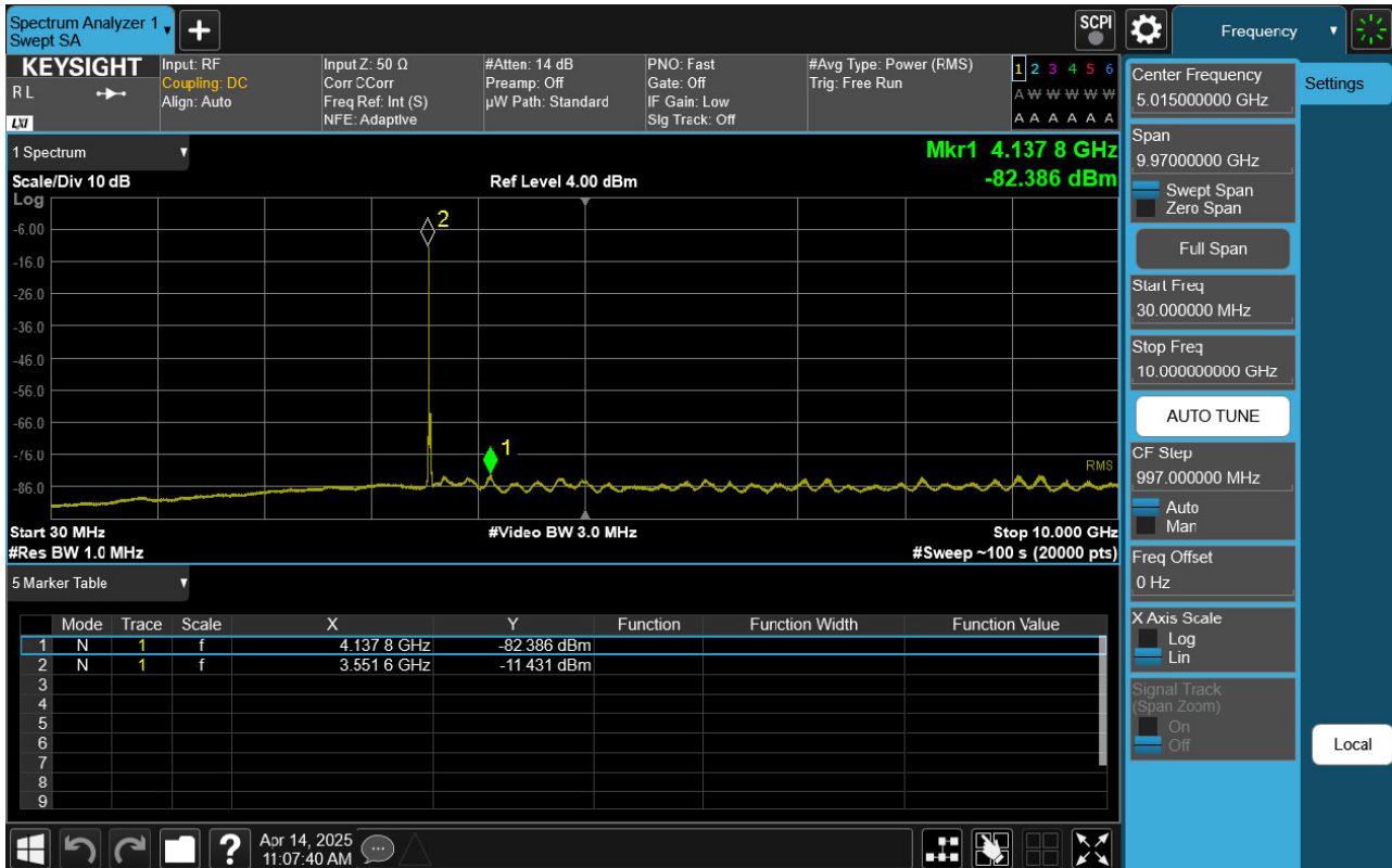
Sub6 n48. Conducted Spurious Plot 1 (20 MHz Ch. 637334 BPSK RB 1, Offset 1)
