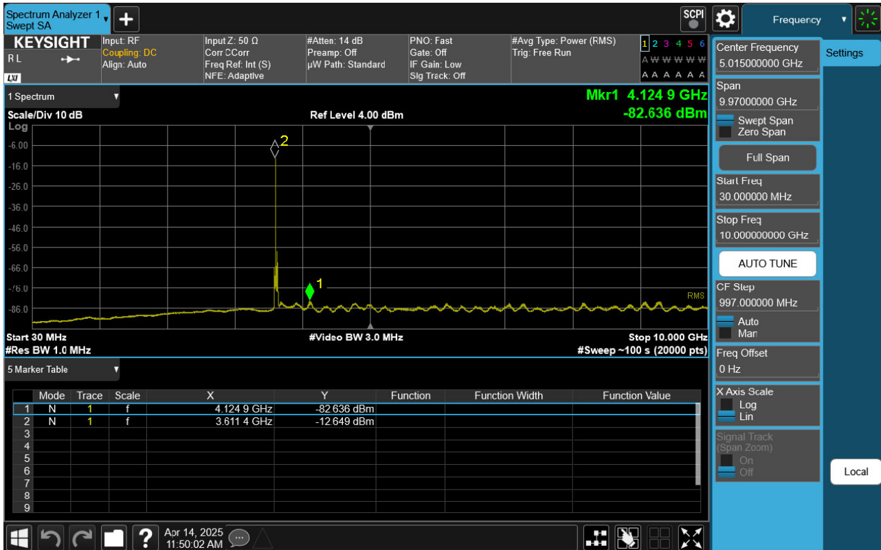
Sub6 n48. Conducted Spurious Plot 1 (30 MHz Ch. 641666 BPSK RB 1, Offset 1)
