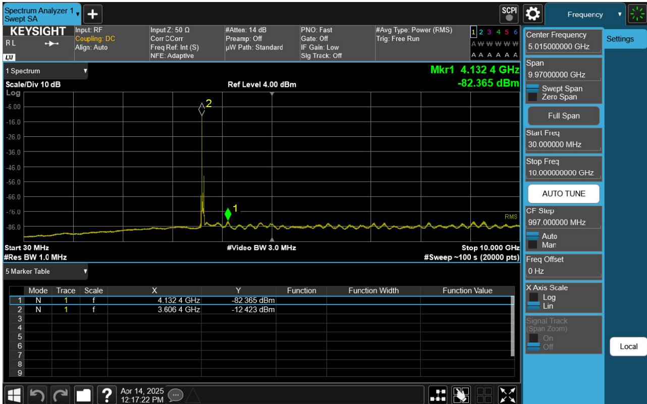
Sub6 n48. Conducted Spurious Plot 1 (40 MHz Ch. 641666 BPSK RB 1, Offset 1)
