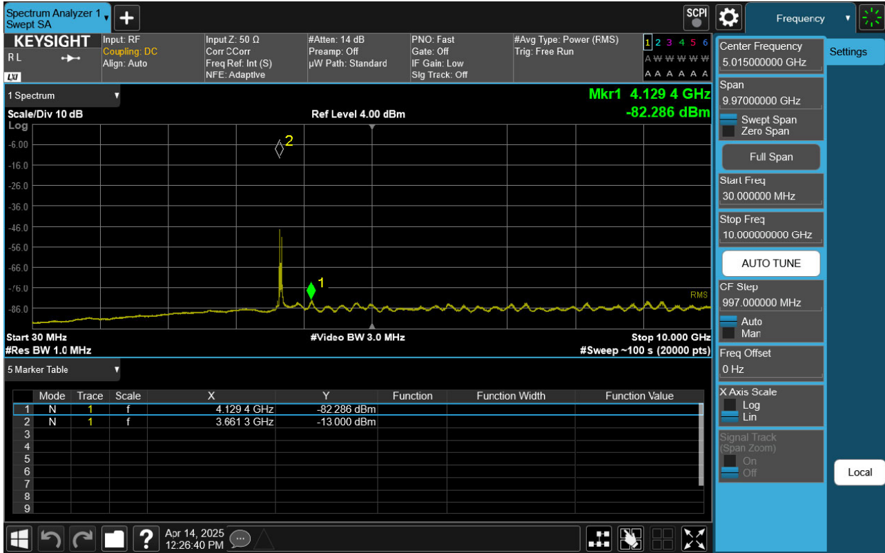
Sub6 n48. Conducted Spurious Plot 1 (40 MHz Ch. 645332 BPSK RB 1, Offset 1)
