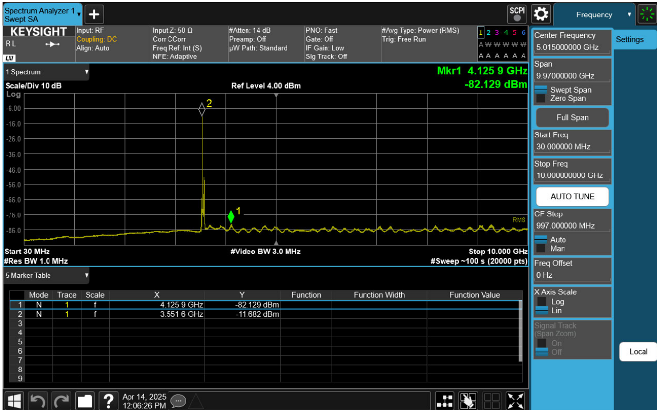
Sub6 n48. Conducted Spurious Plot 1 (40 MHz Ch. 638000 BPSK RB 1, Offset 1)
