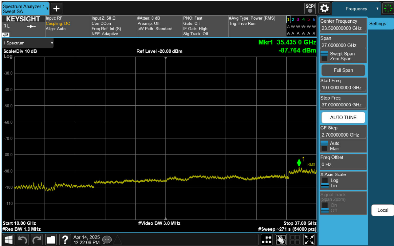
Sub6 n48. Conducted Spurious Plot 2 (40 MHz Ch. 641666 BPSK RB 1, Offset 1)
