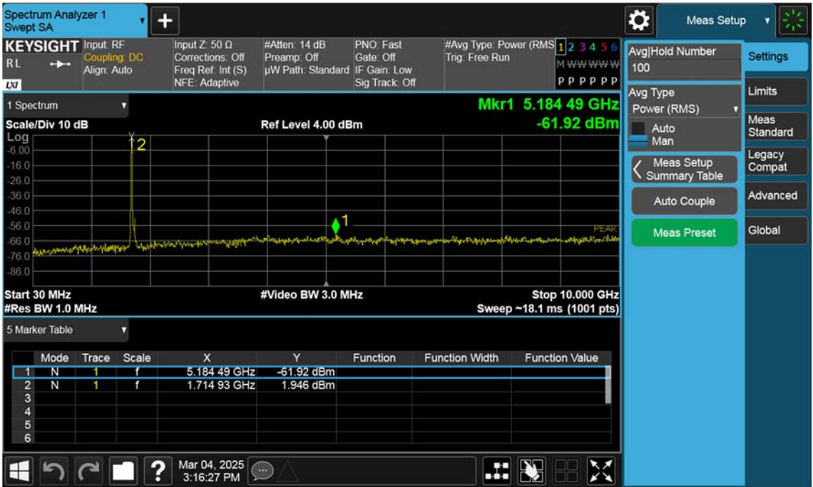
NR66_30 M_Conducted Spurious(30 M-10 G)_Low_BPSK_1RB
