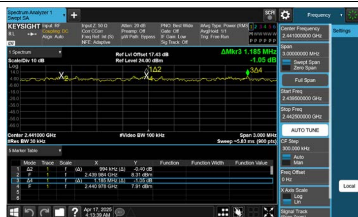
Dual ANT. 2\pi/4 DQPSK : Channel Separation
