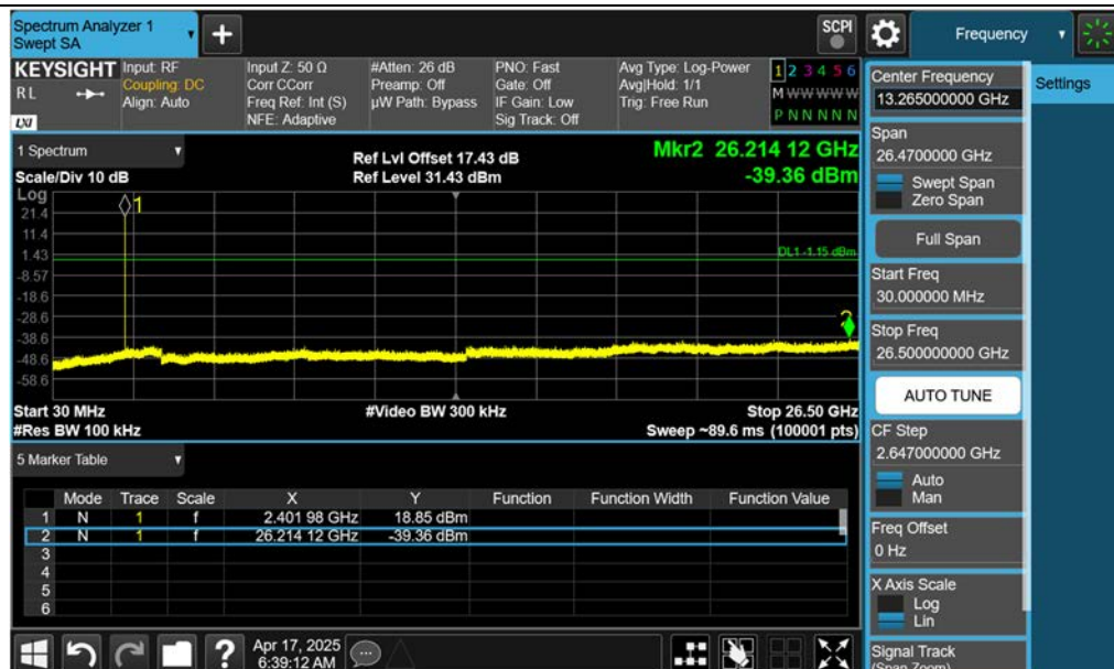
Spurious Emission (30 MHz - 26.50 GHz)Ant.2, GFSK Ch. 0
