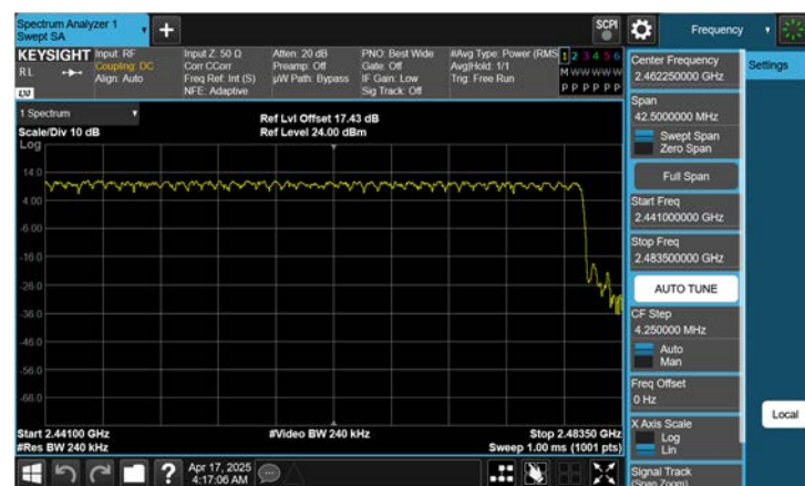
Dual ANT.2 \pi/4 DQPSK (2.441 GHz - 2.483.5 GHz)
