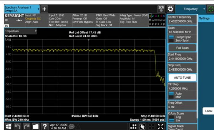
Dual ANT.2 \pi/4 DQPSK (2.441 GHz - 2.483.5 GHz)
