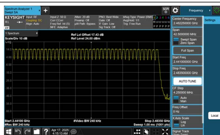
Dual ANT.2 8DPSK (2.441 GHz - 2.483.5 GHz)
