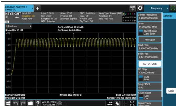
Dual ANT.2 8DPSK (2.4 GHz - 2.441 GHz)
