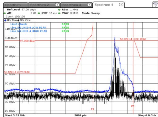
Peak result (802.11be(EHT80) Ch.171, 26T RU 0)
