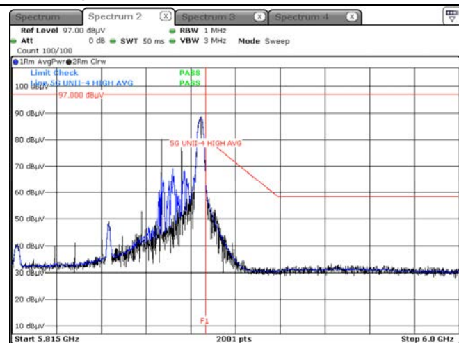
Average result (802.11be(EHT80) Ch.171, 106T RU 60)
