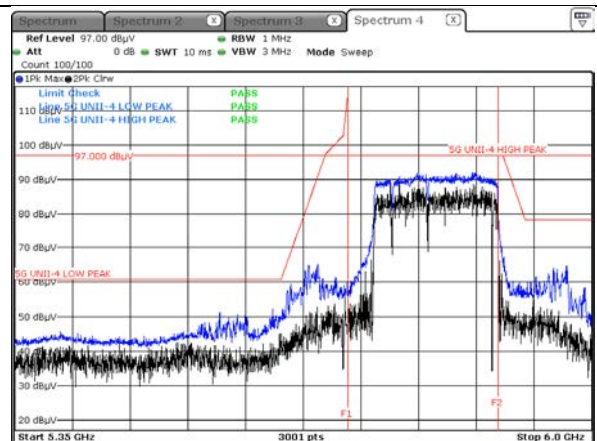
Peak result (802.11be(EHT160) Ch.163, 996T+484T+242T RU 96)
