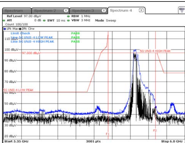
Peak result (802.11be(EHT80) Ch.171, 106T+26T RU 82)
