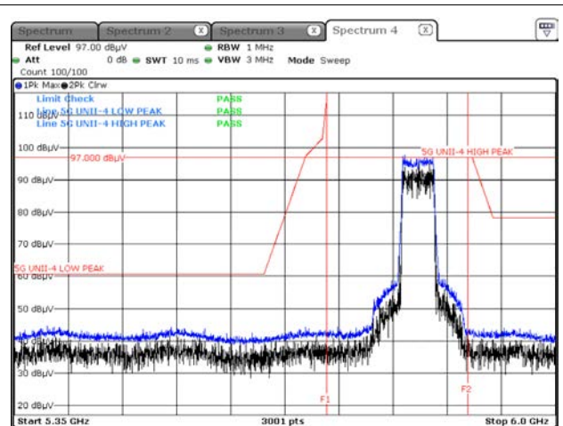
Peak result (802.11be(EHT40) Ch.167, SU)
