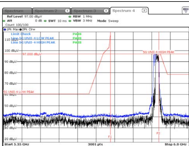
Peak result (802.11be(EHT20) Ch.177, 106T+26T RU 83)
