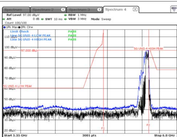
Peak result (802.11be(EHT40) Ch.175, 106T+26T RU 85)
