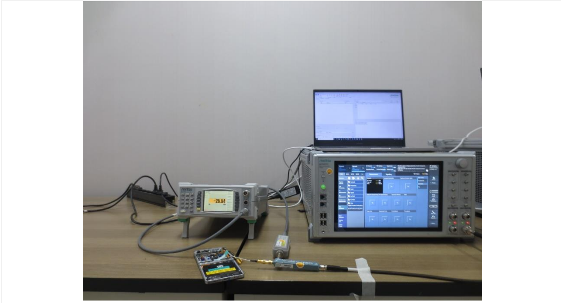
Test setup photo-1 (TC 1)
