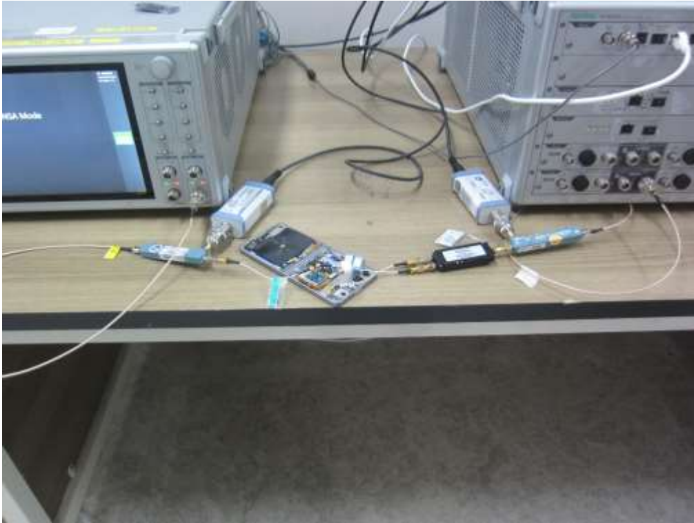
Test setup photo-7 TC 14
