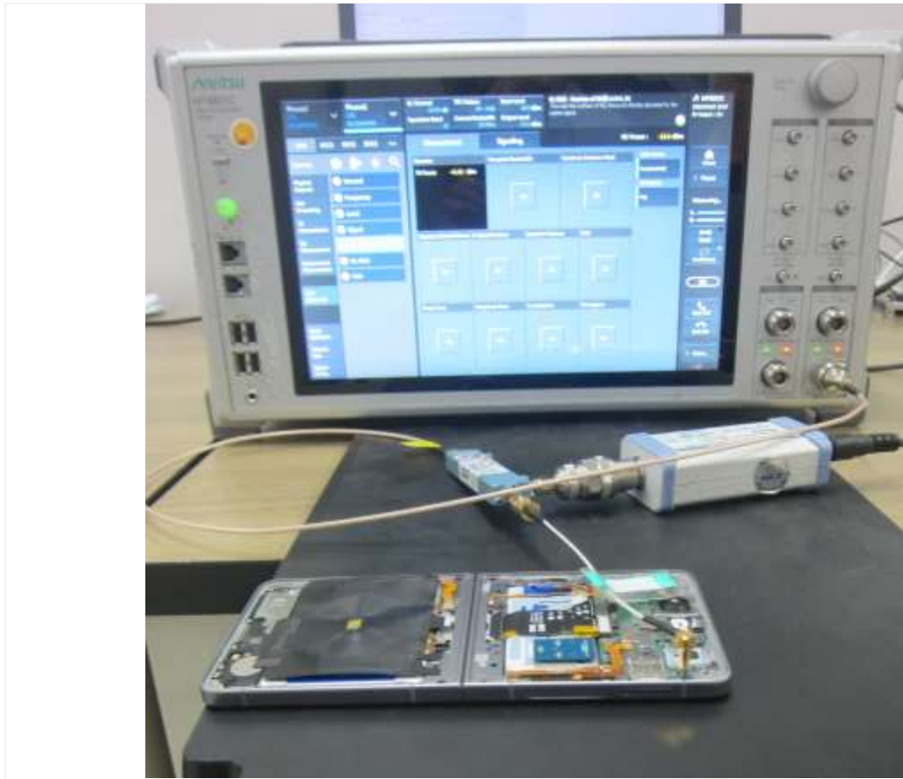
Test setup photo-8 TC 15
