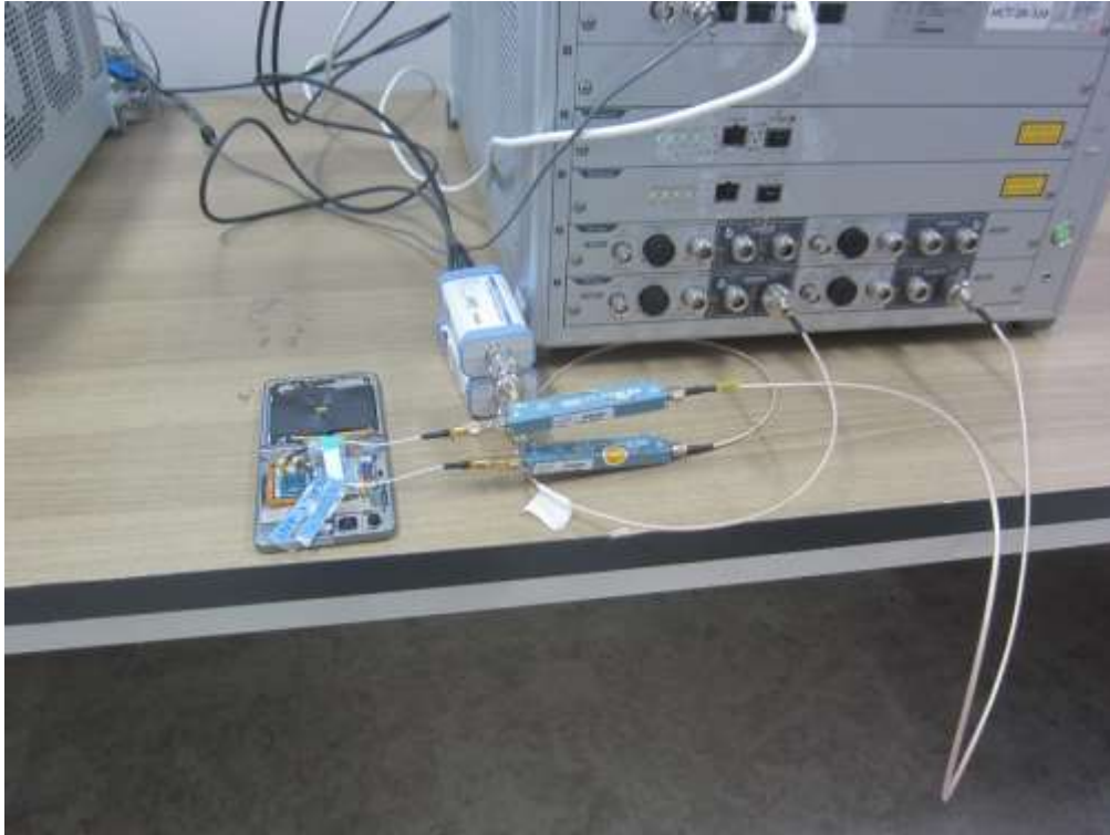
Test setup photo-9 TC 16
