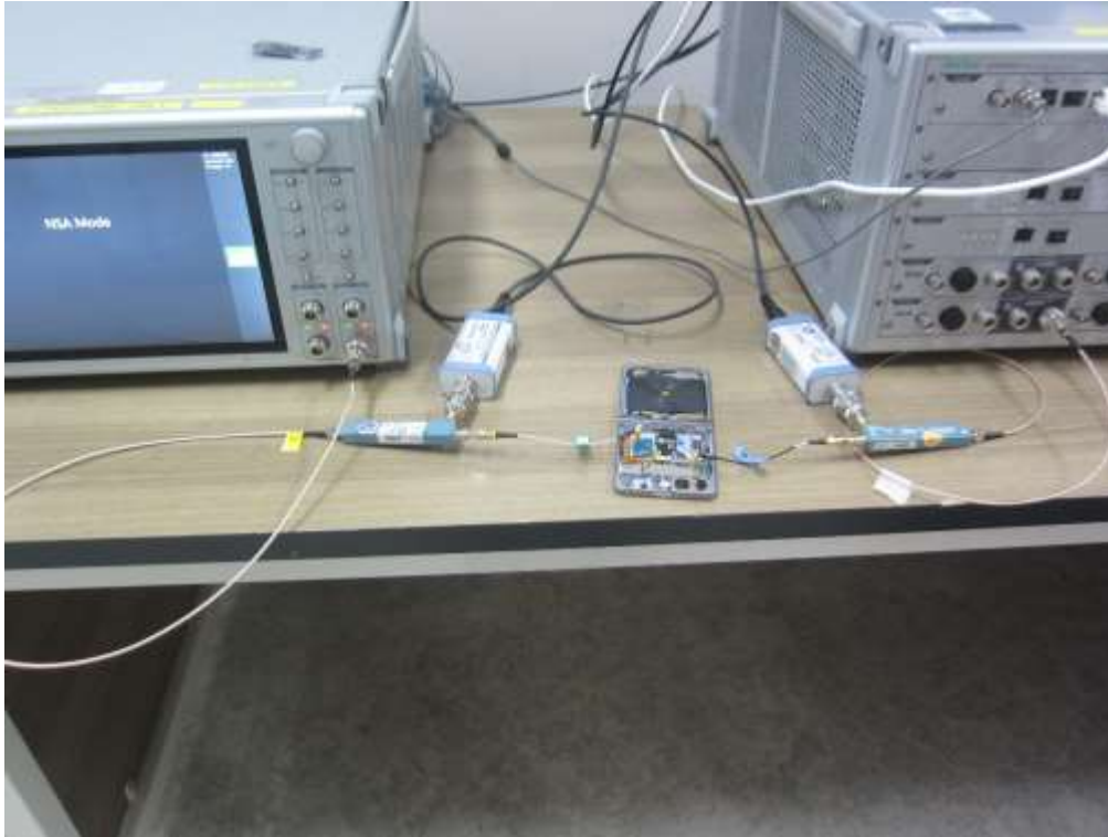
Test setup photo-11 TC 18
