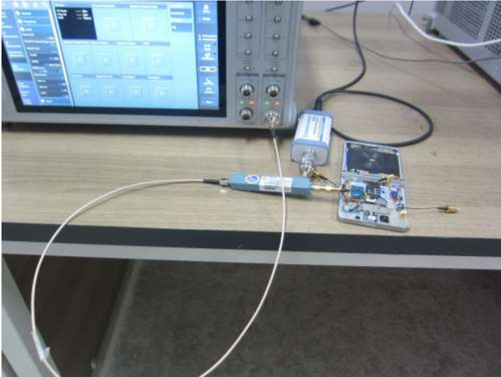
Test setup photo-10 TC 17
