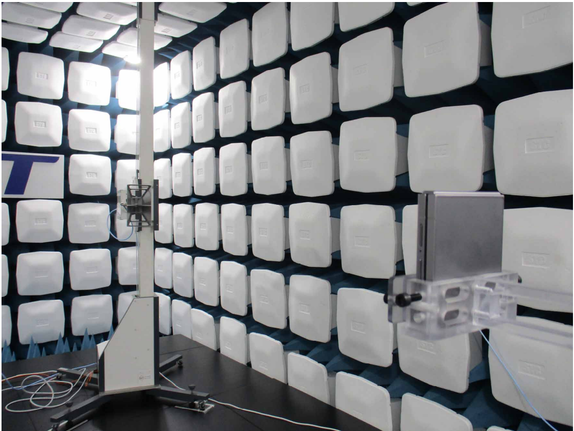
(above 1 GHz, Antenna Mast: Horizontal)
