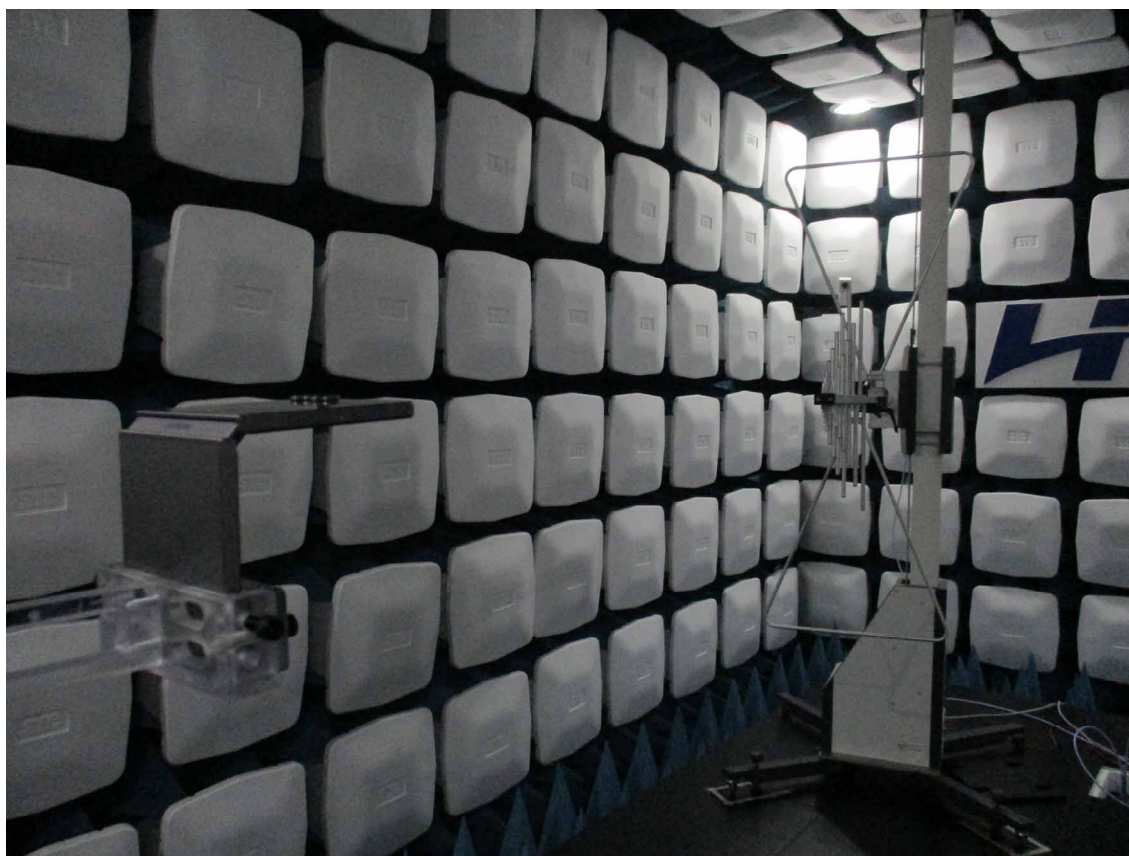
(below 1 GHz, Antenna Mast: Vertical)
