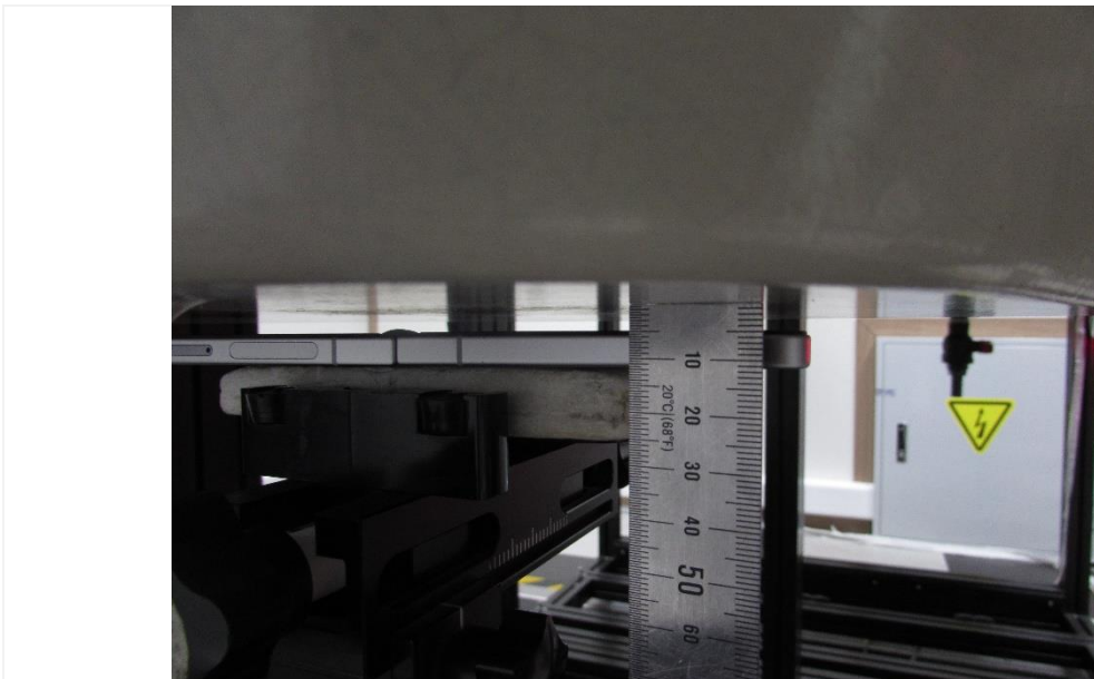
Distance of 5 mm from the EUT
