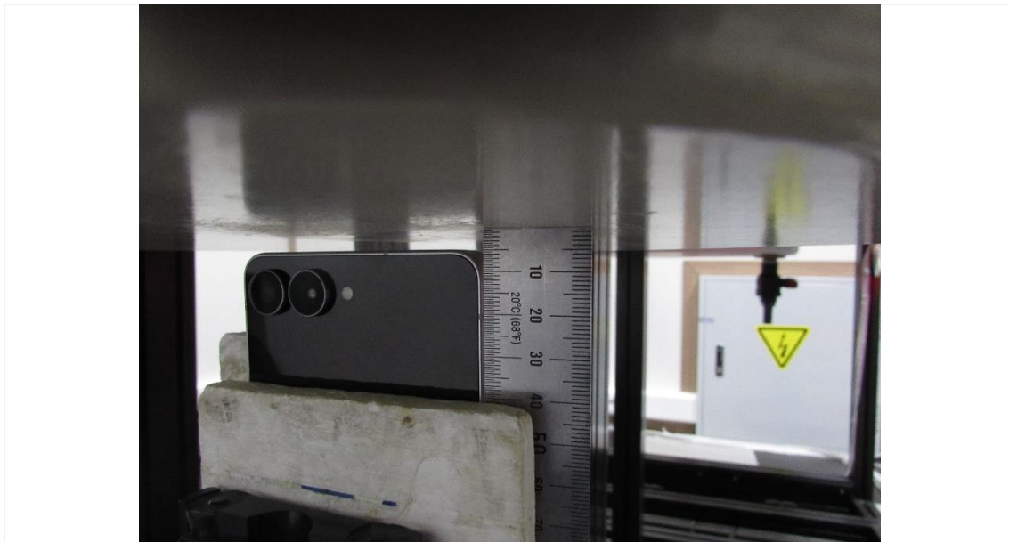
Distance of 5 mm from the EUT
