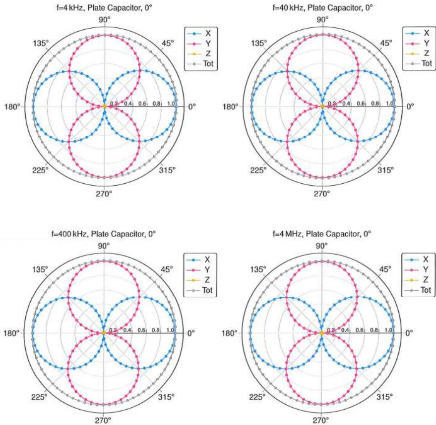
E-Field Receiving Pattern ( \phi ), \theta = 0^\circ
