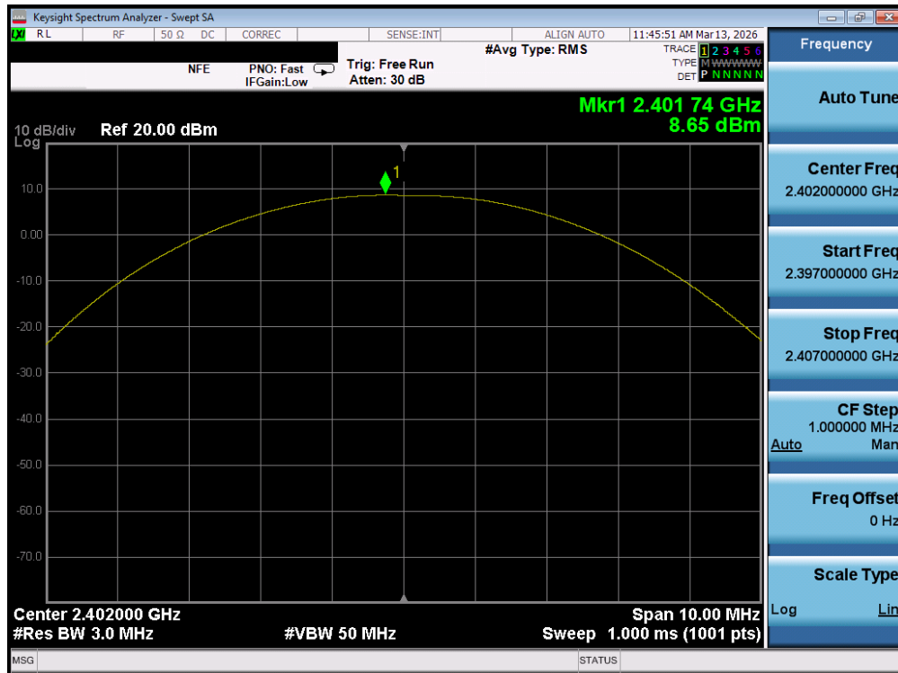
Plot 7-49. Peak Power Plot (Bluetooth (LE), 125kbps – Ch. 37) – Ant 2
