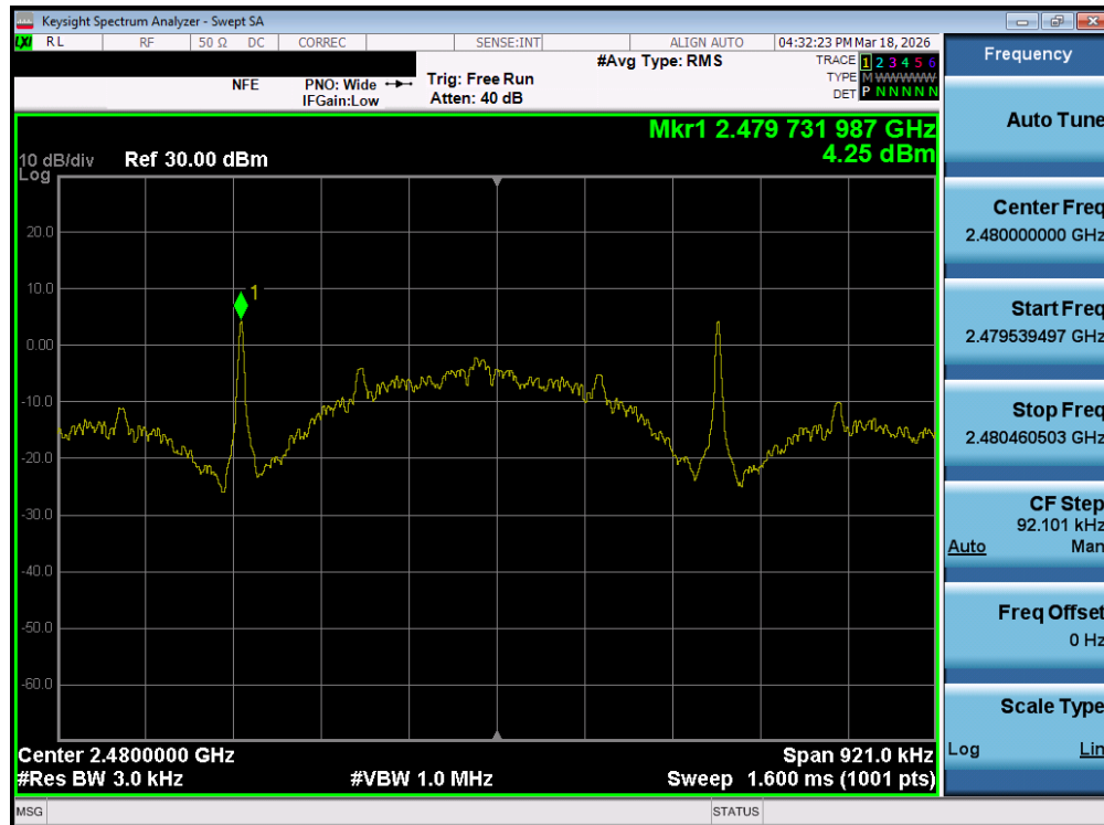
Plot 7-75. Power Spectral Density Plot (Bluetooth (LE), 125kbps – Ch. 39) – Ant 1
