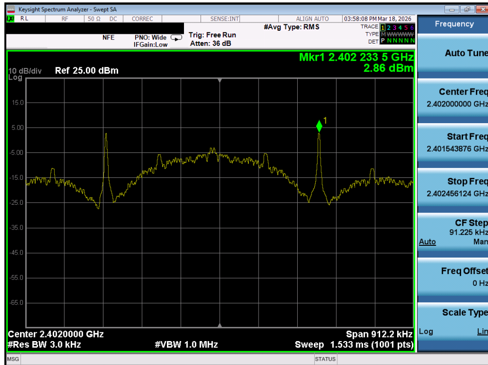
Plot 7-73. Power Spectral Density Plot (Bluetooth (LE), 125kbps – Ch. 37) – Ant 1
