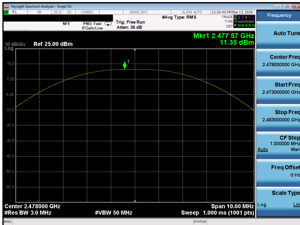
Plot 7-72. Peak Power Plot (Bluetooth (LE), 2Mbps – Ch. 36) – Dual Ant 2
