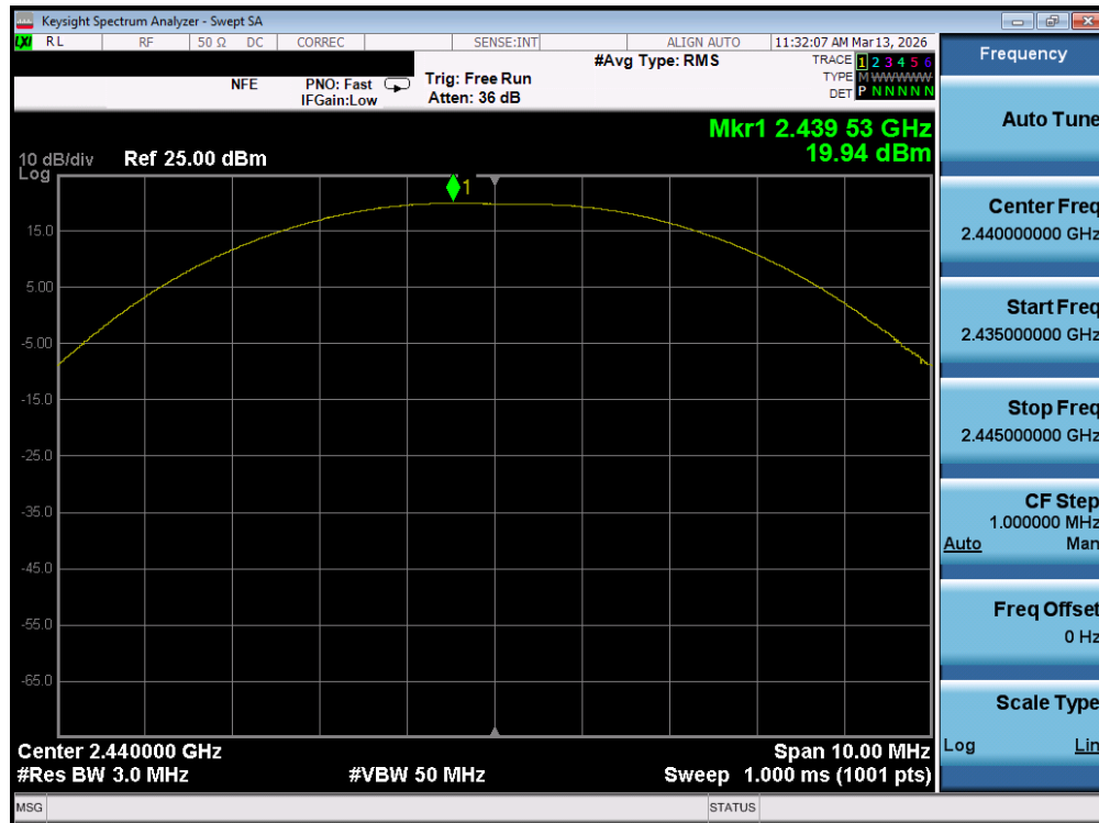
Plot 7-47. Peak Power Plot (Bluetooth (LE), 2Mbps – Ch. 17) – Ant 1
