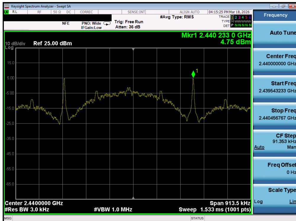
Plot 7-74. Power Spectral Density Plot (Bluetooth (LE), 125kbps – Ch. 17) – Ant 1
