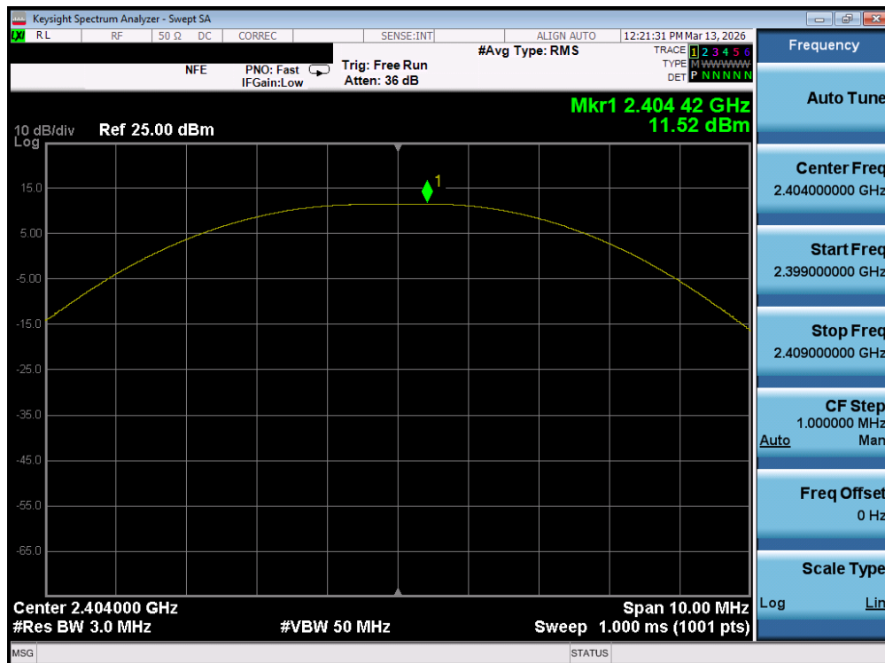
Plot 7-70. Peak Power Plot (Bluetooth (LE), 2Mbps – Ch. 0) – Dual Ant 2
