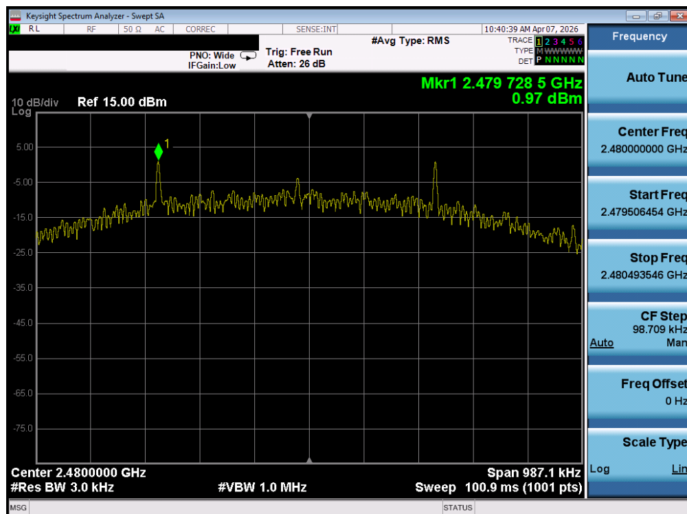
Plot 7-90. Power Spectral Density Plot (Bluetooth (LE), 500kbps – Ch. 39) – Ant 2
