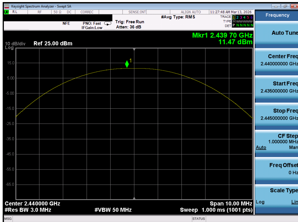
Plot 7-38. Peak Power Plot (Bluetooth (LE), 125kbps – Ch. 17) – Ant 1
