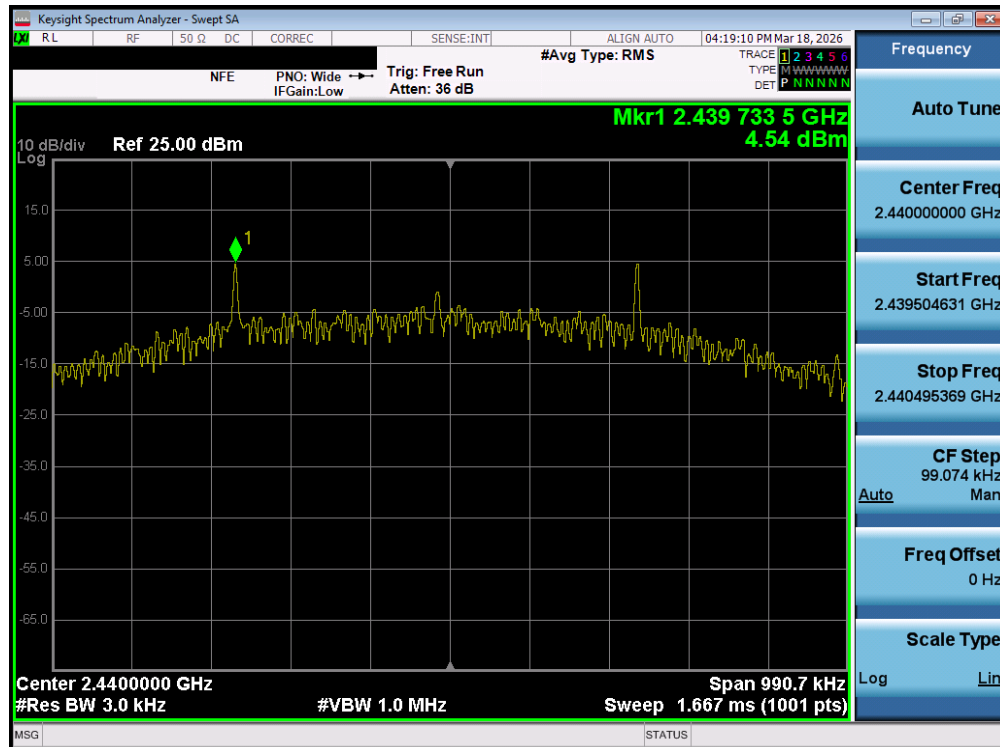
Plot 7-77. Power Spectral Density Plot (Bluetooth (LE), 500kbps – Ch. 17) – Ant 1
