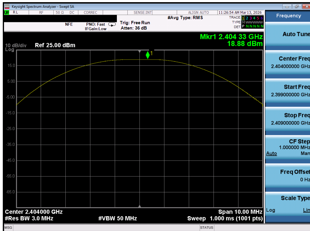
Plot 7-46. Peak Power Plot (Bluetooth (LE), 2Mbps – Ch. 0) – Ant 1
