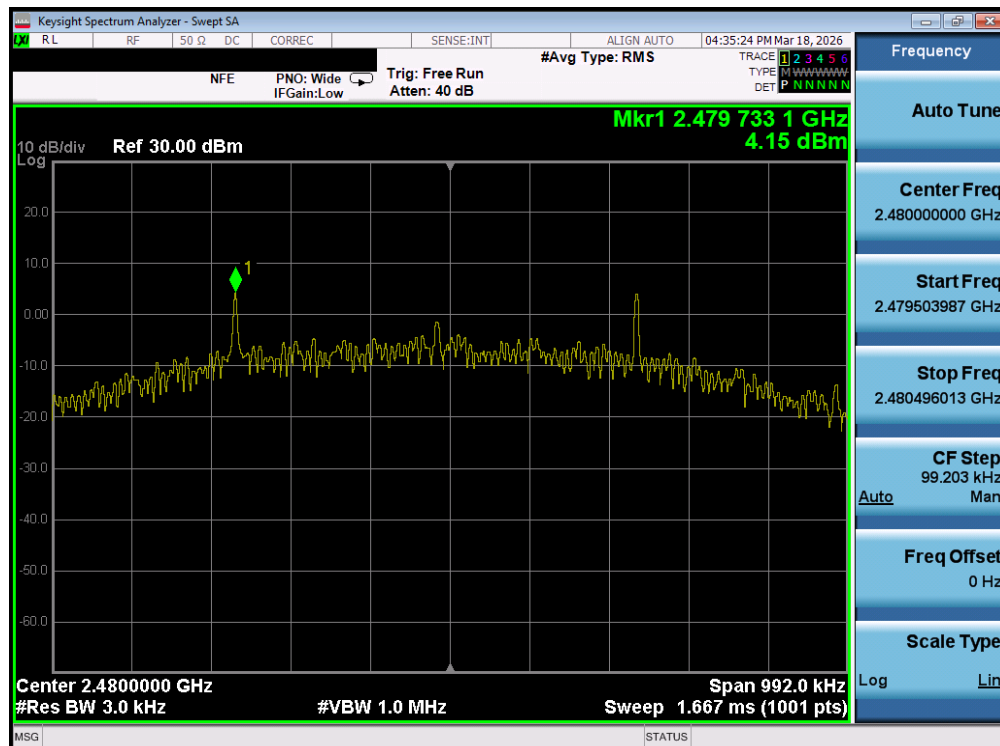
Plot 7-78. Power Spectral Density Plot (Bluetooth (LE), 500kbps – Ch. 39) – Ant 1
