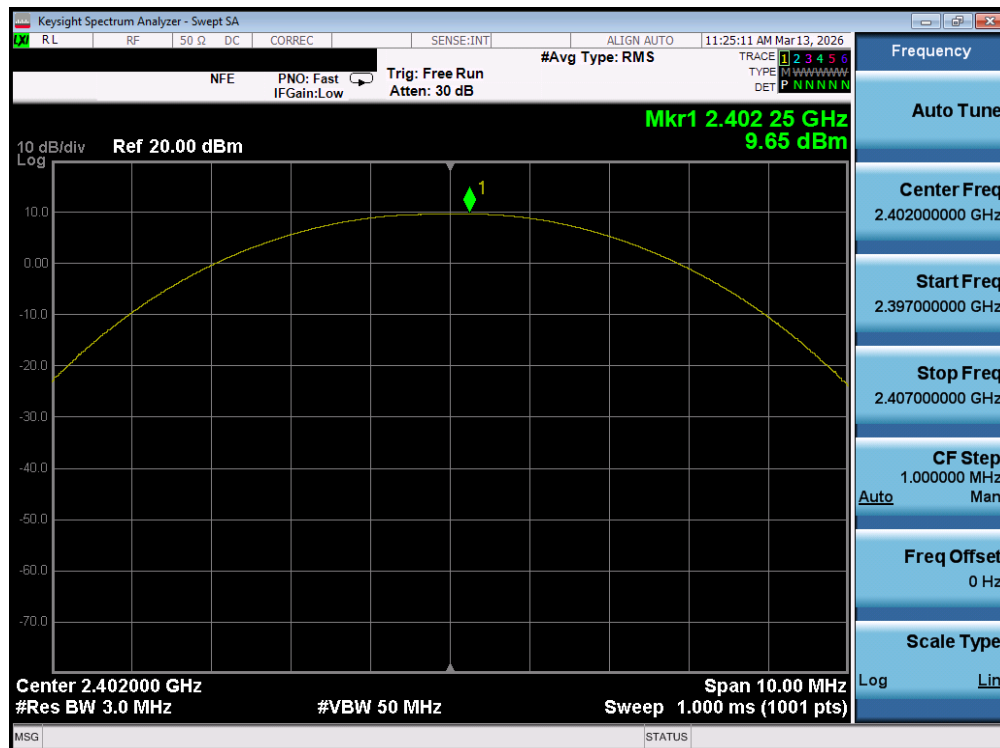
Plot 7-40. Peak Power Plot (Bluetooth (LE), 500kbps – Ch. 37) – Ant 1
