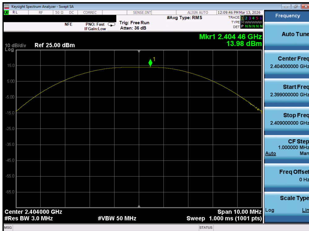
Plot 7-64. Peak Power Plot (Bluetooth (LE), 2Mbps – Ch. 0) – Dual Ant 1
