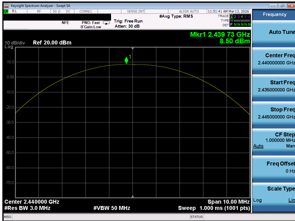
Plot 7-53. Peak Power Plot (Bluetooth (LE), 500kbps – Ch. 17) – Ant 2
