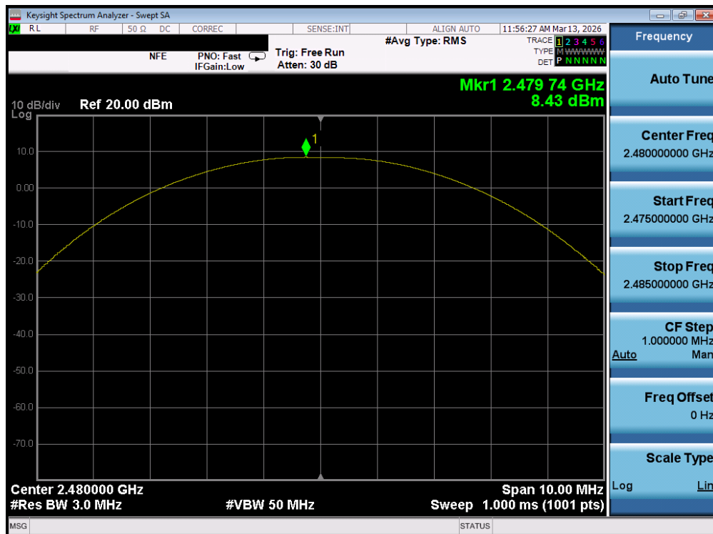
Plot 7-54. Peak Power Plot (Bluetooth (LE), 500kbps – Ch. 39) – Ant 2
