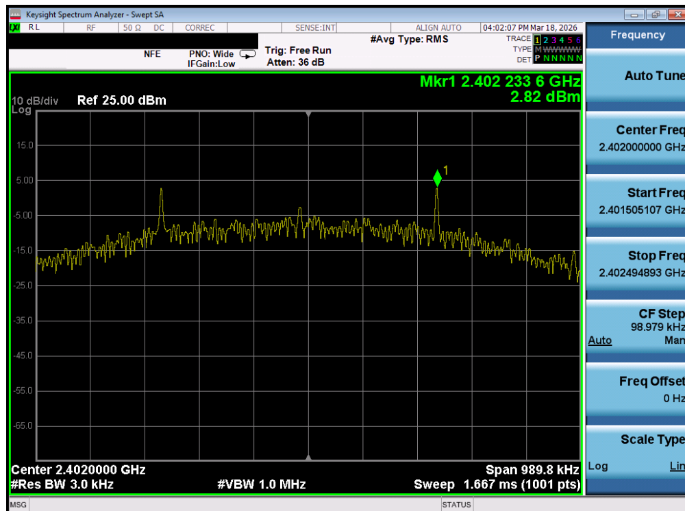
Plot 7-76. Power Spectral Density Plot (Bluetooth (LE), 500kbps – Ch. 37) – Ant 1
