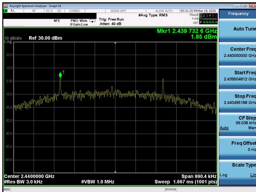
Plot 7-89. Power Spectral Density Plot (Bluetooth (LE), 500kbps – Ch. 17) – Ant 2
