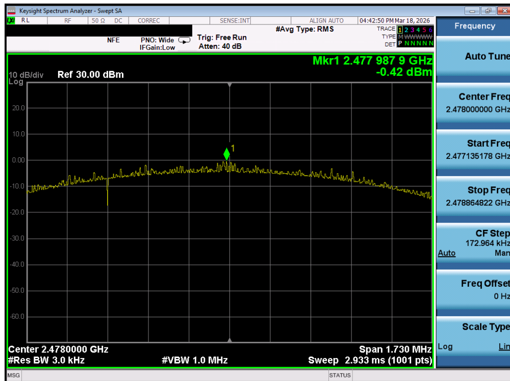
Plot 7-84. Power Spectral Density Plot (Bluetooth (LE), 2Mbps – Ch. 36) – Ant 1
