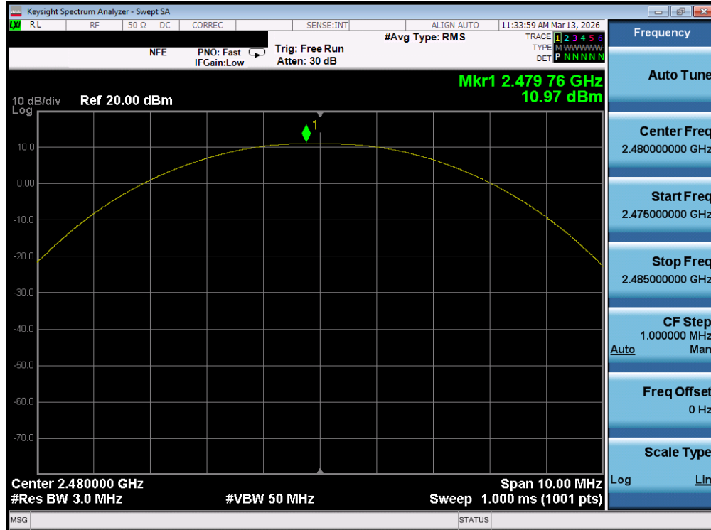
Plot 7-39. Peak Power Plot (Bluetooth (LE), 125kbps – Ch. 39) – Ant 1
