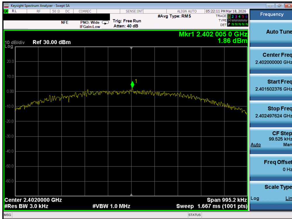
Plot 7-91. Power Spectral Density Plot (Bluetooth (LE), 1Mbps – Ch. 37) – Ant 2
