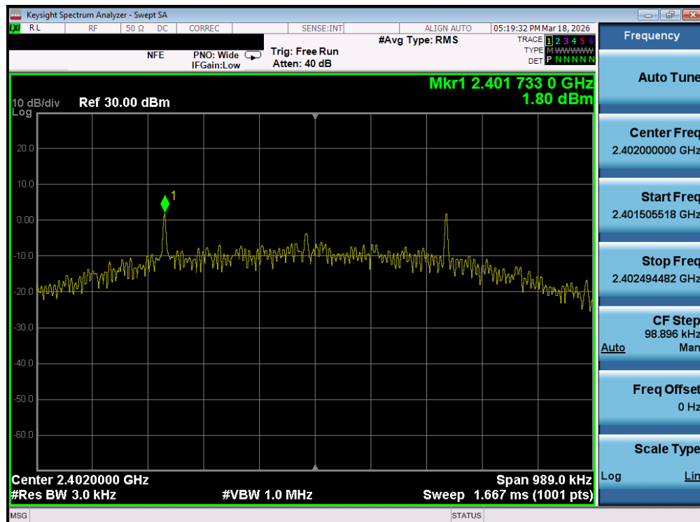
Plot 7-88. Power Spectral Density Plot (Bluetooth (LE), 500kbps – Ch. 37) – Ant 2
