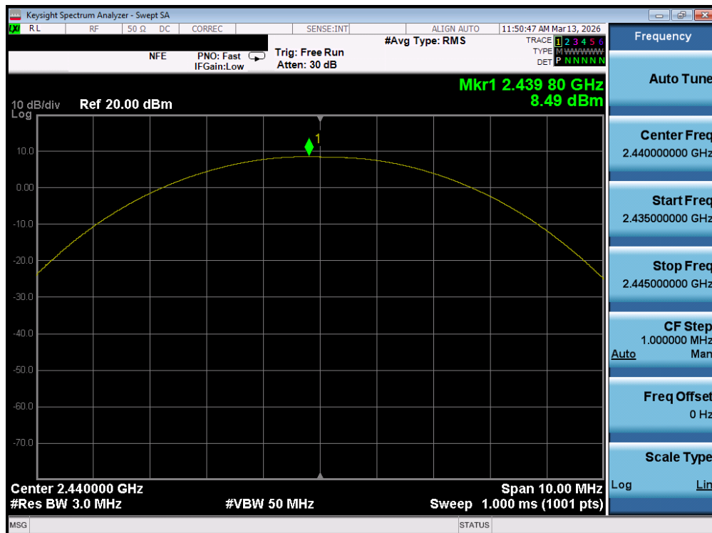
Plot 7-50. Peak Power Plot (Bluetooth (LE), 125kbps – Ch. 17) – Ant 2
