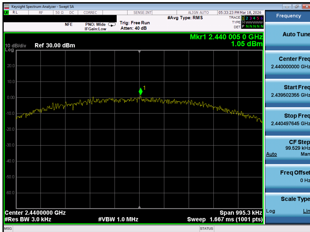
Plot 7-92. Power Spectral Density Plot (Bluetooth (LE), 1Mbps – Ch. 17) – Ant 2
