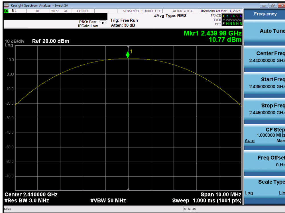
Plot 7-41. Peak Power Plot (Bluetooth (LE), 500kbps – Ch. 17) – Ant 1
