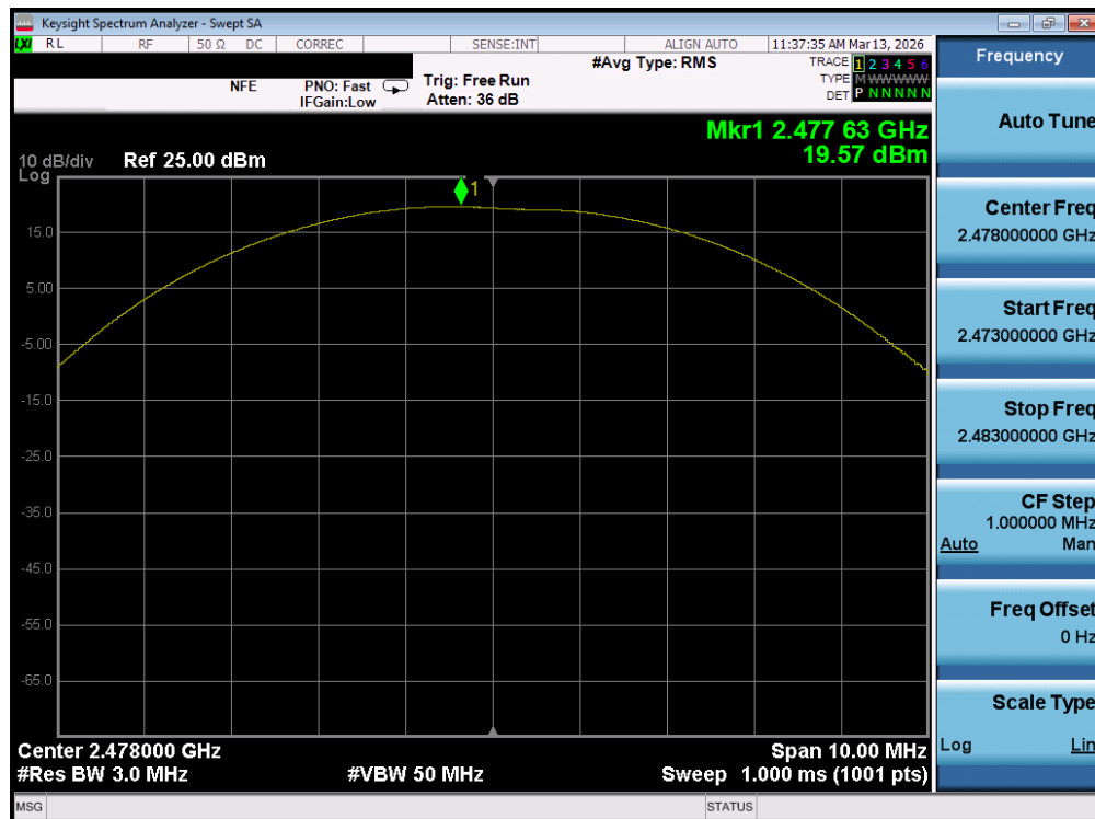
Plot 7-48. Peak Power Plot (Bluetooth (LE), 2Mbps – Ch. 36) – Ant 1
