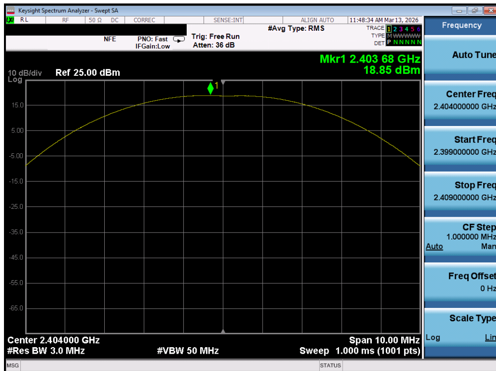
Plot 7-58. Peak Power Plot (Bluetooth (LE), 2Mbps – Ch. 0) – Ant 2
