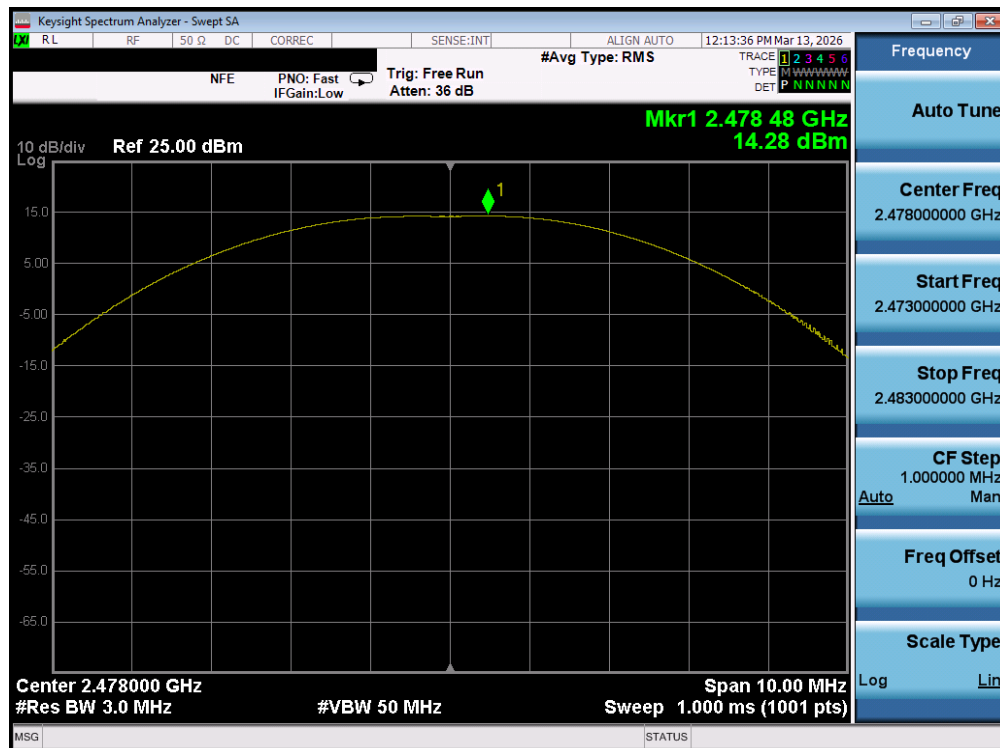
Plot 7-66. Peak Power Plot (Bluetooth (LE), 2Mbps - Ch. 36) - Dual Ant 1
