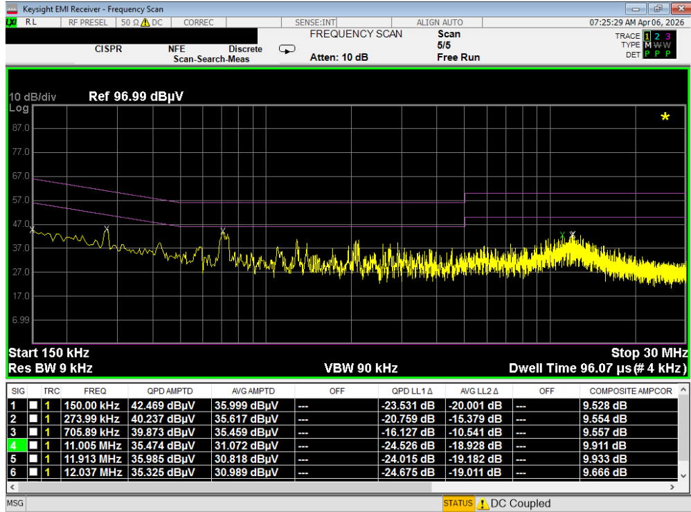
Plot 7-185. Line-Conducted Test Plot (L1) - WCP
