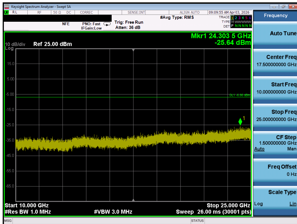
Plot 7-164. Conducted Spurious Plot (Bluetooth, 1Mbps – Ch. 78) – MIMO ANT 2
