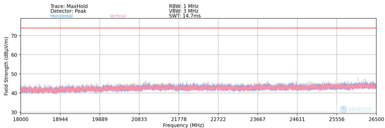
Plot 7-176. Radiated Spurious Plot above 18GHz – MIMO
