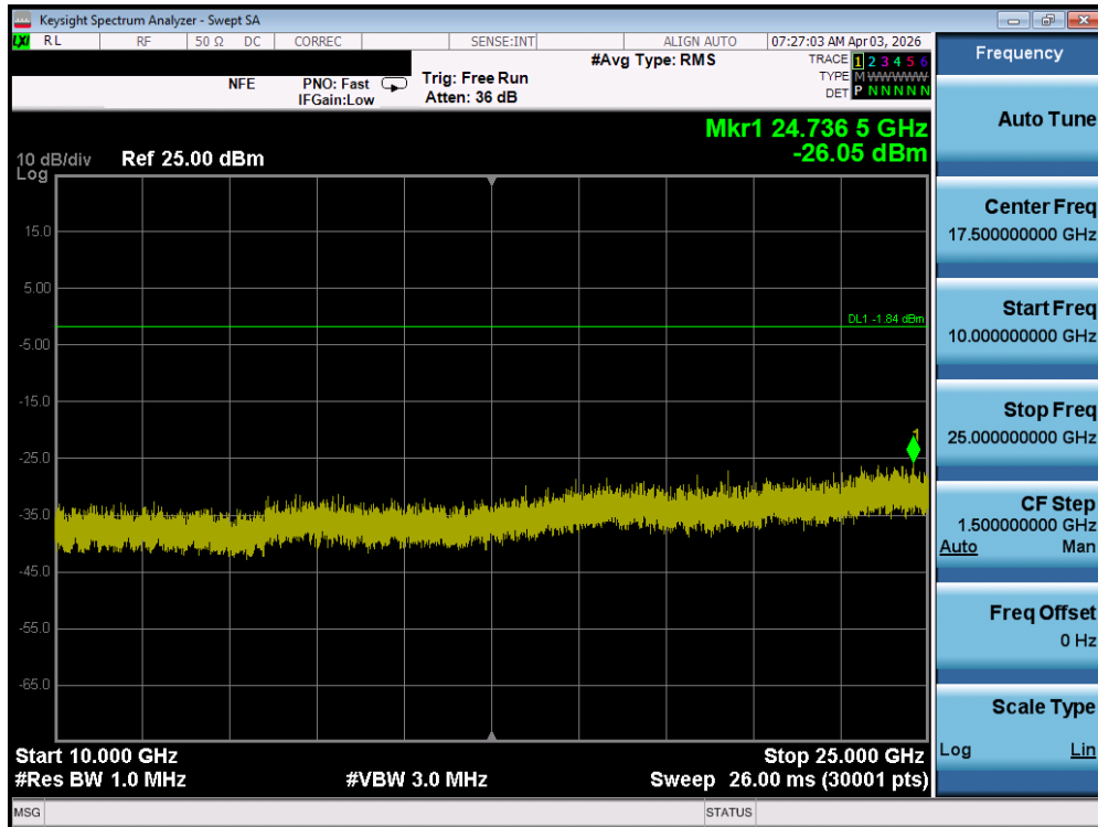
Plot 7-142. Conducted Spurious Plot (Bluetooth, 1Mbps – Ch. 0) – SISO ANT 1
