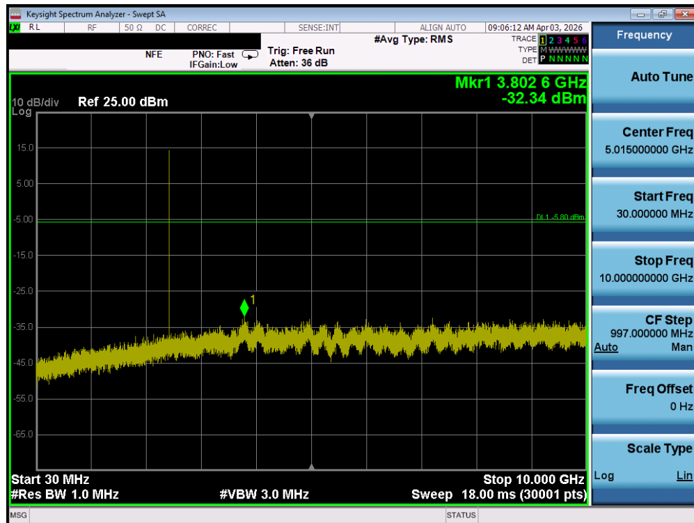
Plot 7-155. Conducted Spurious Plot (Bluetooth, 1Mbps – Ch. 39) – MIMO ANT 1
