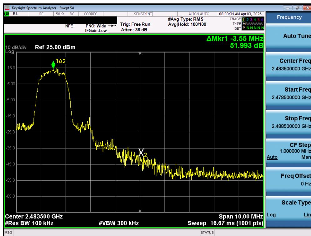
Plot 7-114. Band Edge Plot (Bluetooth with Hopping Disabled, 3 Mbps – Ch. 78) – SISO ANT 2
