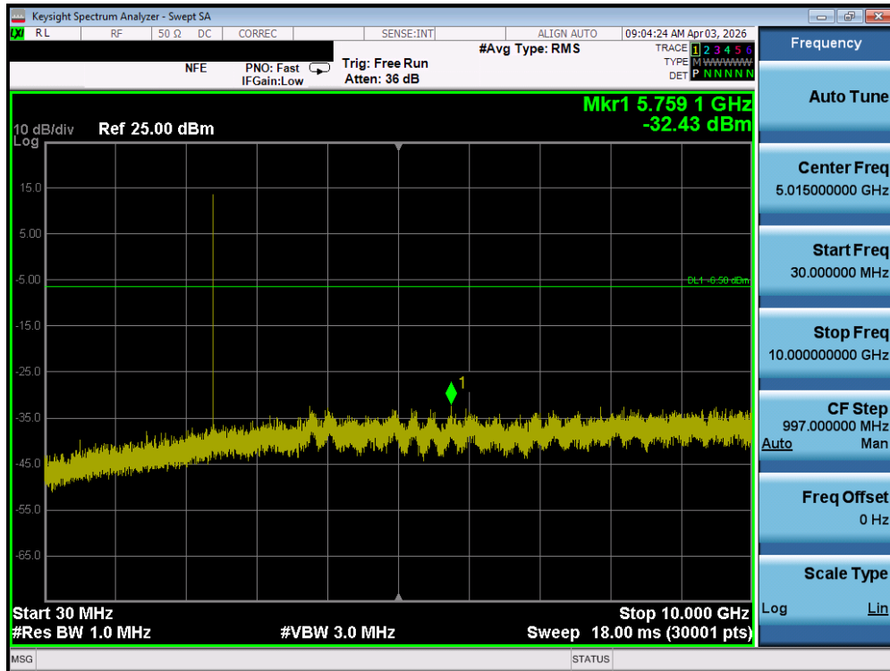
Plot 7-159. Conducted Spurious Plot (Bluetooth, 1Mbps – Ch. 0) – MIMO ANT 2
