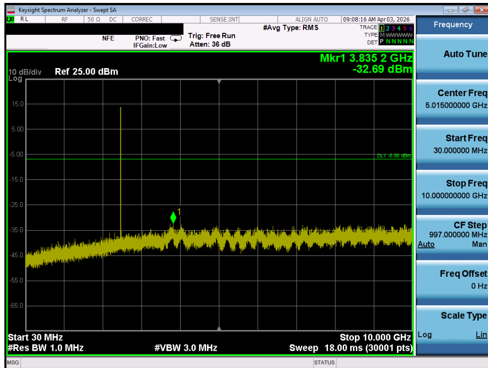
Plot 7-163. Conducted Spurious Plot (Bluetooth, 1Mbps – Ch. 78) – MIMO ANT 2
