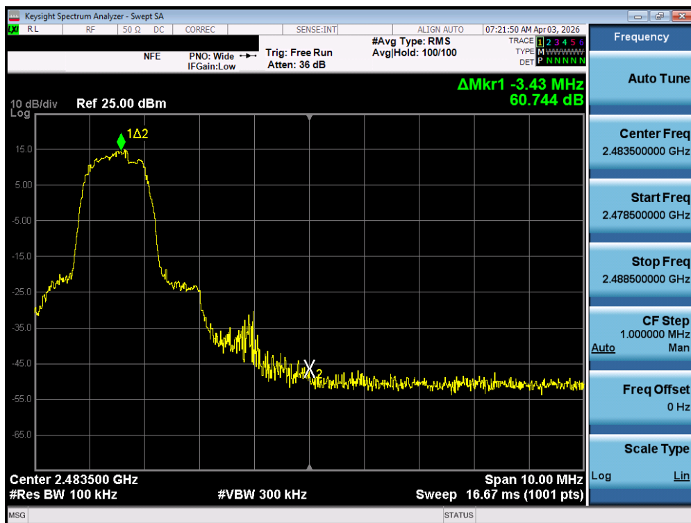
Plot 7-110. Band Edge Plot (Bluetooth with Hopping Disabled, 3 Mbps – Ch. 78) – SISO ANT 1
