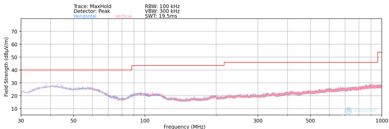
Plot 7-190. Radiated Spurious Plot below 1GHz – Ant 2
