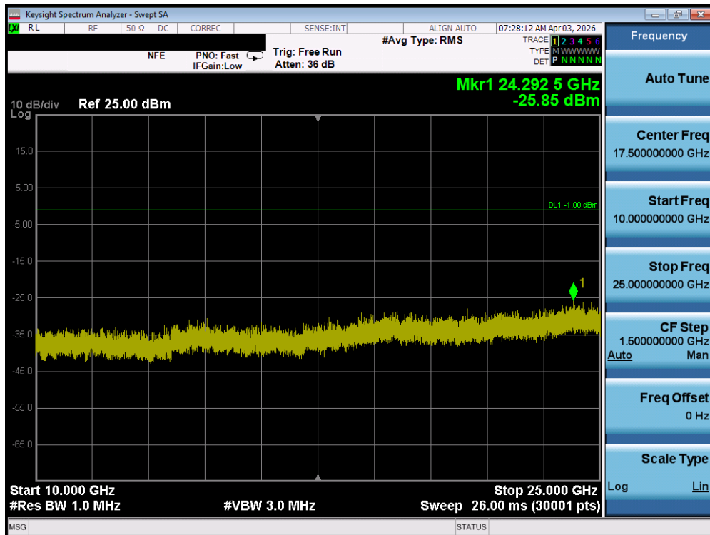
Plot 7-150. Conducted Spurious Plot (Bluetooth, 1Mbps – Ch. 39) – SISO ANT 2
