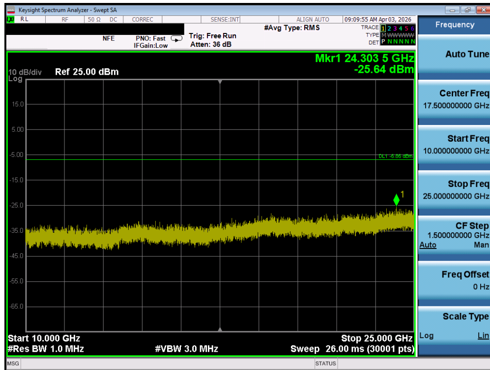
Plot 7-158. Conducted Spurious Plot (Bluetooth, 1Mbps – Ch. 78) – MIMO ANT 1
