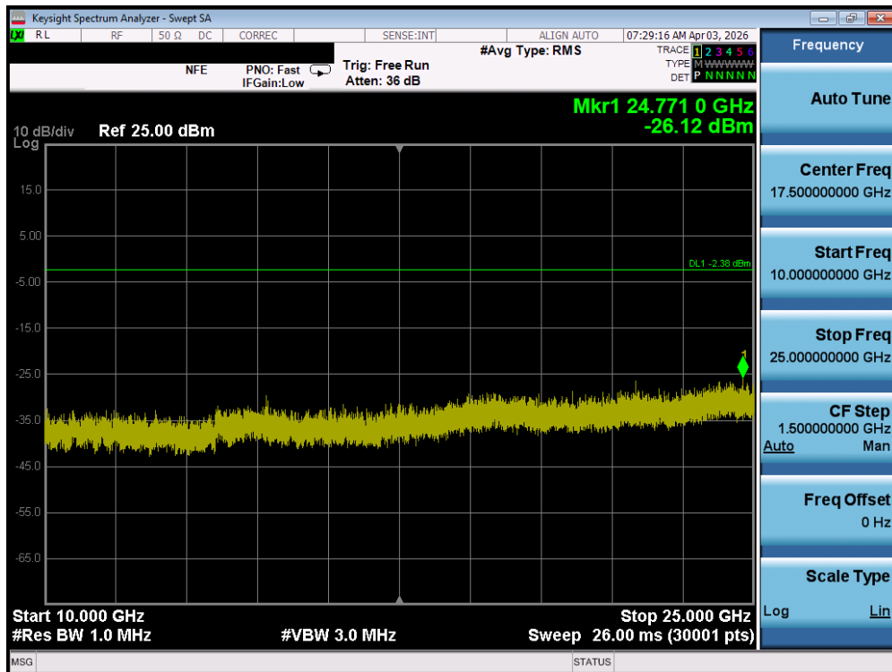
Plot 7-152. Conducted Spurious Plot (Bluetooth, 1Mbps – Ch. 78) – SISO ANT 2
