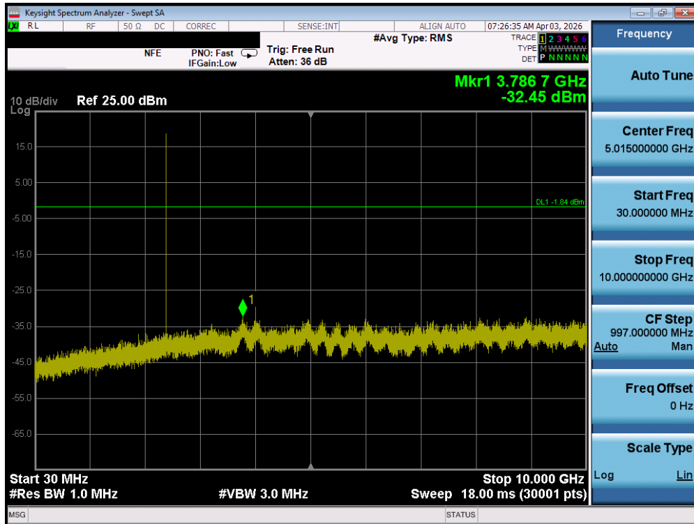
Plot 7-141. Conducted Spurious Plot (Bluetooth, 1Mbps – Ch. 0) – SISO ANT 1
