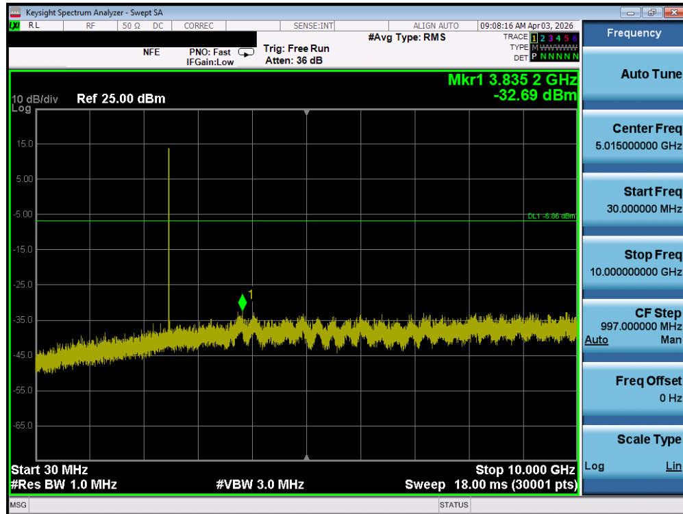
Plot 7-157. Conducted Spurious Plot (Bluetooth, 1Mbps – Ch. 78) – MIMO ANT 1
