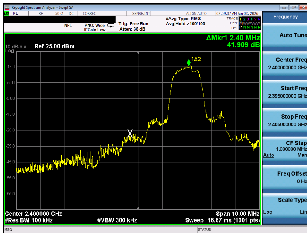
Plot 7-113. Band Edge Plot (Bluetooth with Hopping Disabled, 3 Mbps – Ch. 0) – SISO ANT 2
