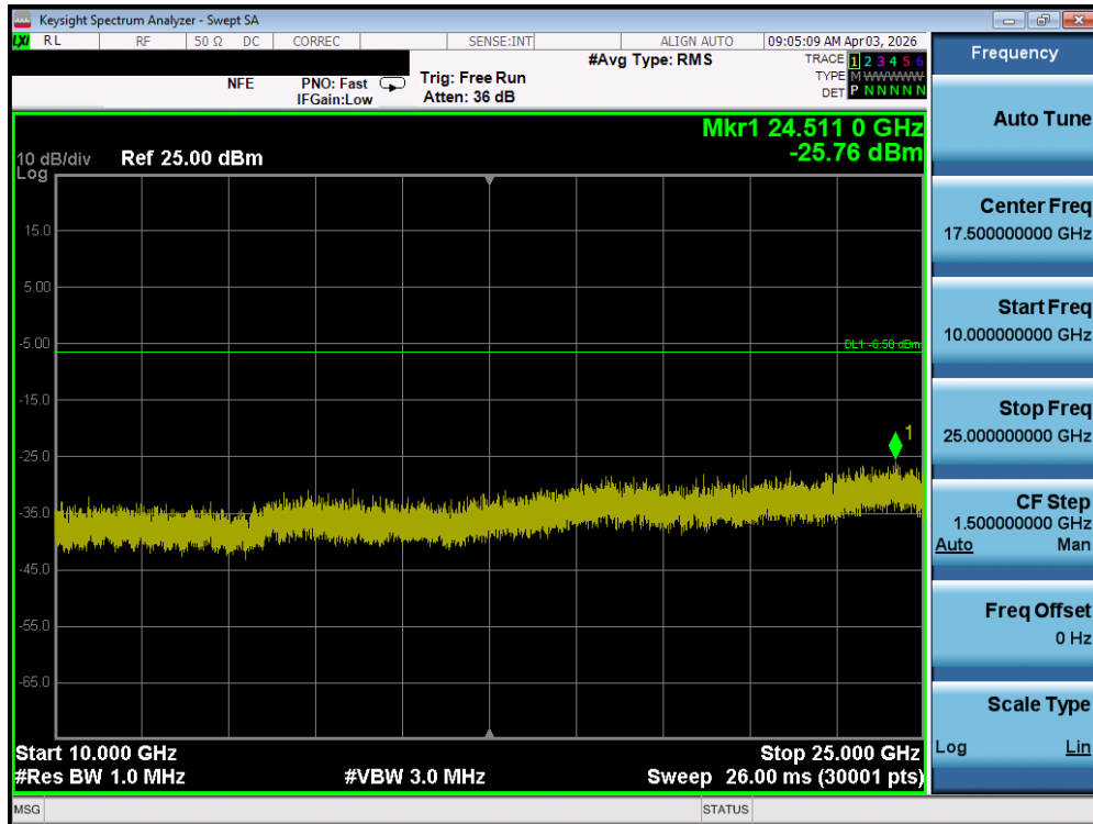
Plot 7-160. Conducted Spurious Plot (Bluetooth, 1Mbps – Ch. 0) – MIMO ANT 2
