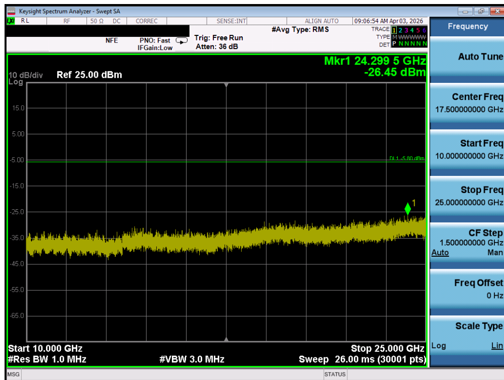
Plot 7-162. Conducted Spurious Plot (Bluetooth, 1Mbps – Ch. 39) – MIMO ANT 2
