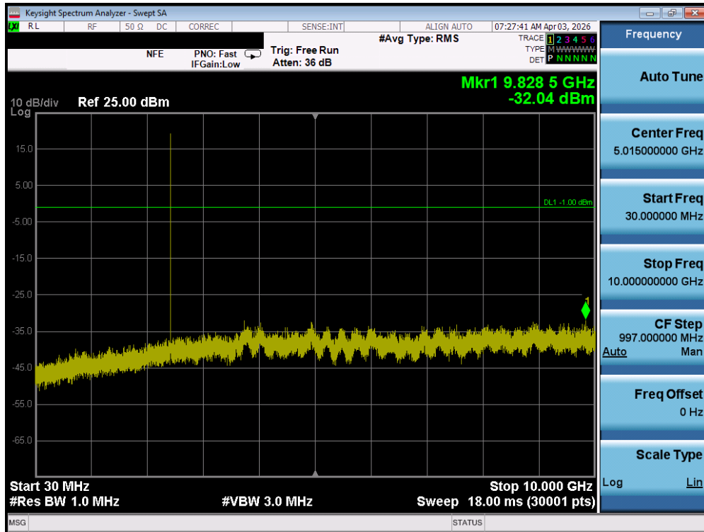
Plot 7-149. Conducted Spurious Plot (Bluetooth, 1Mbps – Ch. 39) – SISO ANT 2
