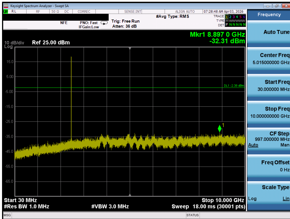
Plot 7-151. Conducted Spurious Plot (Bluetooth, 1Mbps – Ch. 78) – SISO ANT 2
