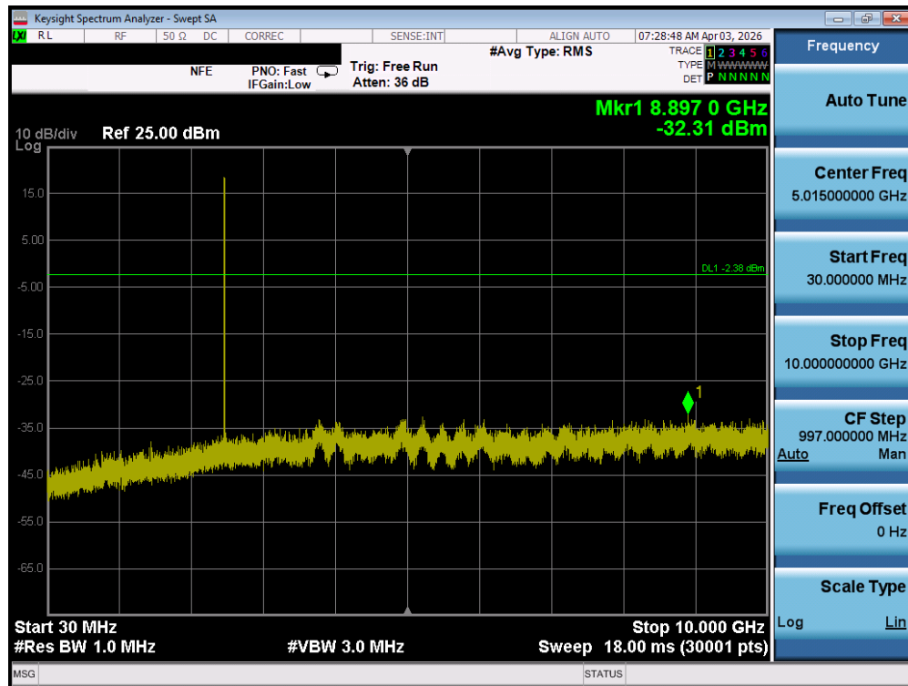
Plot 7-145. Conducted Spurious Plot (Bluetooth, 1Mbps – Ch. 78) – SISO ANT 1
