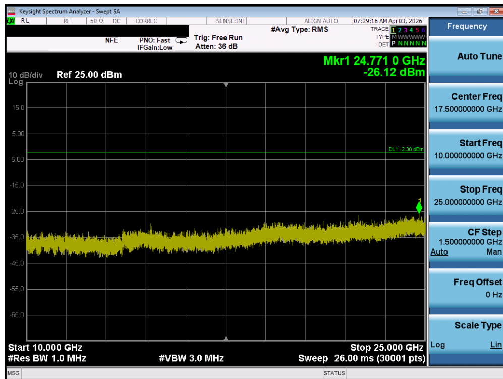
Plot 7-146. Conducted Spurious Plot (Bluetooth, 1Mbps – Ch. 78) – SISO ANT 1
