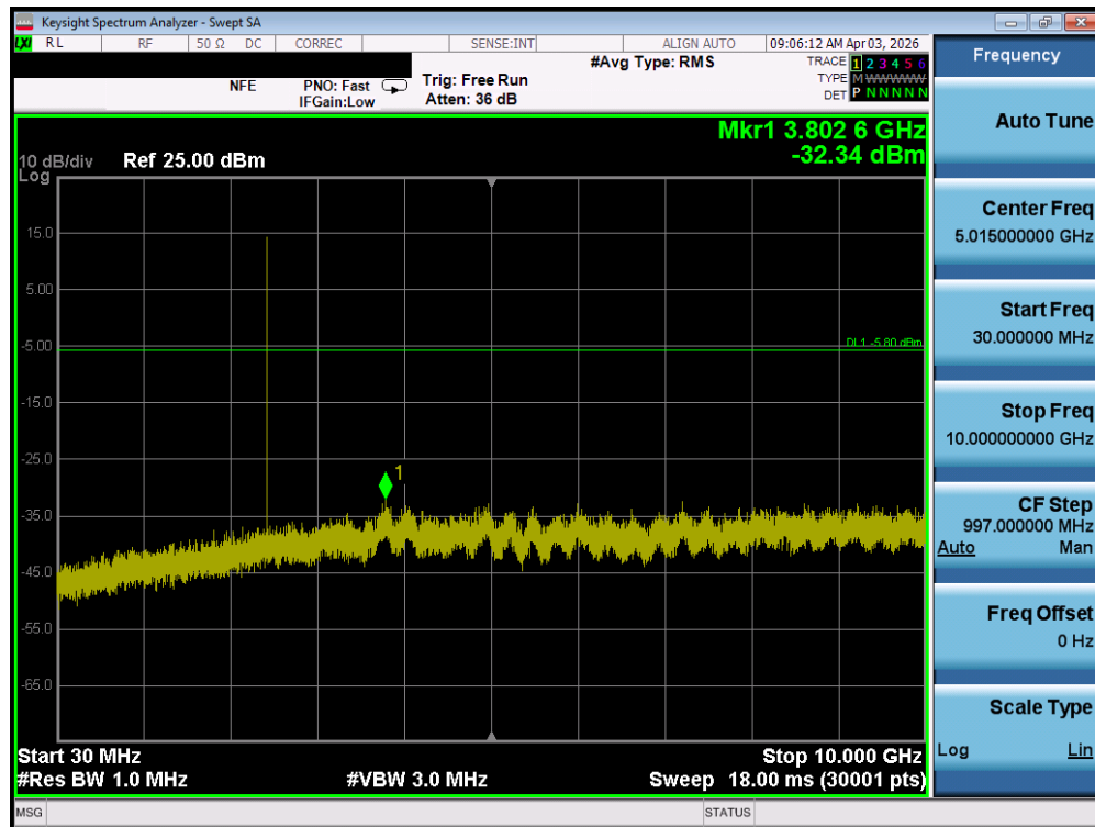
Plot 7-161. Conducted Spurious Plot (Bluetooth, 1Mbps – Ch. 39) – MIMO ANT 2
