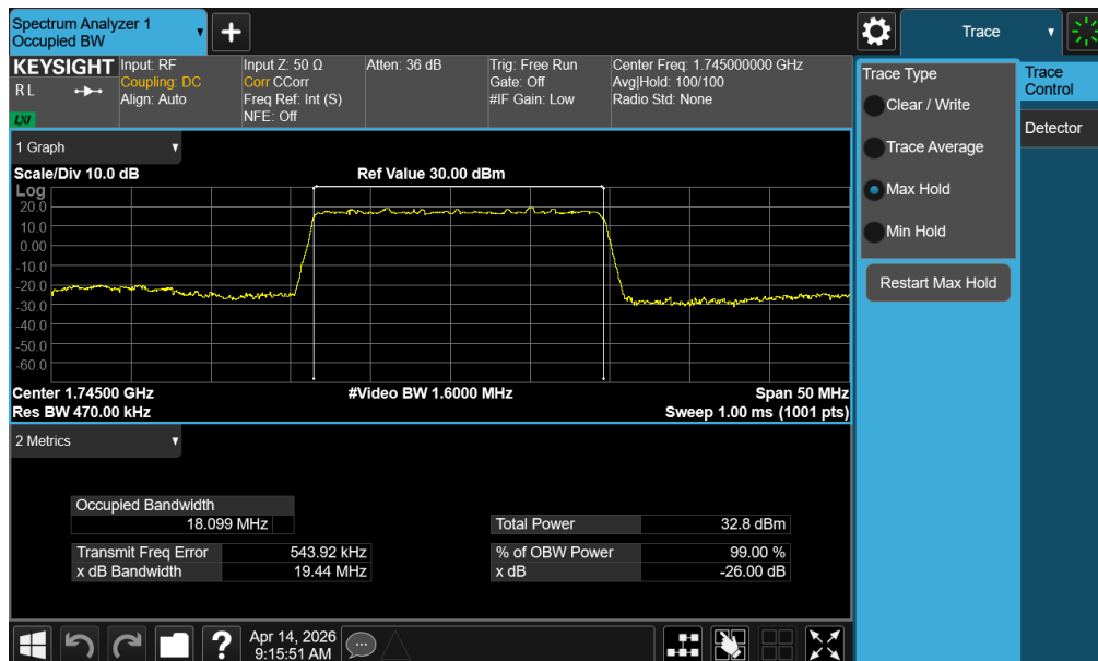
Plot 7-47. Occupied Bandwidth Plot (NR Band n66 - 20.0MHz DFT-s-OFDM BPSK - Full RB – ANT1)
