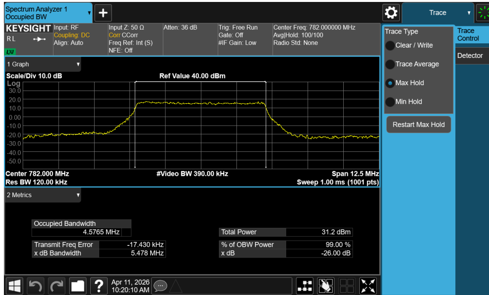
Plot 7-12. Occupied Bandwidth Plot (LTE Band 13 - 5MHz QPSK - Full RB – ANT1)
