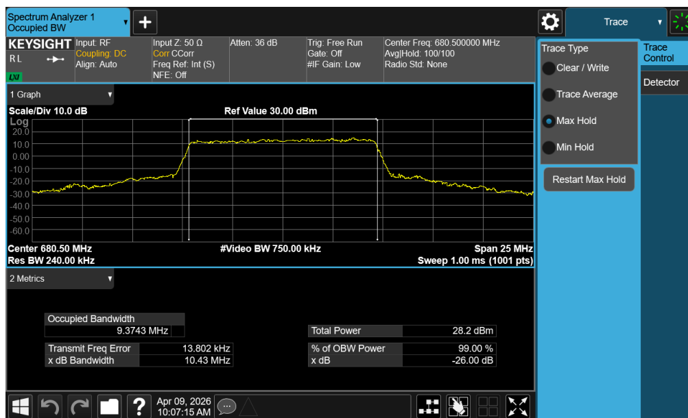
Plot 7-33. Occupied Bandwidth Plot (NR Band n71 - 10MHz CP-OFDM QPSK - Full RB – ANT1)
