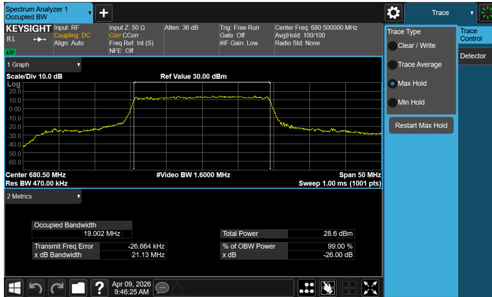
Plot 7-28. Occupied Bandwidth Plot (NR Band n71 - 20MHz CP-OFDM 16-QAM - Full RB – ANT1)
