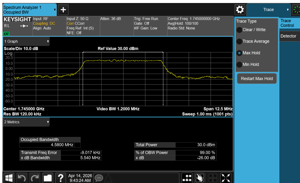
Plot 7-57. Occupied Bandwidth Plot (NR Band n66 - 5.0MHz CP-OFDM QPSK - Full RB – ANT1)
