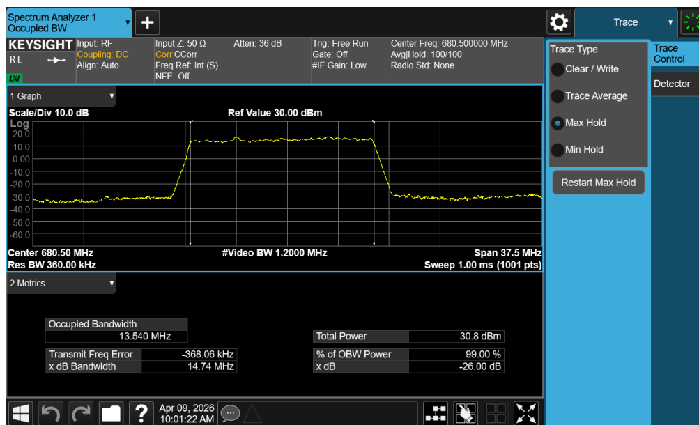
Plot 7-29. Occupied Bandwidth Plot (NR Band n71 - 15MHz DFT-s-OFDM BPSK - Full RB – ANT1)
