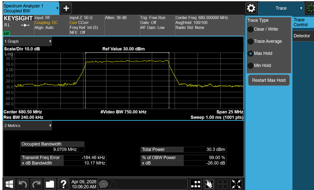
Plot 7-32. Occupied Bandwidth Plot (NR Band n71 - 10MHz DFT-s-OFDM BPSK - Full RB – ANT1)
