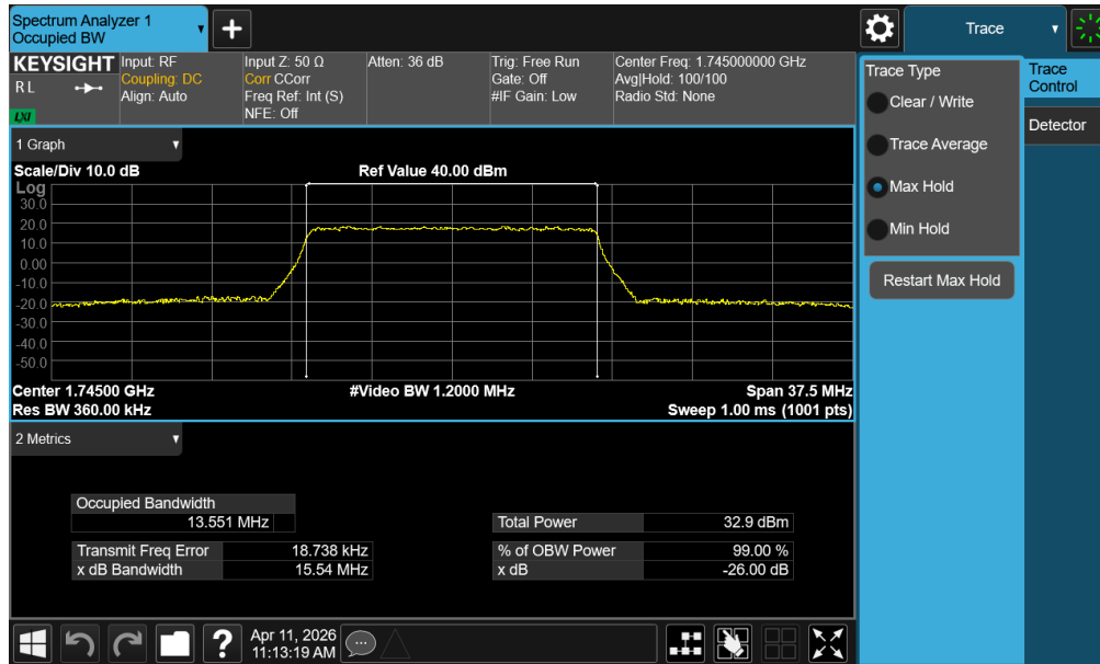
Plot 7-16. Occupied Bandwidth Plot (LTE Band 66/4 - 15MHz QPSK - Full RB - ANT1)
