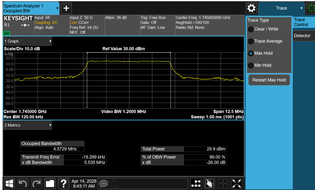
Plot 7-58. Occupied Bandwidth Plot (NR Band n66 - 5.0MHz CP-OFDM 16QAM - Full RB – ANT1)
