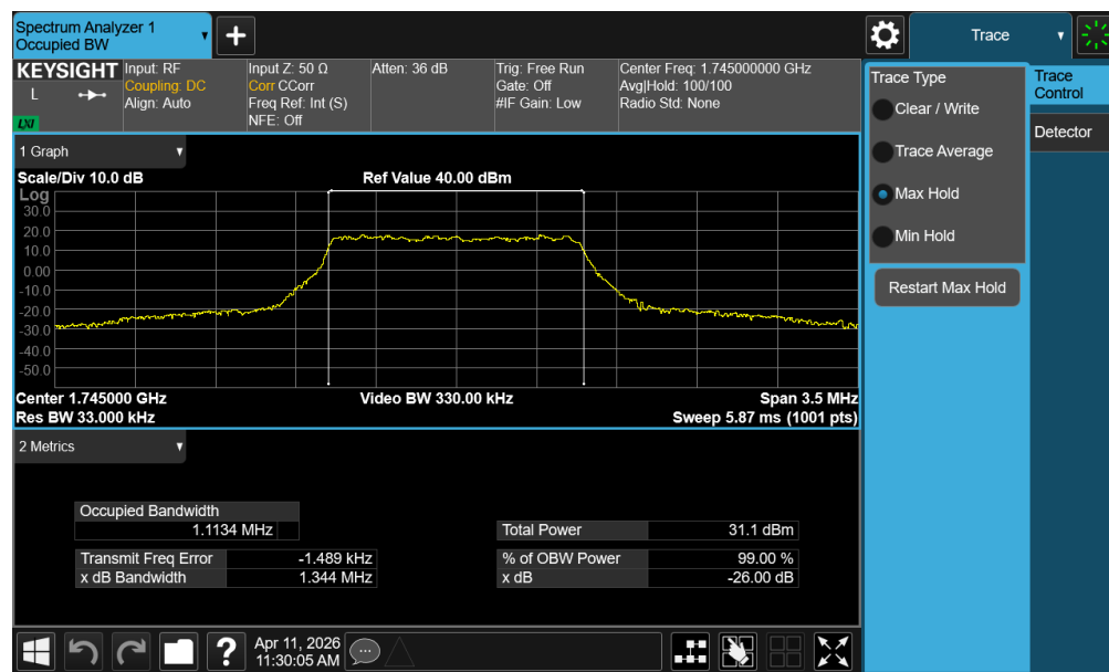
Plot 7-25. Occupied Bandwidth Plot (LTE Band 66/4 - 1.4MHz 16-QAM - Full RB - ANT1)
