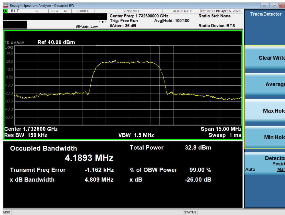
Plot 7-59. Occupied Bandwidth Plot (WCDMA, Ch. 1413 – ANT2)
