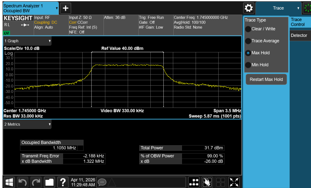
Plot 7-24. Occupied Bandwidth Plot (LTE Band 66/4 - 1.4MHz QPSK - Full RB - ANT1)
