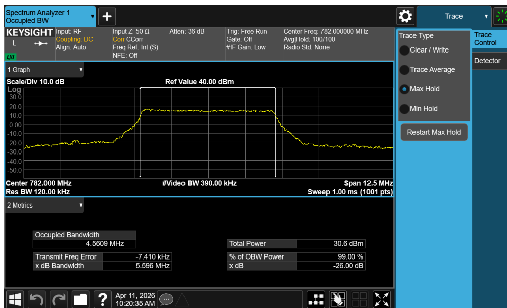
Plot 7-13. Occupied Bandwidth Plot (LTE Band 13 - 5MHz 16-QAM - Full RB – ANT1)
