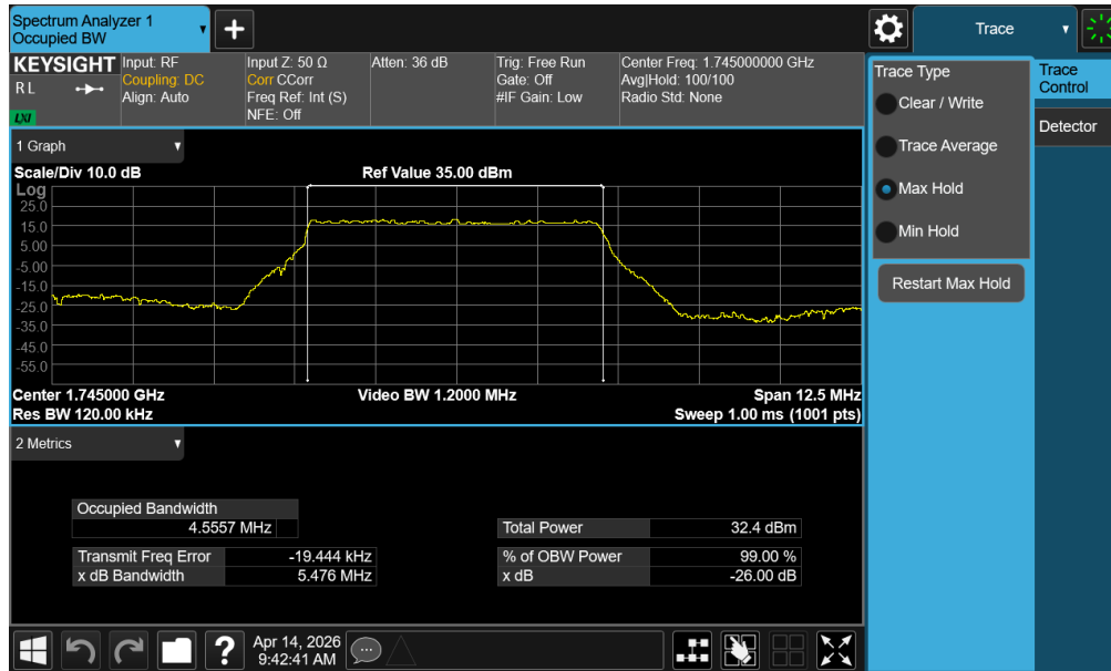
Plot 7-56. Occupied Bandwidth Plot (NR Band n66 - 5.0MHz DFT-s-OFDM BPSK - Full RB – ANT1)
