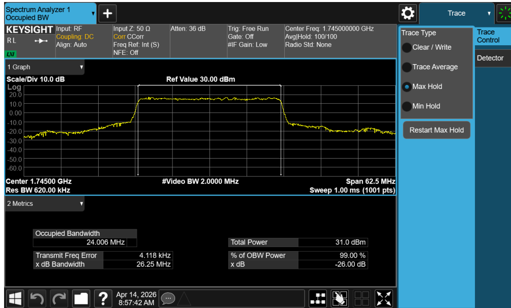
Plot 7-46. Occupied Bandwidth Plot (NR Band n66 - 25.0MHz CP-OFDM 16QAM - Full RB – ANT1)
