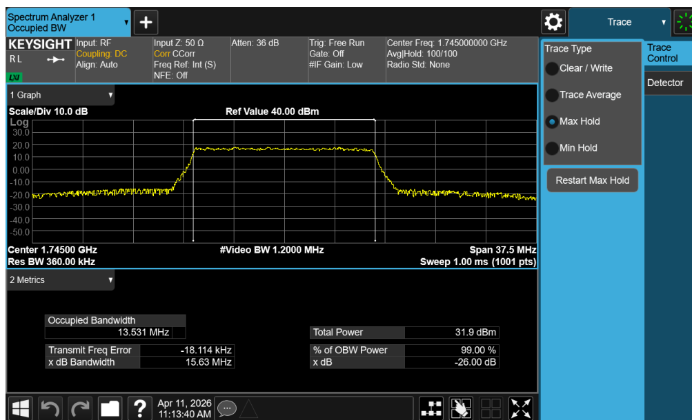
Plot 7-17. Occupied Bandwidth Plot (LTE Band 66/4 - 15MHz 16-QAM - Full RB - ANT1)
