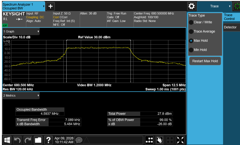
Plot 7-36. Occupied Bandwidth Plot (NR Band n71 - 5MHz CP-OFDM QPSK - Full RB – ANT1)
