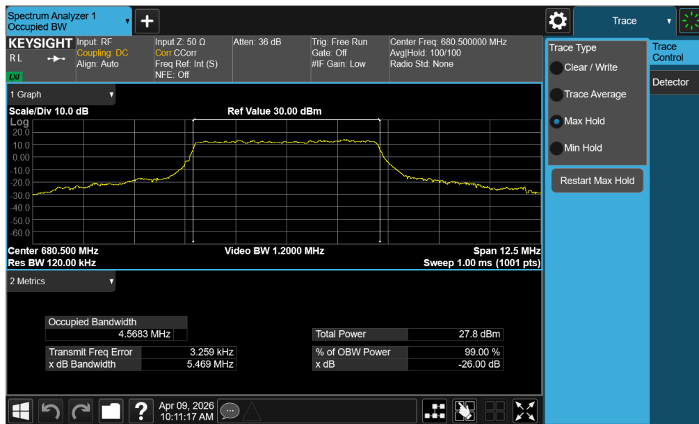
Plot 7-37. Occupied Bandwidth Plot (NR Band n71 - 5MHz CP-OFDM 16-QAM - Full RB – ANT1)
