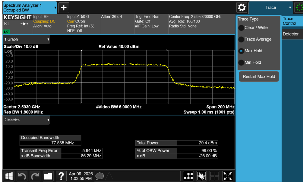
Plot 7-25. Occupied Bandwidth Plot (NR Band n41 PC3 – 80MHz 16-QAM – Full RB – Default – Ant1)
