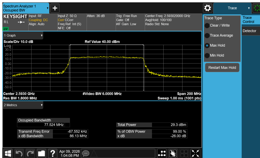
Plot 7-24. Occupied Bandwidth Plot (NR Band n41 PC3 – 80MHz QPSK – Full RB – Default – Ant1)
