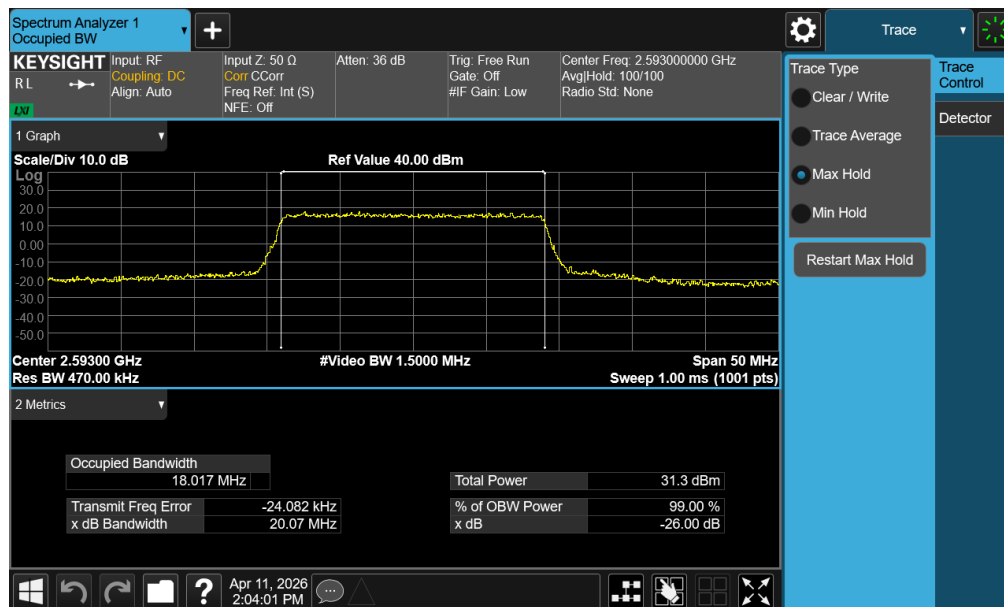
Plot 7-9. Occupied Bandwidth Plot (LTE Band 41(PC3) - 20MHz QPSK - Full RB - Ant1)
