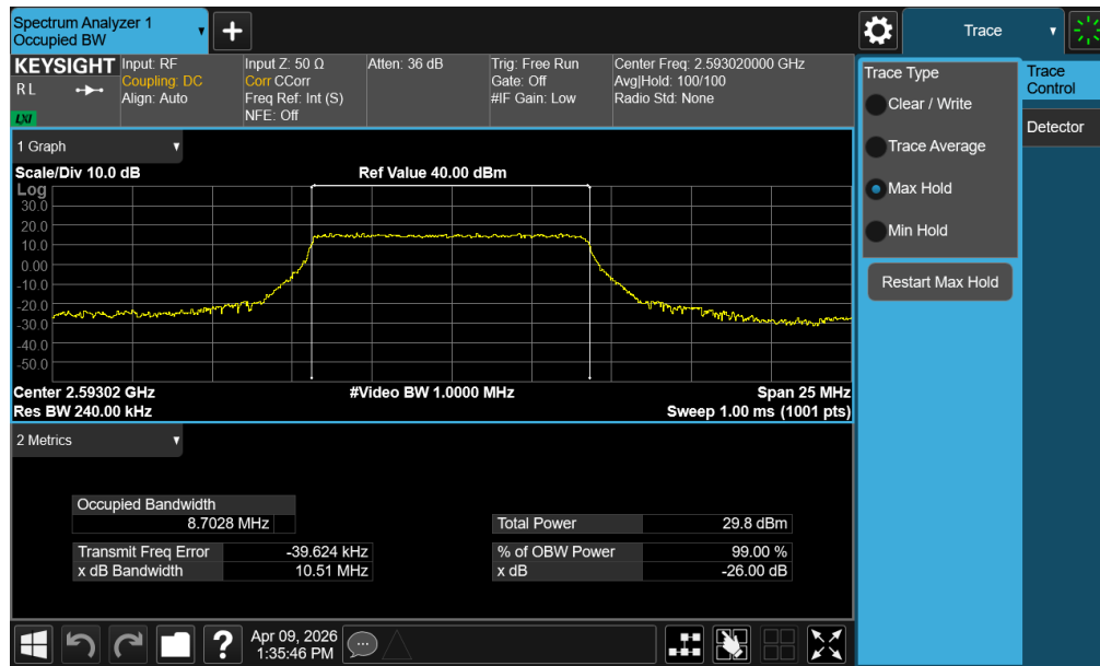
Plot 7-49. Occupied Bandwidth Plot (NR Band n41 PC3 – 10MHz 16-QAM – Full RB – Default – Ant1)
