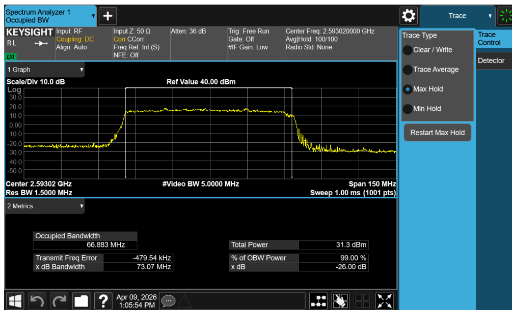
Plot 7-26. Occupied Bandwidth Plot (NR Band n41 PC3 – 70MHz \pi/2 BPSK – Full RB – Default – Ant1)
