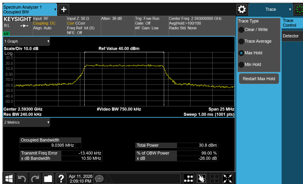
Plot 7-14. Occupied Bandwidth Plot (LTE Band 41(PC3)/38 - 10MHz 16-QAM - Full RB - Ant1)
