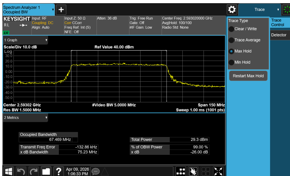
Plot 7-28. Occupied Bandwidth Plot (NR Band n41 PC3 – 70MHz 16-QAM – Full RB – Default – Ant1)
