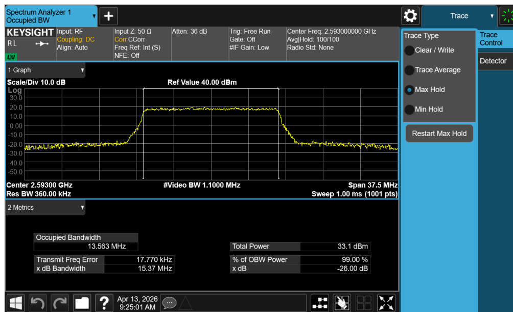
Plot 7-53. Occupied Bandwidth Plot (LTE Band 41(PC2) - 15MHz 16-QAM - Full RB – Ant2)
