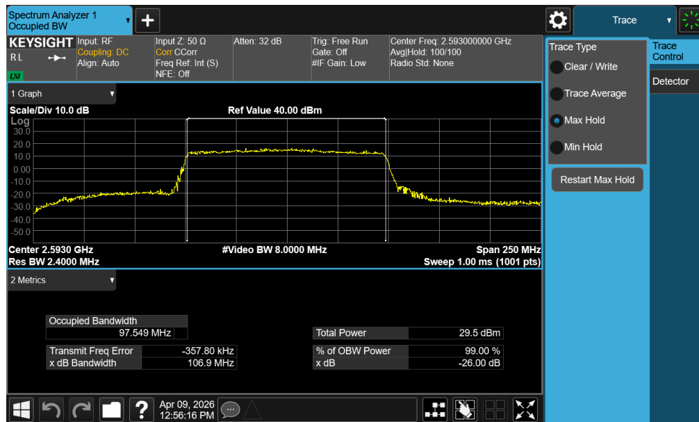
Plot 7-18. Occupied Bandwidth Plot (NR Band n41 PC3 – 100MHz QPSK – Full RB – Default – Ant1)
