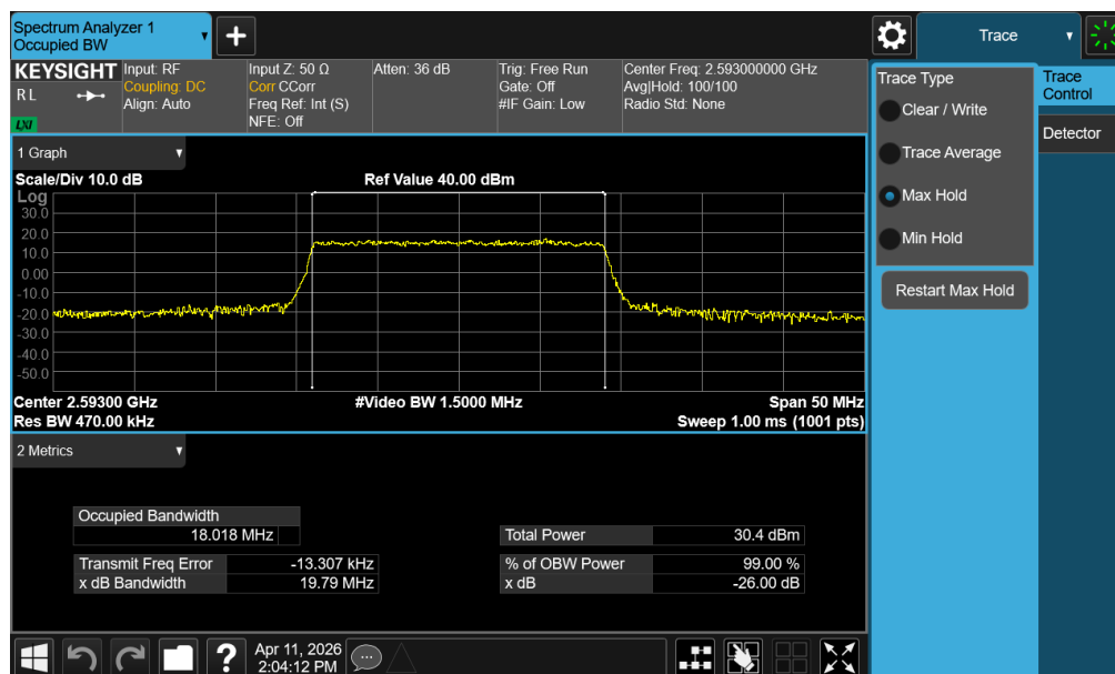
Plot 7-10. Occupied Bandwidth Plot (LTE Band 41(PC3) - 20MHz 16-QAM - Full RB - Ant1)
