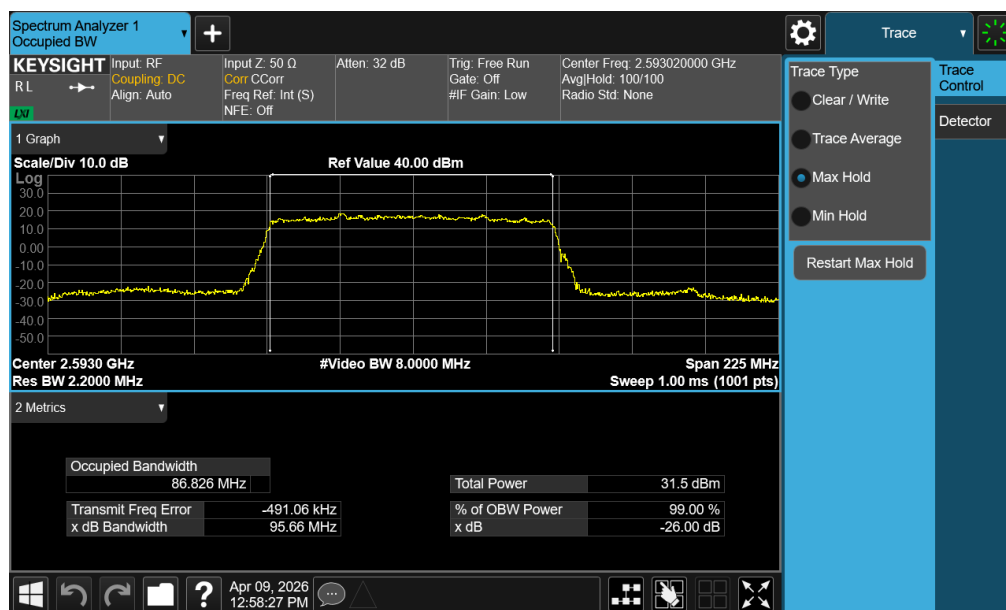
Plot 7-20. Occupied Bandwidth Plot (NR Band n41 PC3 – 90MHz \pi/2 BPSK – Full RB – Default – Ant1)
