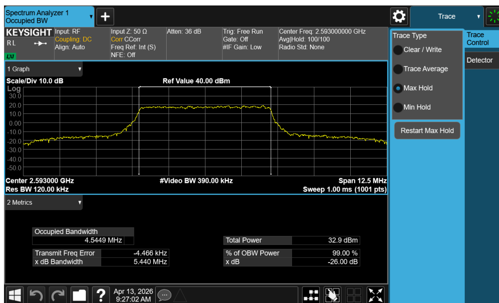
Plot 7-57. Occupied Bandwidth Plot (LTE Band 41(PC2) - 5MHz 16-QAM - Full RB – Ant2)
