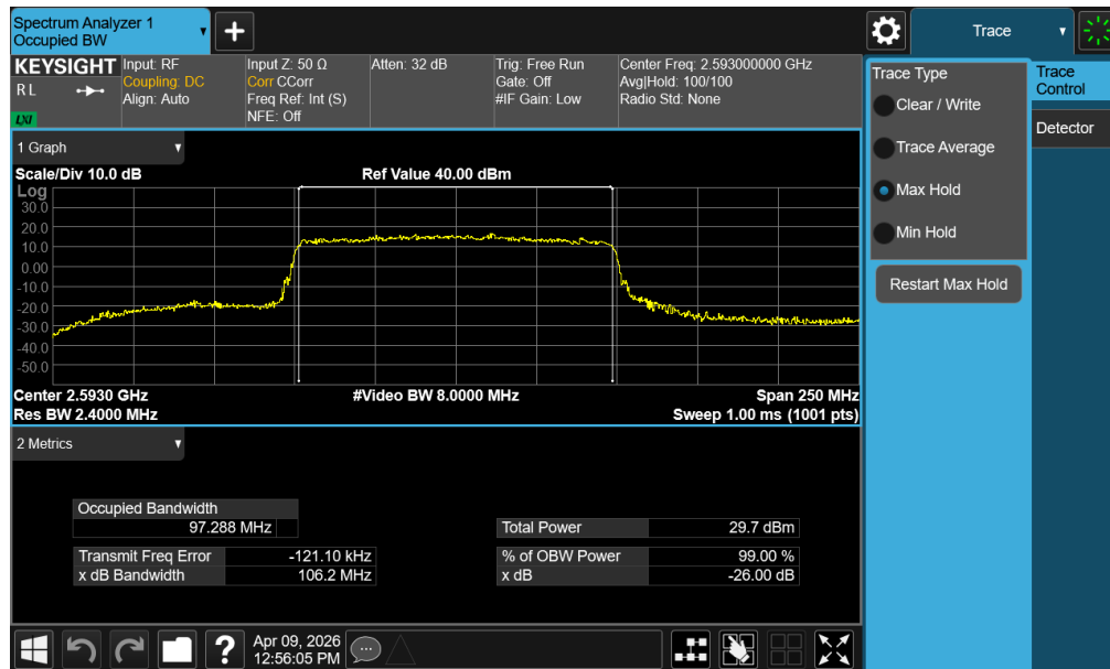
Plot 7-19. Occupied Bandwidth Plot (NR Band n41 PC3 – 100MHz 16-QAM – Full RB – Default – Ant1)
