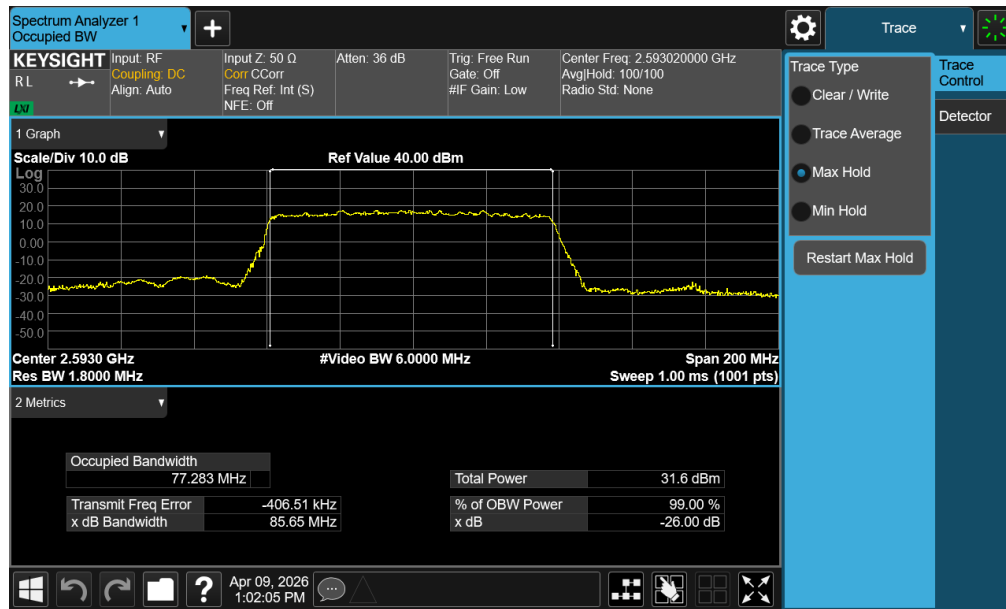
Plot 7-23. Occupied Bandwidth Plot (NR Band n41 PC3 – 80MHz \pi/2 BPSK – Full RB – Default – Ant1)
