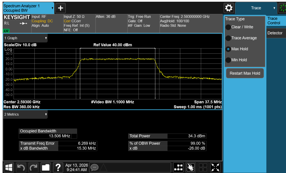
Plot 7-52. Occupied Bandwidth Plot (LTE Band 41(PC2- 15MHz QPSK - Full RB – Ant2)
