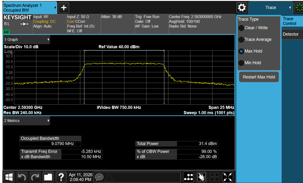
Plot 7-13. Occupied Bandwidth Plot (LTE Band 41(PC3)/38 - 10MHz QPSK - Full RB - Ant1)
