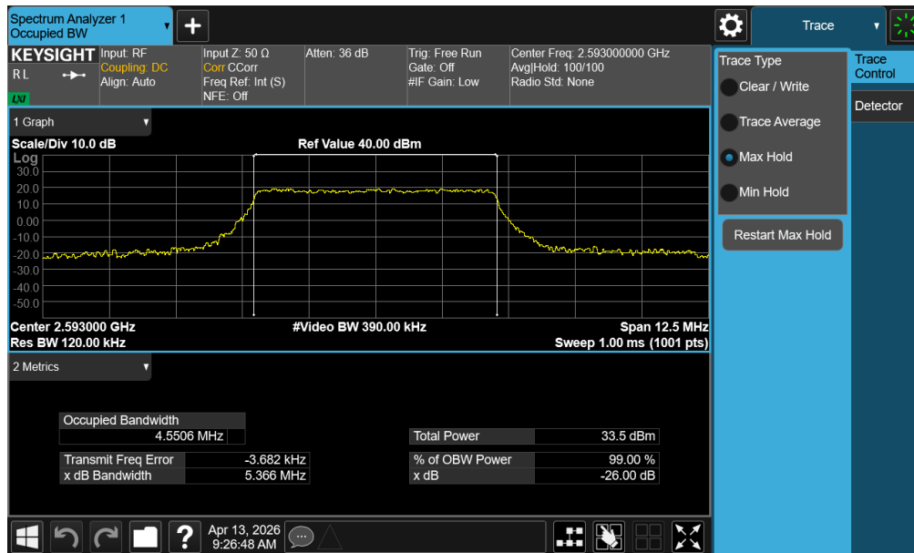
Plot 7-56. Occupied Bandwidth Plot (LTE Band 41(PC2) - 5MHz QPSK - Full RB – Ant2)
