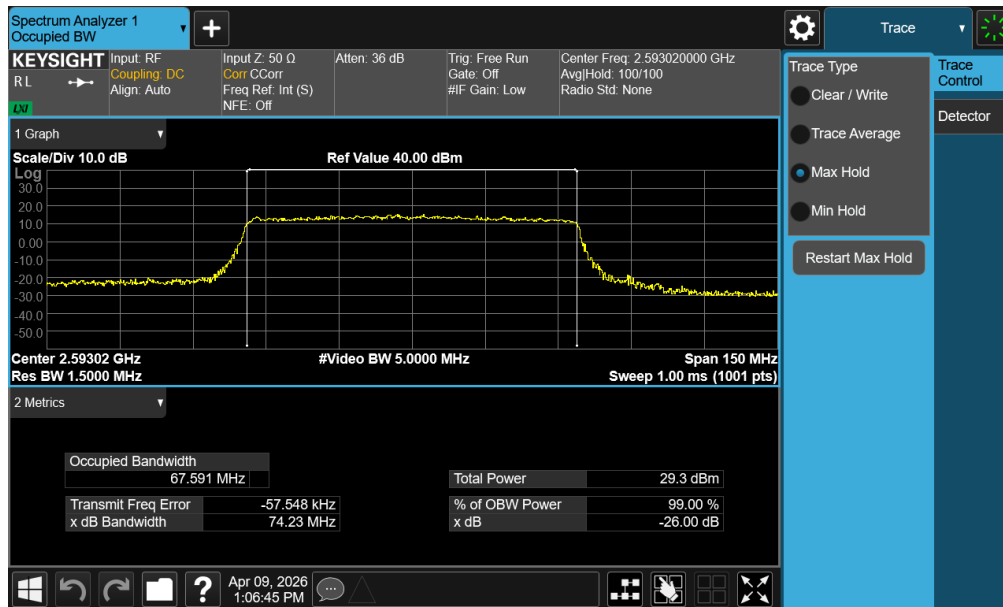
Plot 7-27. Occupied Bandwidth Plot (NR Band n41 PC3 – 70MHz QPSK – Full RB – Default – Ant1)
