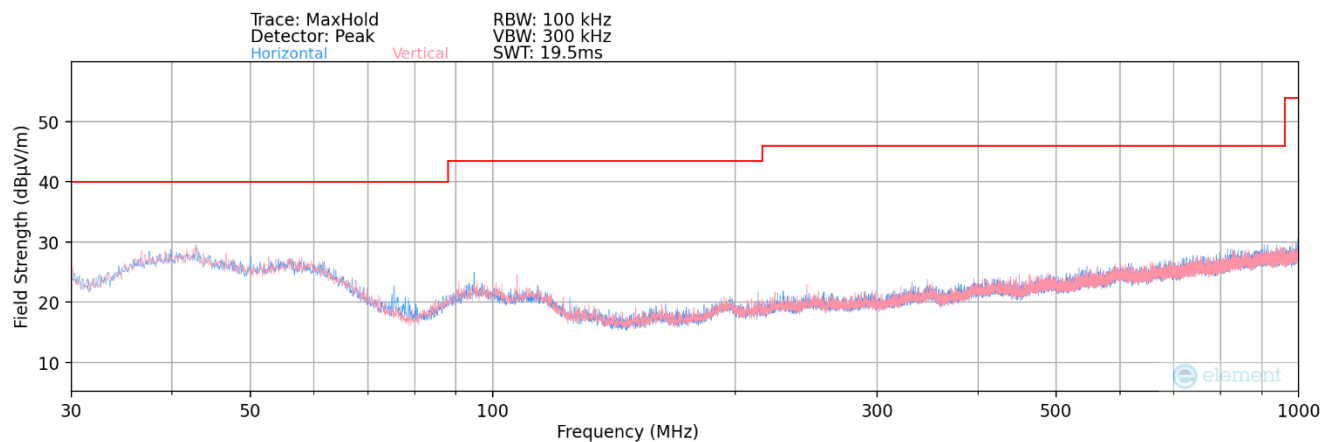
Plot 7-1. Radiated Spurious Plot below 1GHz
