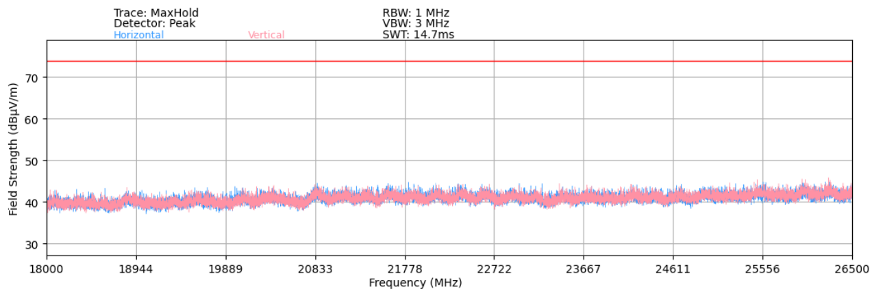
Plot 7-3. Radiated Spurious Plot 18-26.5GHz
