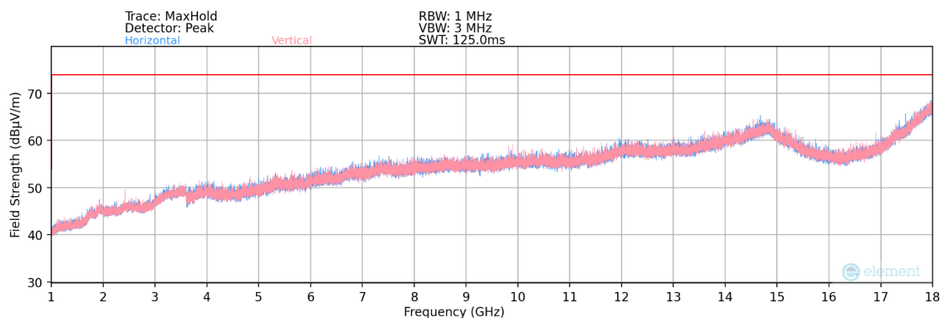
Plot 7-2. Radiated Spurious Plot above 1GHz
