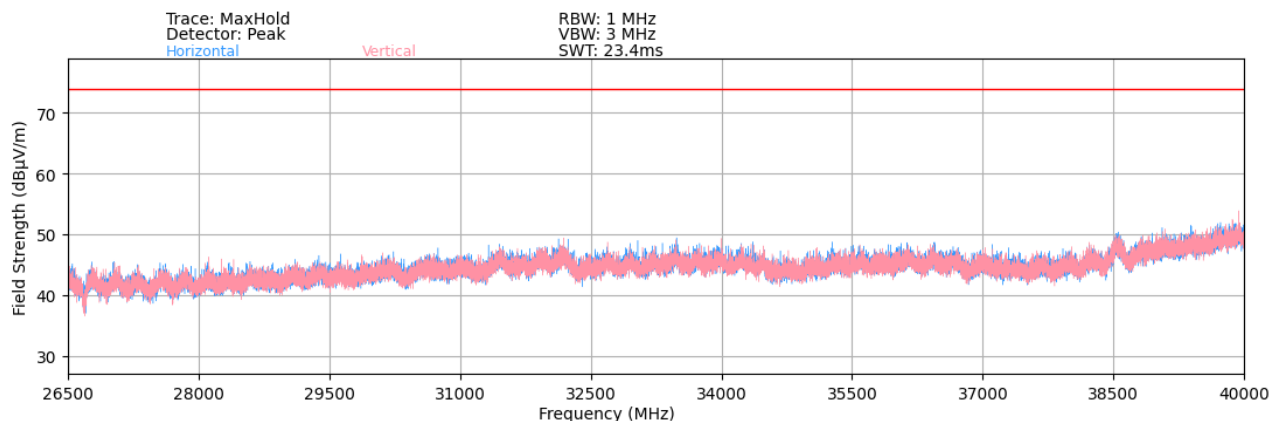
Plot 7-4. Radiated Spurious Plot above 26.5-40GHz
