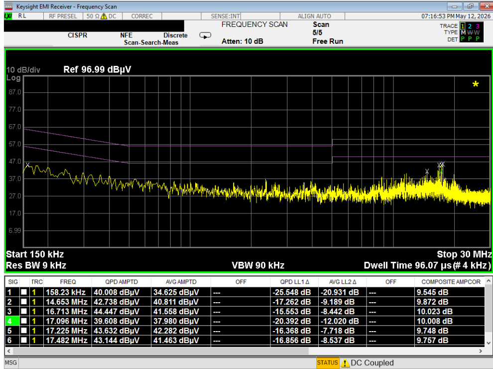
Plot 7-7. Line-Conducted Test Plot (L1) – WCP
