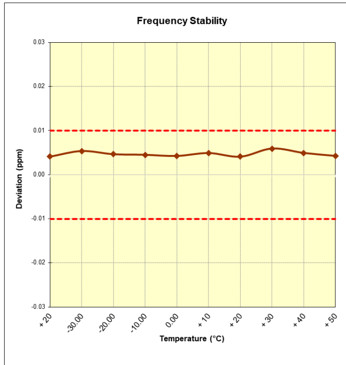
Figure 7-3. Frequency Stability Plot
