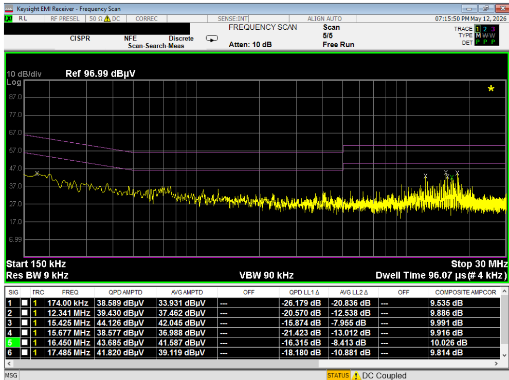
Plot 7-8. Line-Conducted Test Plot (N) – WCP
