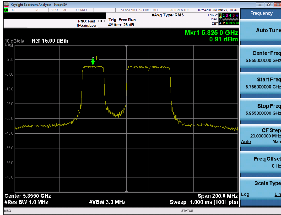
Plot 7-87. Power Spectral Density Plot MIMO ANT1 (80MHz BW 802.11be (20MHz Puncture) (UNII Band 3/4) – Ch. 171)
