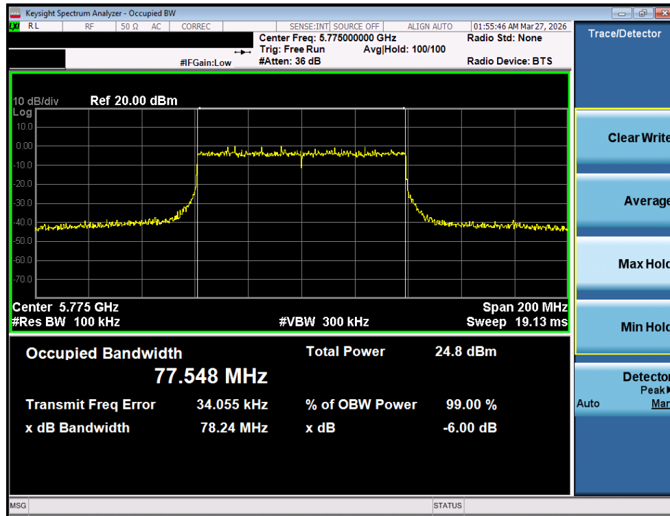
Plot 7-29. 6dB Bandwidth Plot MIMO ANT1 (80MHz BW 802.11be (UNII Band 3) – Ch. 155)
