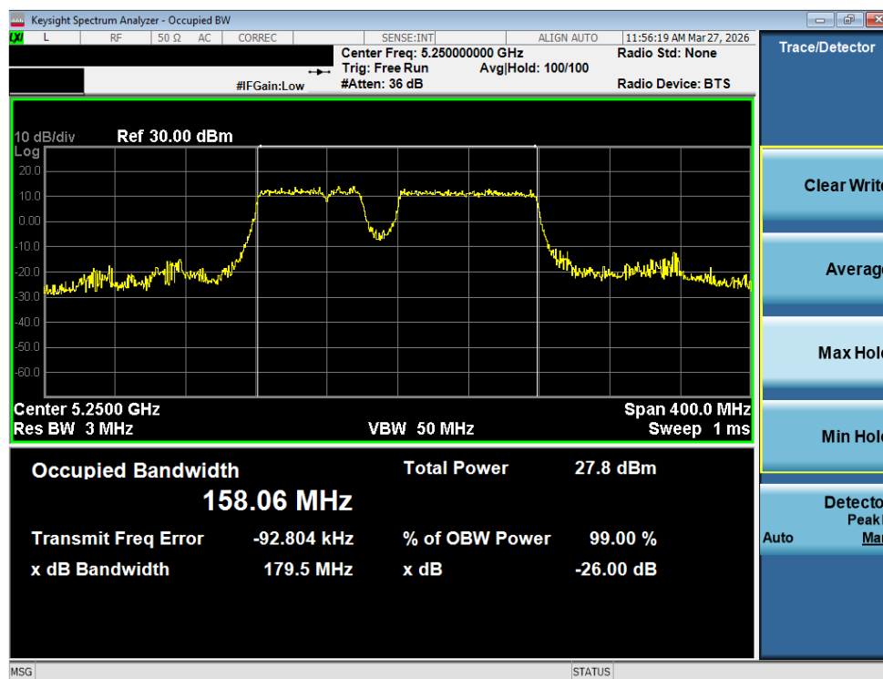
Plot 7-22. 26dB Bandwidth Plot MIMO ANT2 (160MHz BW 802.11be (20MHz Puncture) (UNII Band 1/2A) – Ch. 50)
