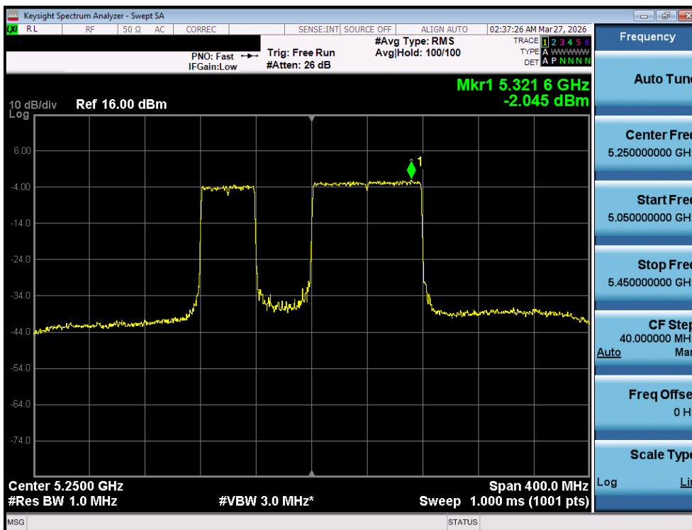
Plot 7-70. Power Spectral Density Plot MIMO ANT1 (160MHz BW 802.11be (40MHz Puncture) (UNII Band 1/2A) – Ch. 50)
