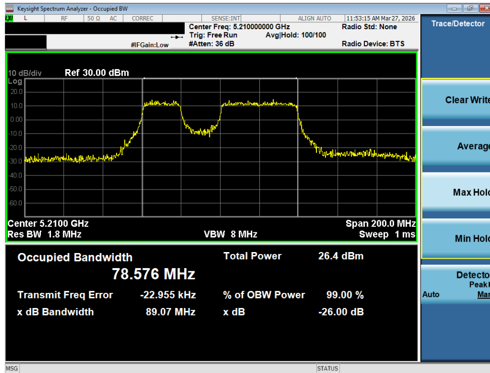
Plot 7-21. 26dB Bandwidth Plot MIMO ANT2 (80MHz BW 802.11be (20MHz Puncture) (UNII Band 1) – Ch. 42)
