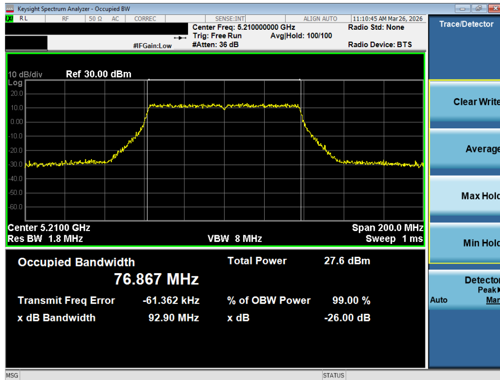
Plot 7-17. 26dB Bandwidth Plot MIMO ANT2 (80MHz BW 802.11ac (UNII Band 1) – Ch. 42)
