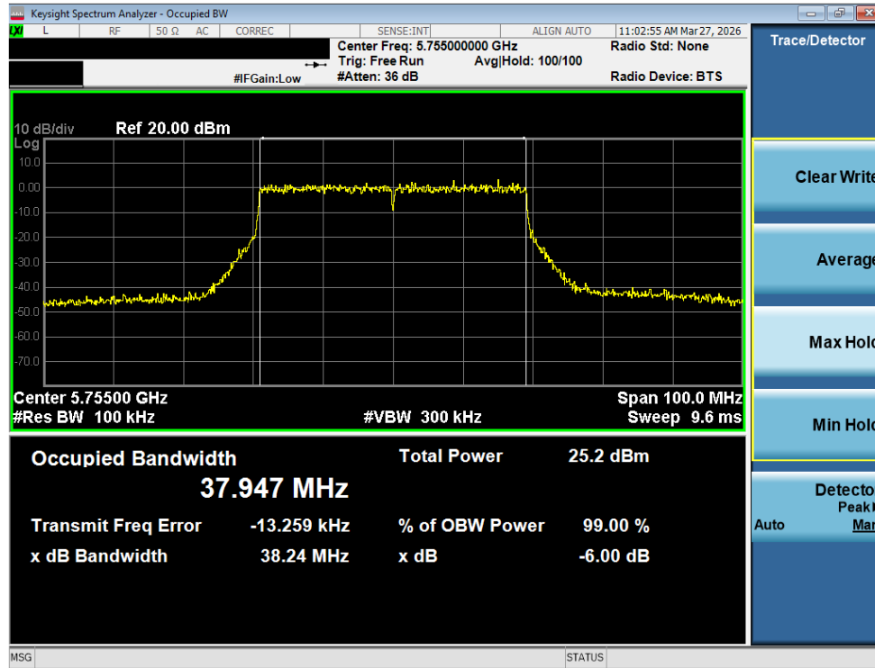
Plot 7-46. 6dB Bandwidth Plot MIMO ANT2 (40MHz BW 802.11be (UNII Band 3) – Ch. 151)
