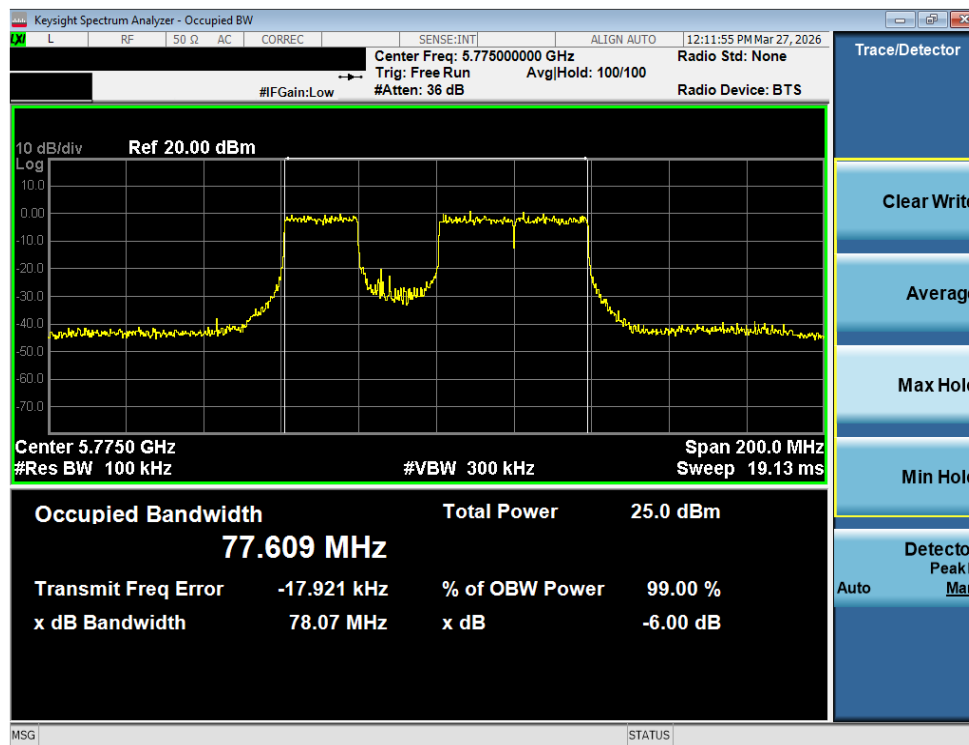
Plot 7-48. 6dB Bandwidth Plot MIMO ANT2 (80MHz BW 802.11be (20MHz Puncture) (UNII Band 3) – Ch. 155)
