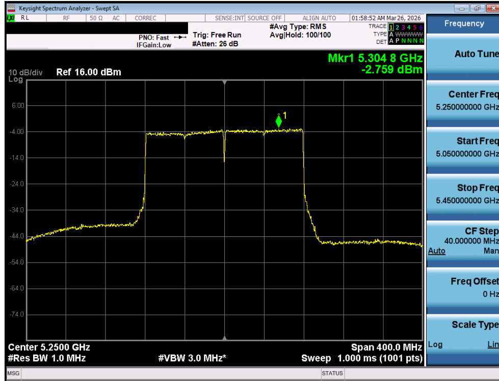
Plot 7-71. Power Spectral Density Plot MIMO ANT1 (160MHz BW 802.11be (UNII Band 1/2A) – Ch. 50)
