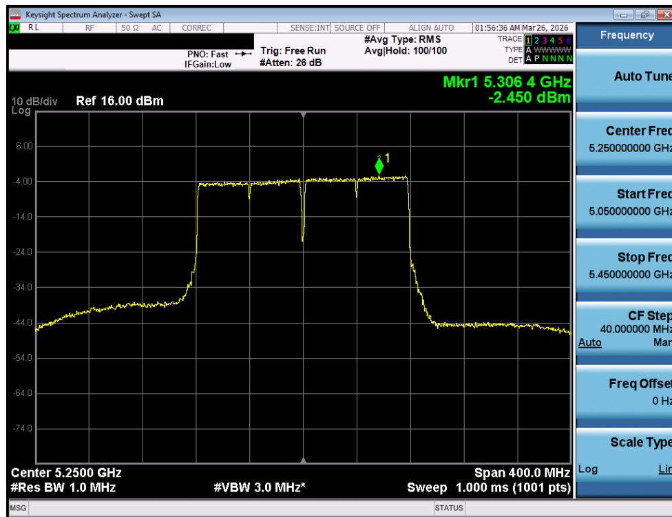
Plot 7-69. Power Spectral Density Plot MIMO ANT1 (160MHz BW 802.11ac (UNII Band 1/2A) – Ch. 50)
