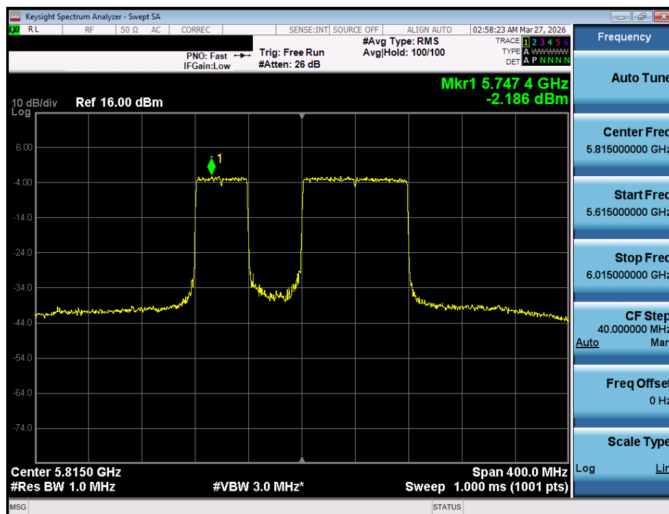
Plot 7-90. Power Spectral Density Plot MIMO ANT1 (160MHz BW 802.11be (40MHz Puncture) (UNII Band 3/4) – Ch. 163)
