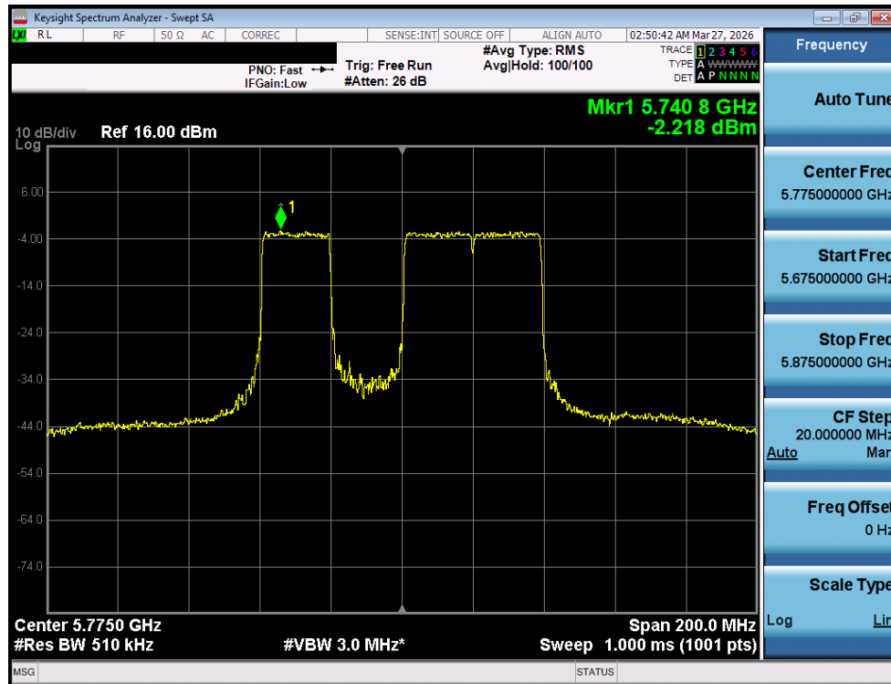
Plot 7-79. Power Spectral Density Plot MIMO ANT1 (80MHz BW 802.11be (20MHz Puncture) (UNII Band 3) – Ch. 155)
