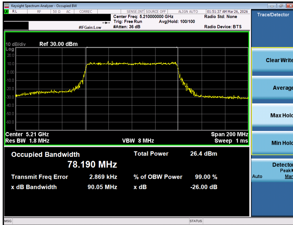
Plot 7-7. 26dB Bandwidth Plot MIMO ANT1 (80MHz BW 802.11be (UNII Band 1) – Ch. 42)
