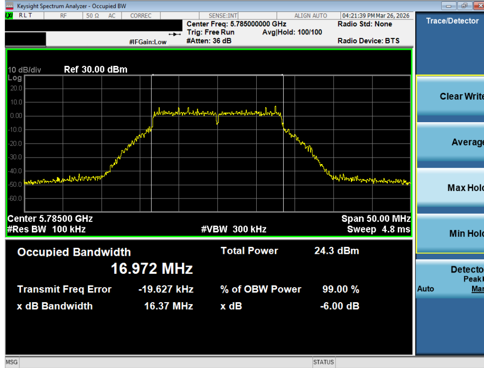
Plot 7-42. 6dB Bandwidth Plot MIMO ANT2 (802.11a (UNII Band 3) – Ch. 157)
