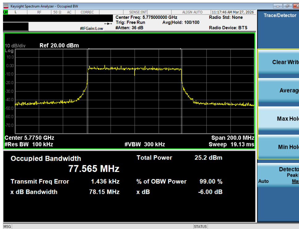
Plot 7-49. 6dB Bandwidth Plot MIMO ANT2 (80MHz BW 802.11be (UNII Band 3) – Ch. 155)
