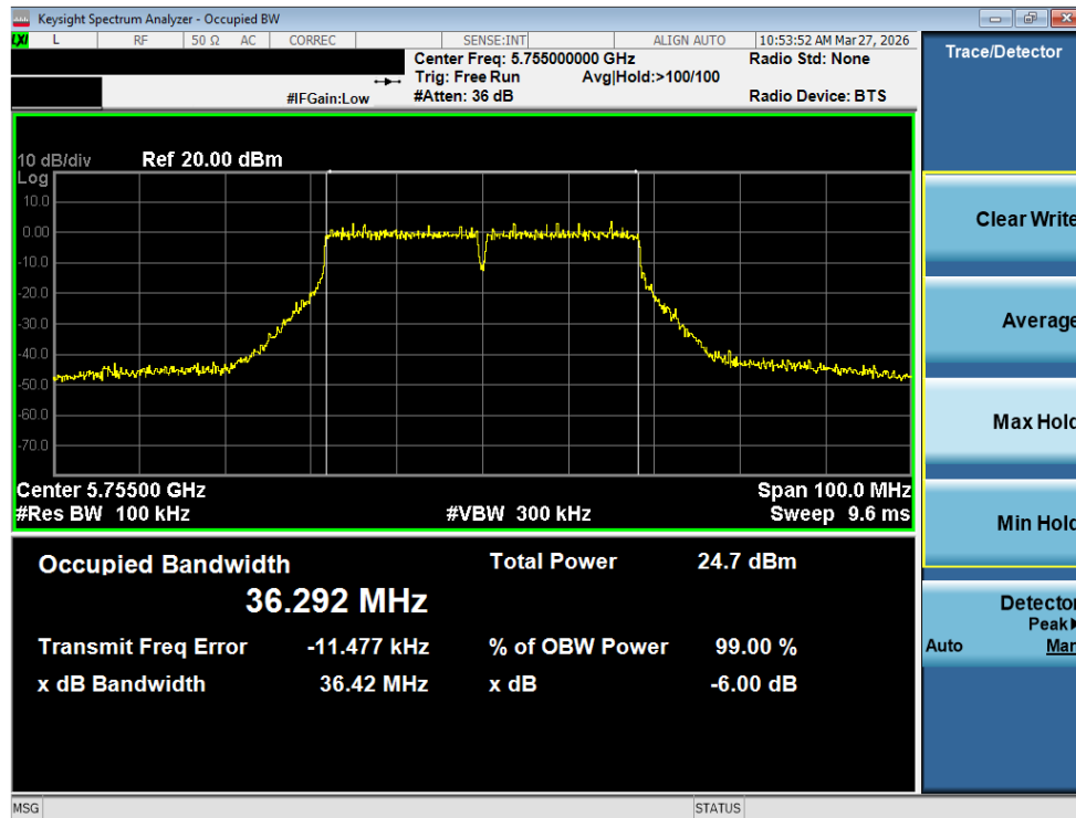
Plot 7-45. 6dB Bandwidth Plot MIMO ANT2 (40MHz BW 802.11n (UNII Band 3) – Ch. 151)
