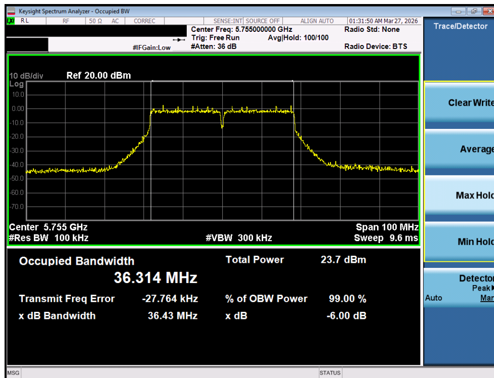
Plot 7-26. 6dB Bandwidth Plot MIMO ANT1 (40MHz BW 802.11n (UNII Band 3) – Ch. 151)
