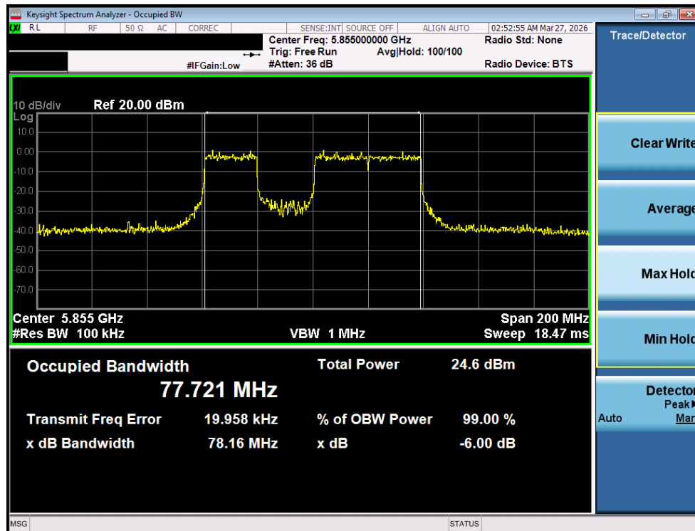
Plot 7-40. 6dB Bandwidth Plot MIMO ANT1 (80MHz BW 802.11be (20MHz Puncture) (UNII Band 3/4) – Ch. 171)
