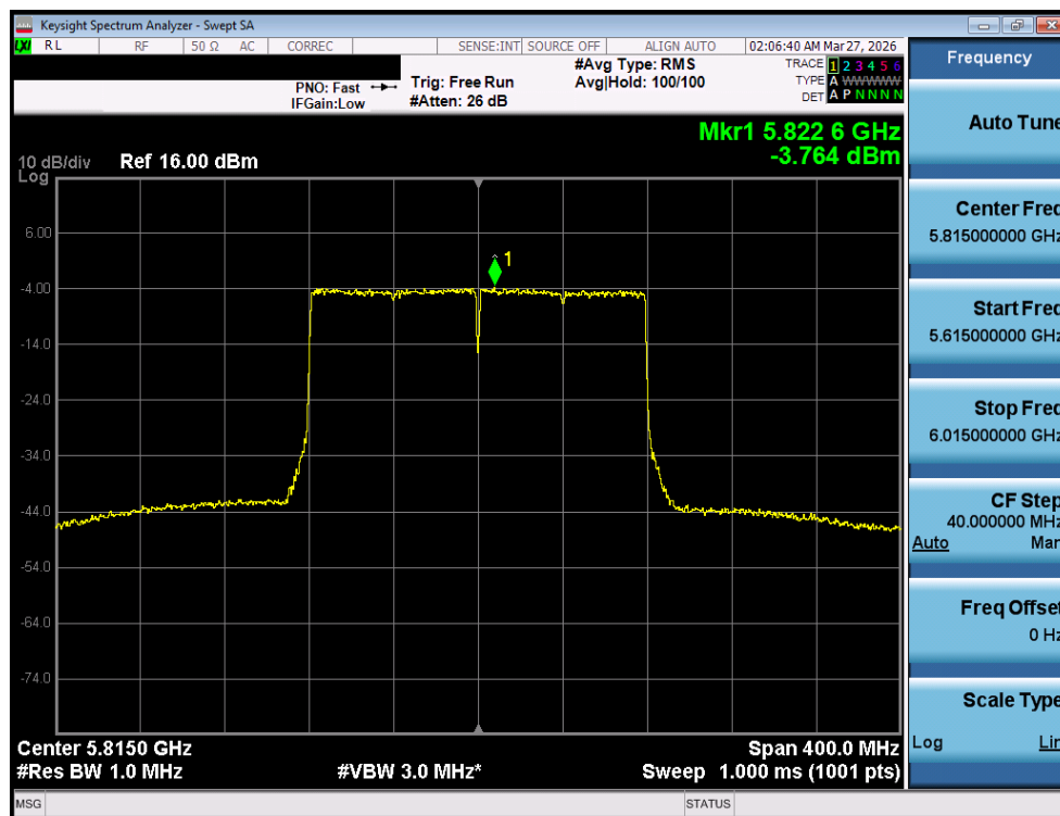
Plot 7-89. Power Spectral Density Plot MIMO ANT1 (160MHz BW 802.11be (UNII Band 3/4) – Ch. 163)
