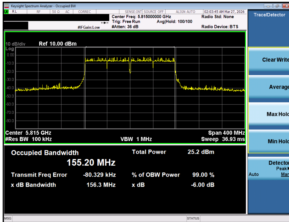
Plot 7-38. 6dB Bandwidth Plot MIMO ANT1 (160MHz BW 802.11ac (UNII Band 3/4) – Ch. 163)
