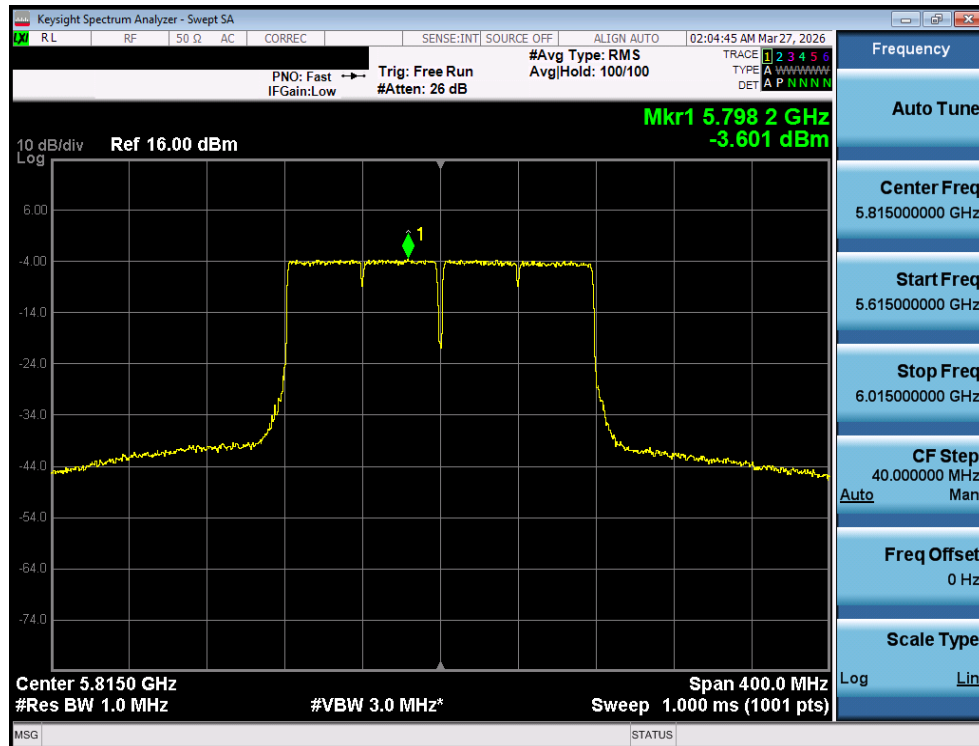
Plot 7-88. Power Spectral Density Plot MIMO ANT1 (160MHz BW 802.11ac (UNII Band 3/4) – Ch. 163)
