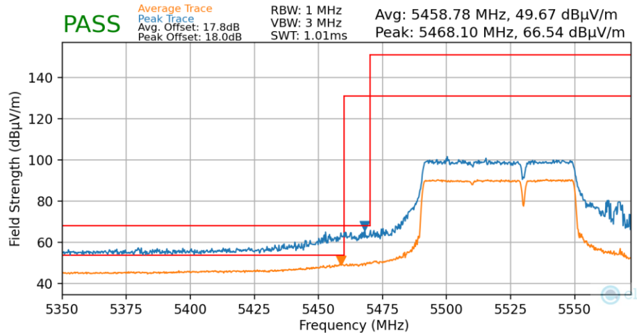
Plot 7-155. Radiated Lower Band Edge Plot MIMO (Average & Peak – UNII Band 2C – Punctured)
