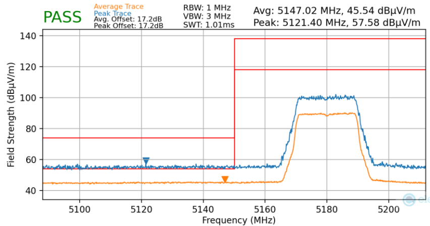
Plot 7-146. Radiated Lower Band Edge Plot MIMO (Average & Peak – UNII Band 1) - WCP
