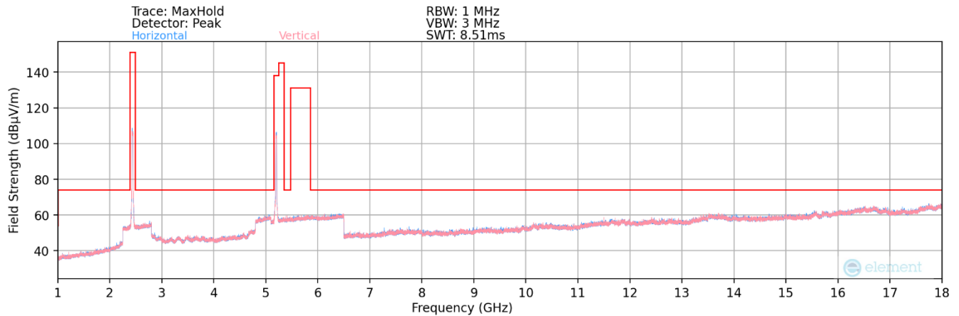
Plot 7-131. Radiated Spurious Plot below 1-18GHz MIMO 802.11b (2.4GHz – Ch.6) + MIMO 802.11a (5GHz – Ch. 120)
