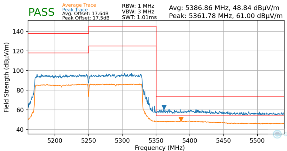
Plot 7-160. Radiated Upper Band Edge Plot MIMO (Average & Peak – UNII Band 2A)
