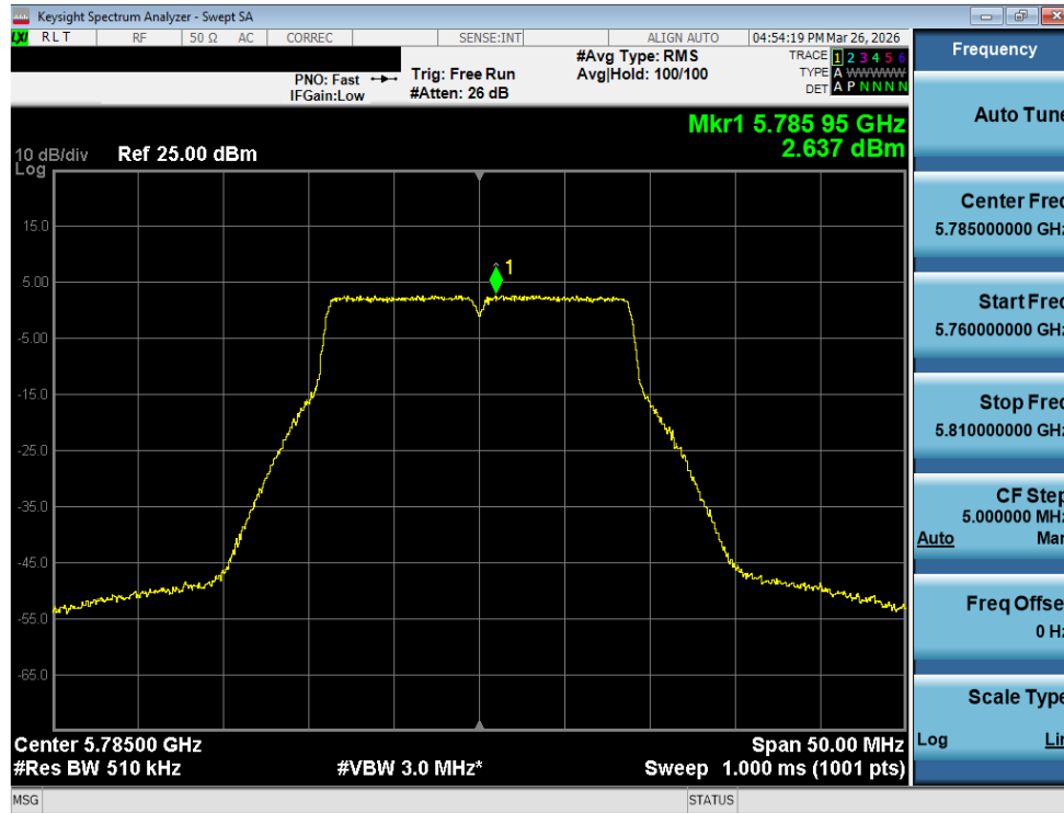
Plot 7-103. Power Spectral Density Plot MIMO ANT2 (20MHz BW 802.11n (UNII Band 3) – Ch. 157)
