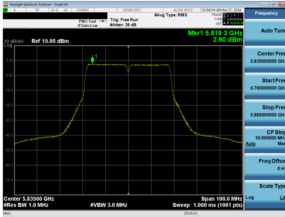
Plot 7-113. Power Spectral Density Plot MIMO ANT2 (40MHz BW 802.11n (UNII Band 3/4) – Ch. 167)
