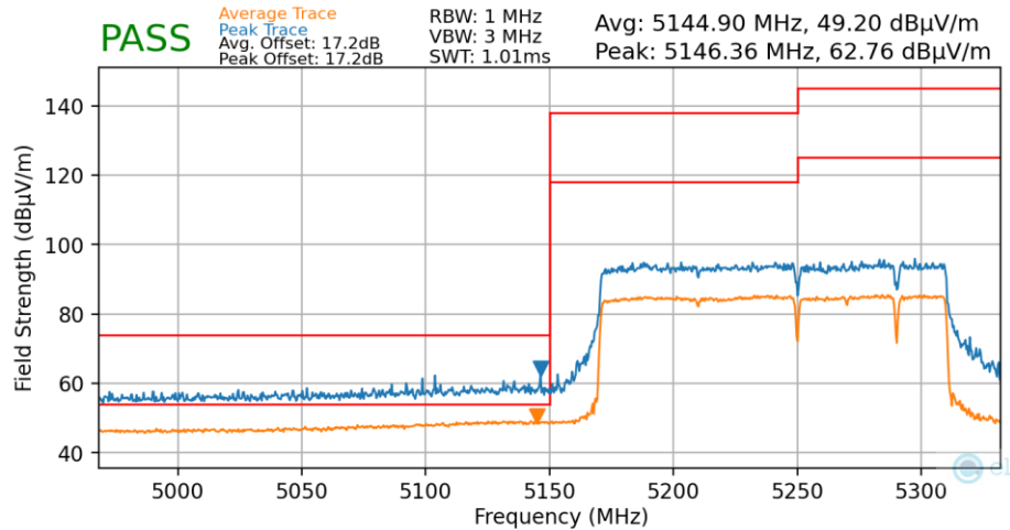
Plot 7-164. Radiated Lower Band Edge Plot MIMO (Average & Peak – UNII Band 1 – Punctured)
