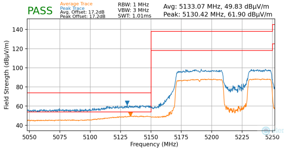
Plot 7-153. Radiated Lower Band Edge Plot MIMO (Average & Peak – UNII Band 1 - Punctured)
