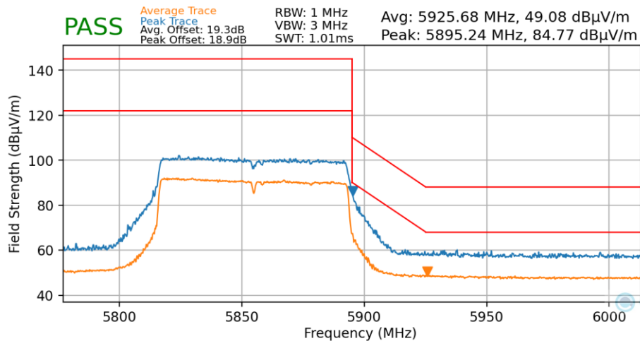
Plot 7-152. Radiated Upper Band Edge Plot MIMO (Average & Peak – UNII Band 4)
