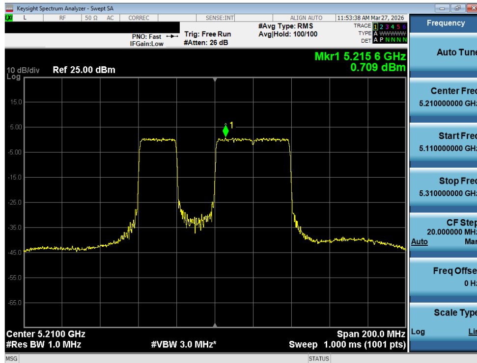
Plot 7-98. Power Spectral Density Plot MIMO ANT2 (80MHz BW 802.11be (20MHz Puncture) (UNII Band 1) – Ch. 42)
