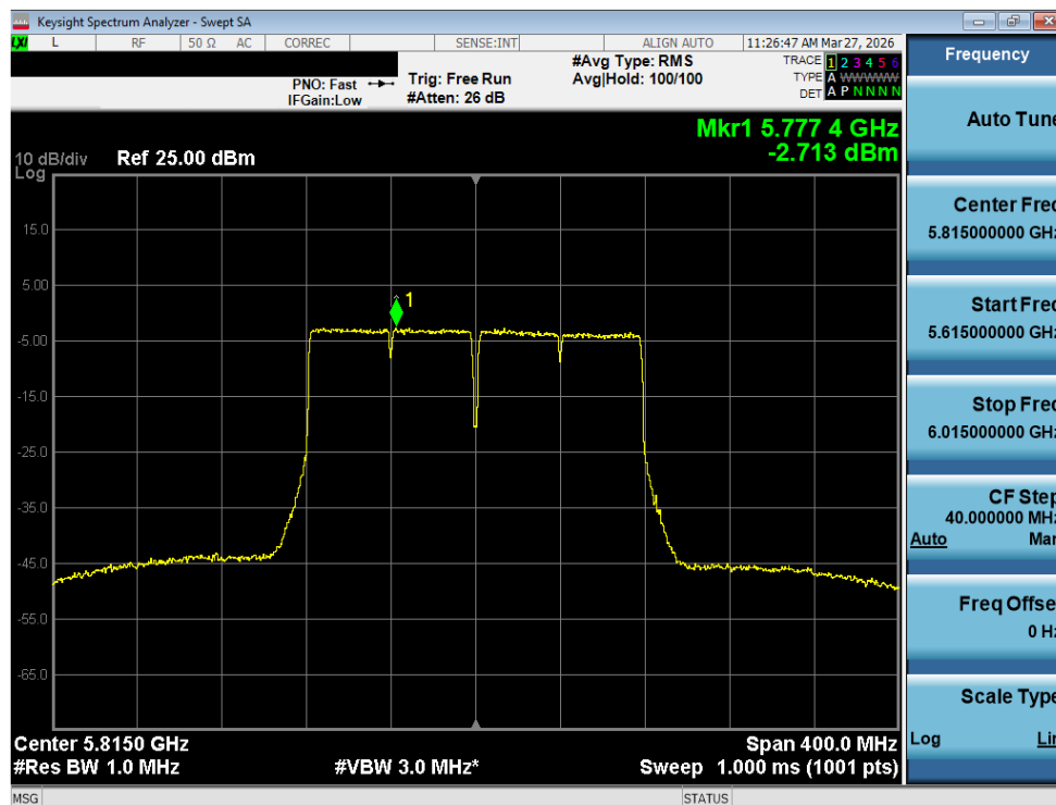
Plot 7-118. Power Spectral Density Plot MIMO ANT2 (160MHz BW 802.11ac (UNII Band 3/4) – Ch. 163)
