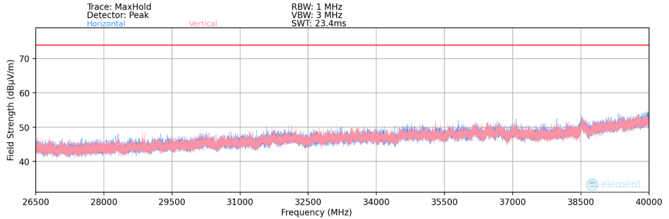
Plot 7-133. Radiated Spurious Plot below 26.5-40GHz MIMO 802.11b (2.4GHz – Ch.6) + MIMO 802.11a (5GHz – Ch. 120)
