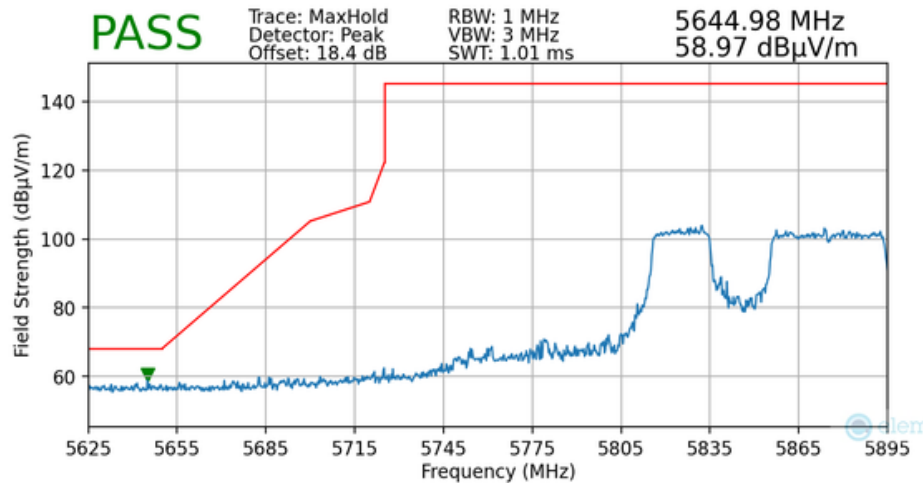
Plot 7-157. Radiated Lower Band Edge Plot MIMO (Peak – UNII Band 4 – Punctured)
