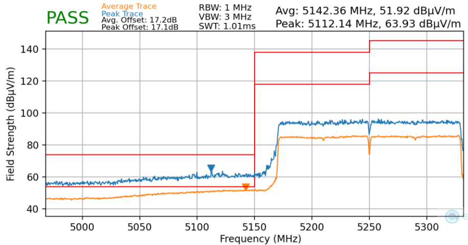
Plot 7-159. Radiated Lower Band Edge Plot MIMO (Average & Peak – UNII Band 1)
