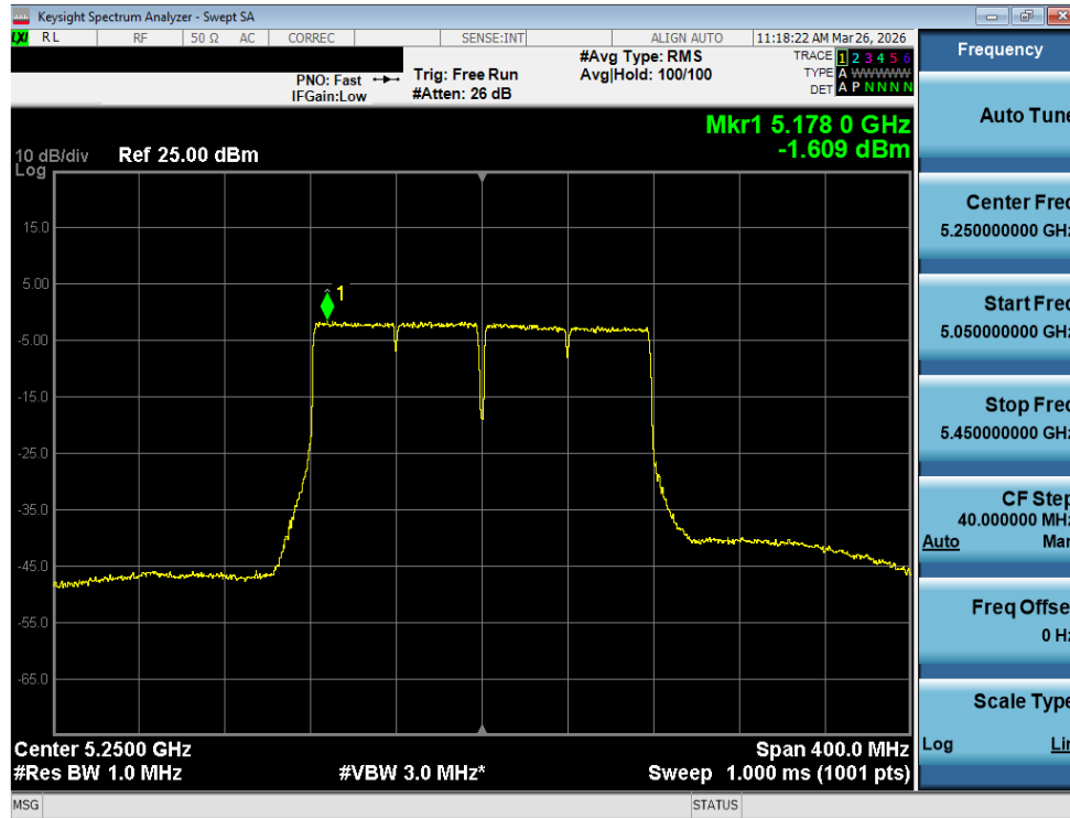
Plot 7-99. Power Spectral Density Plot MIMO ANT2 (160MHz BW 802.11ac (UNII Band 1/2A) – Ch. 50)
