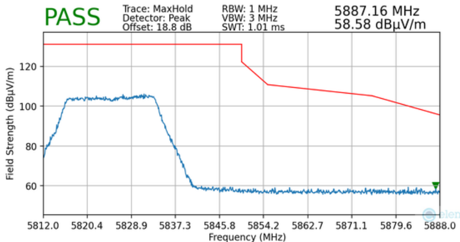
Plot 7-137. Radiated Upper Band Edge Plot MIMO (Peak – UNII Band 3)
