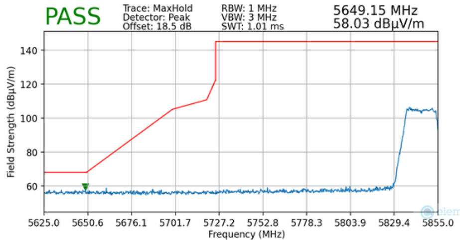
Plot 7-138. Radiated Lower Band Edge Plot MIMO (Peak – UNII Band 4)
