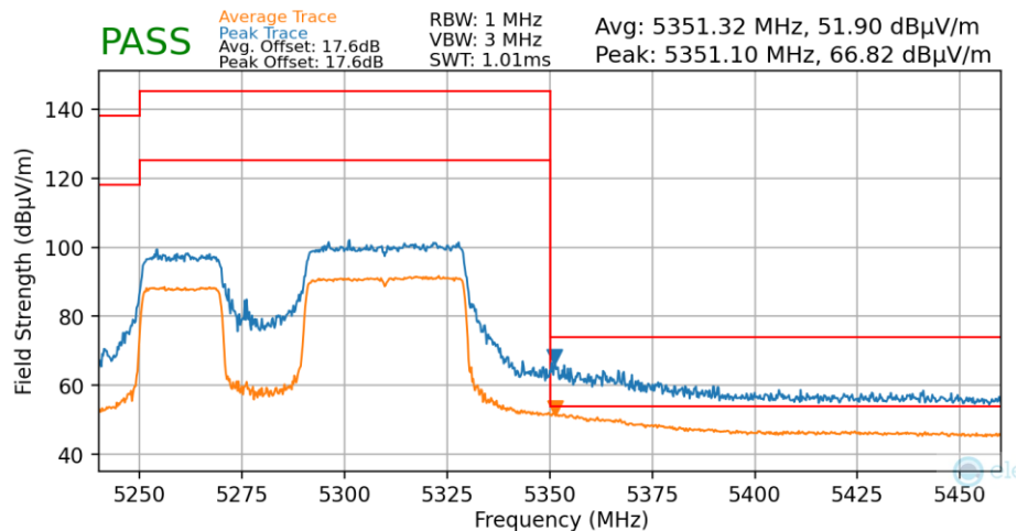
Plot 7-154. Radiated Upper Band Edge Plot MIMO (Average & Peak – UNII Band 2A – Punctured)
