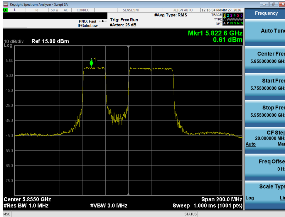
Plot 7-117. Power Spectral Density Plot MIMO ANT2 (80MHz BW 802.11b (20MHz Puncture) (UNII Band 3/4) – Ch. 171)
