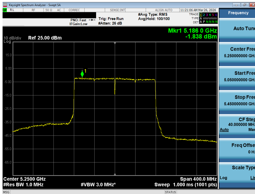
Plot 7-100. Power Spectral Density Plot MIMO ANT2 (160MHz BW 802.11be (UNII Band 1/2A) – Ch. 50)
