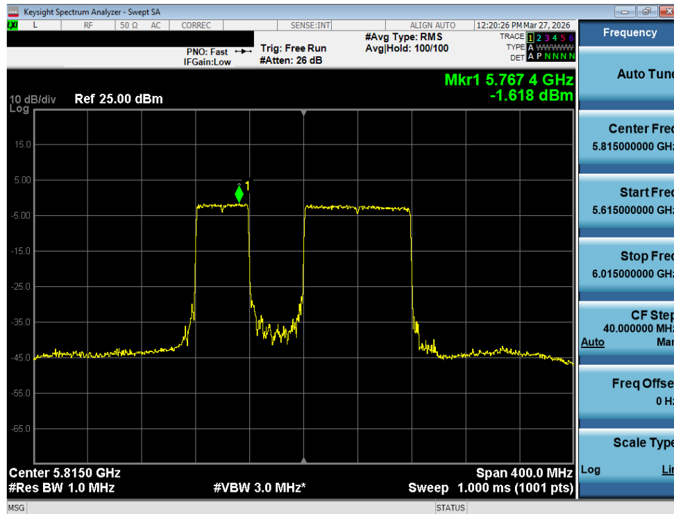
Plot 7-120. Power Spectral Density Plot MIMO ANT2 (160MHz BW 802.11be (40MHz Puncture) (UNII Band 3/4) – Ch. 163)
