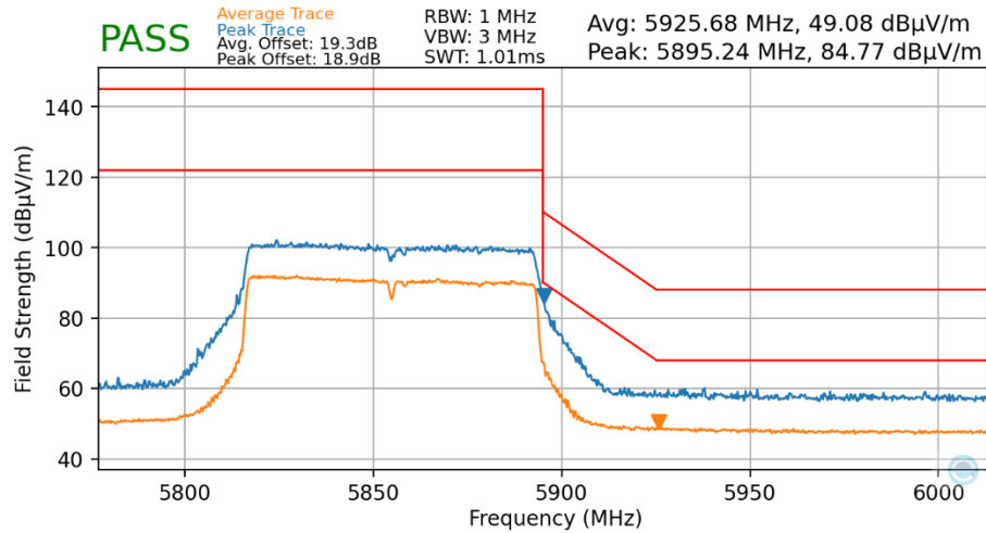
Plot 7-163. Radiated Upper Band Edge Plot MIMO (Average & Peak – UNII Band 4)
