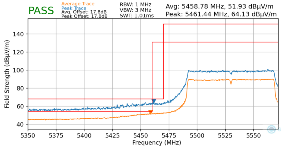
Plot 7-149. Radiated Lower Band Edge Plot MIMO (Average & Peak – UNII Band 2C)
