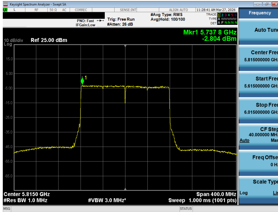
Plot 7-119. Power Spectral Density Plot MIMO ANT2 (160MHz BW 802.11be (UNII Band 3/4) – Ch. 163)
