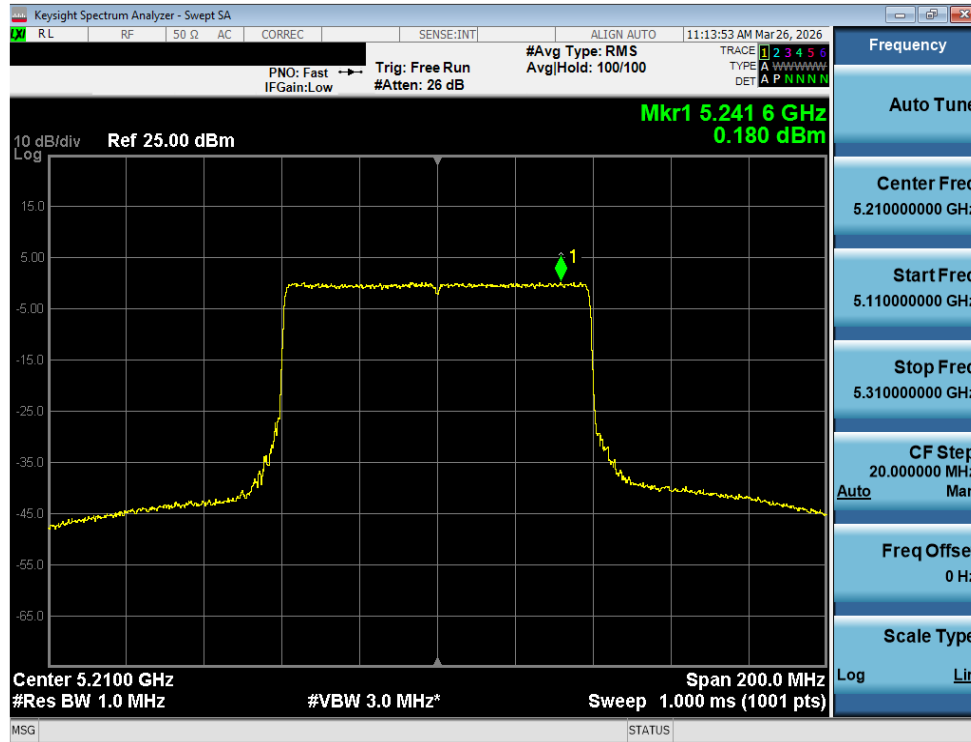
Plot 7-97. Power Spectral Density Plot MIMO ANT2 (80MHz BW 802.11be (UNII Band 1) – Ch. 42)
