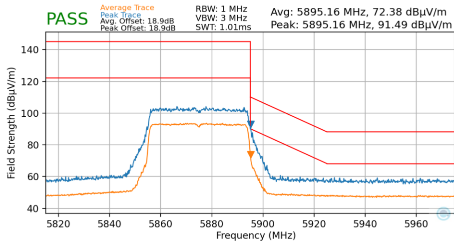
Plot 7-145. Radiated Upper Band Edge Plot MIMO (Average & Peak – UNII Band 4)
