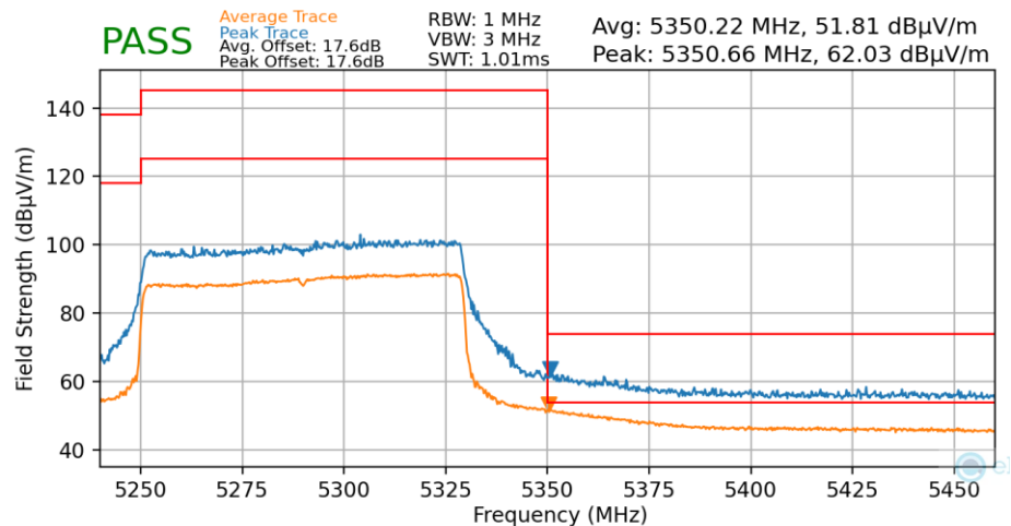
Plot 7-148. Radiated Upper Band Edge Plot MIMO (Average & Peak – UNII Band 2A)
