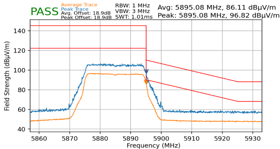
Plot 7-139. Radiated Upper Band Edge Plot MIMO (Average & Peak – UNII Band 4)
