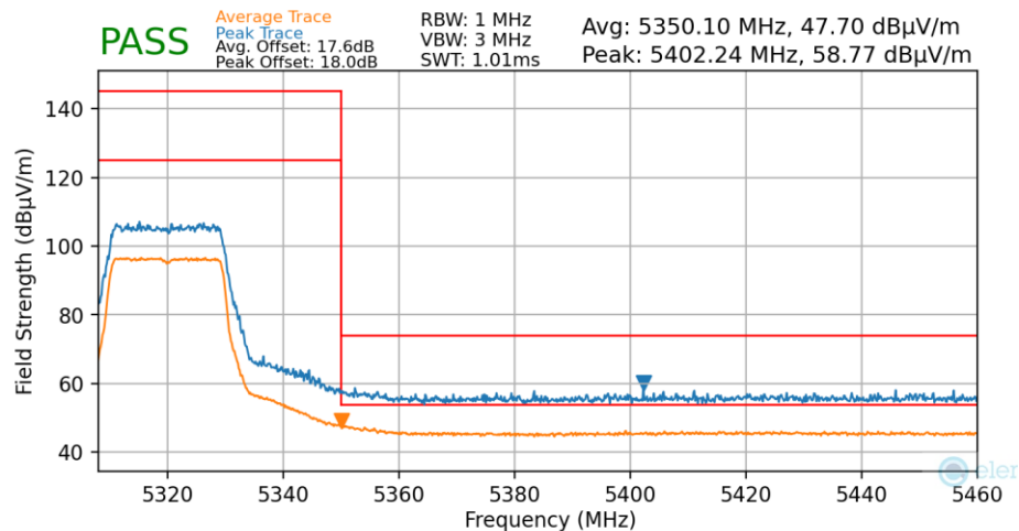
Plot 7-135. Radiated Upper Band Edge Plot MIMO (Average & Peak – UNII Band 2A)
