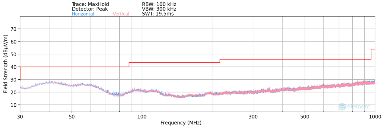
Plot 7-130. Radiated Spurious Plot below 1GHz MIMO 802.11b (2.4GHz – Ch. 6) + MIMO 802.11a (5GHz – Ch. 120)
