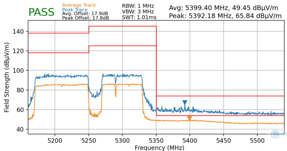
Plot 7-165. Radiated Upper Band Edge Plot MIMO (Average & Peak – UNII Band 2A – Punctured)
