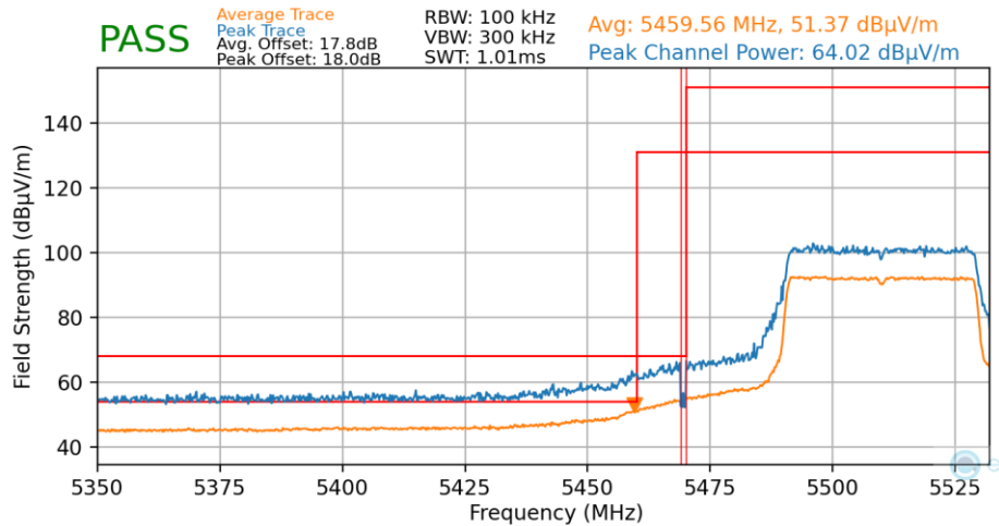
Plot 7-142. Radiated Lower Band Edge Plot MIMO (Average & Peak – UNII Band 2C)
