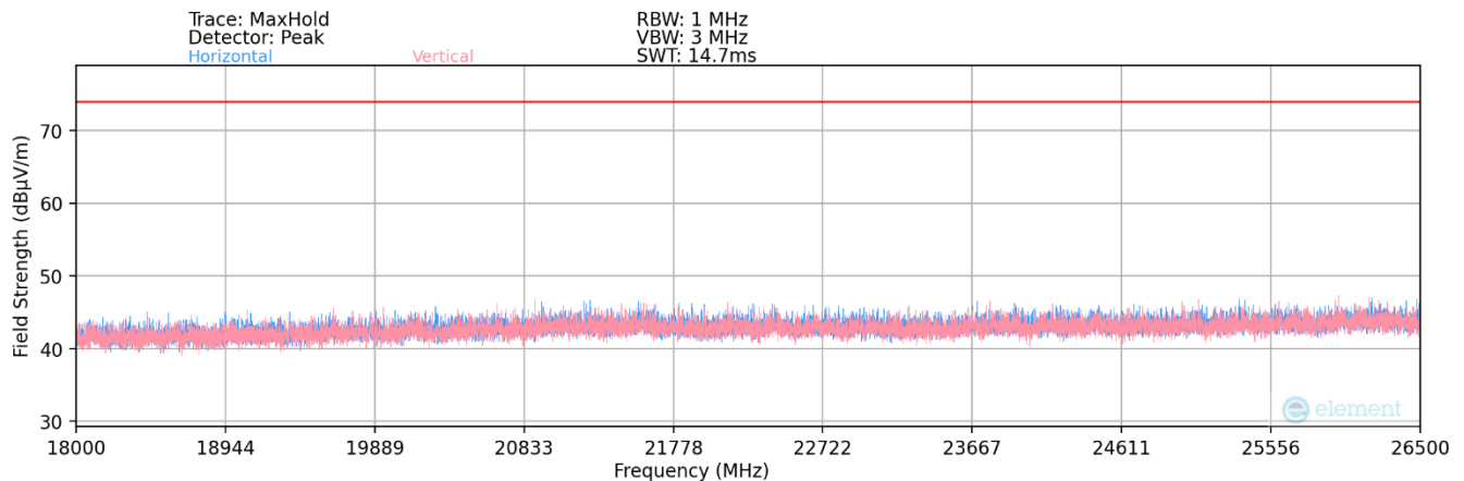
Plot 7-132. Radiated Spurious Plot below 18-26.5GHz MIMO 802.11b (2.4GHz – Ch.6) + MIMO 802.11a (5GHz – Ch. 120)
