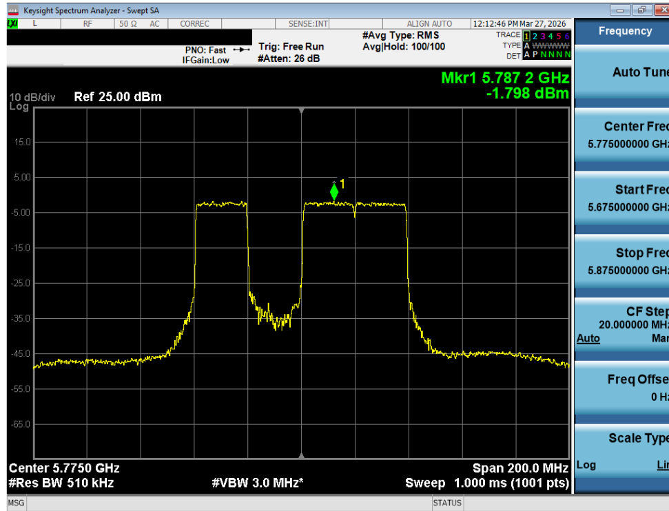
Plot 7-109. Power Spectral Density Plot MIMO ANT2 (80MHz BW 802.11be (20MHz Puncture) (UNII Band 3) – Ch. 155)
