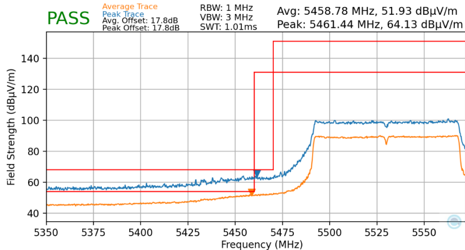
Plot 7-161. Radiated Lower Band Edge Plot MIMO (Average & Peak – UNII Band 2C)
