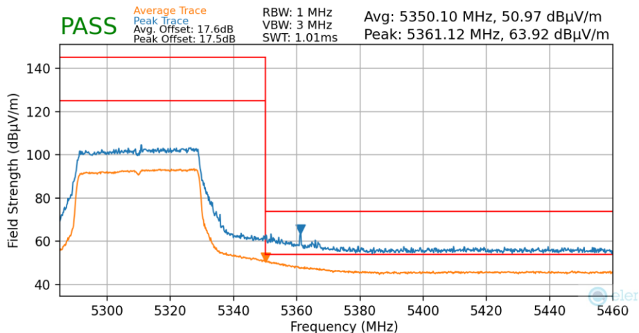
Plot 7-141. Radiated Upper Band Edge Plot MIMO (Average & Peak – UNII Band 2A)
