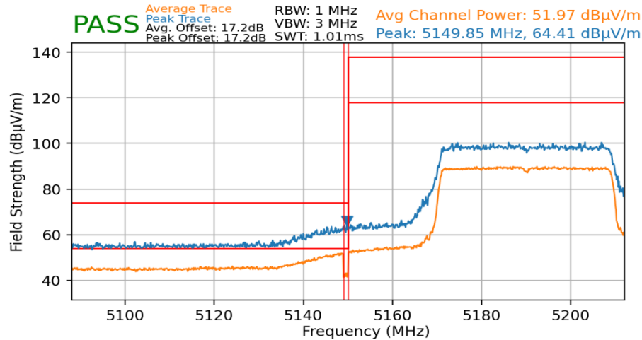
Plot 7-140. Radiated Lower Band Edge Plot MIMO (Average & Peak – UNII Band 1)
