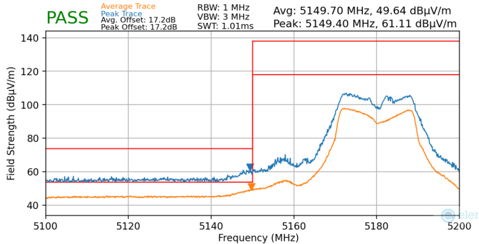
Plot 7-134. Radiated Lower Band Edge Plot MIMO (Average & Peak – UNII Band 1)
