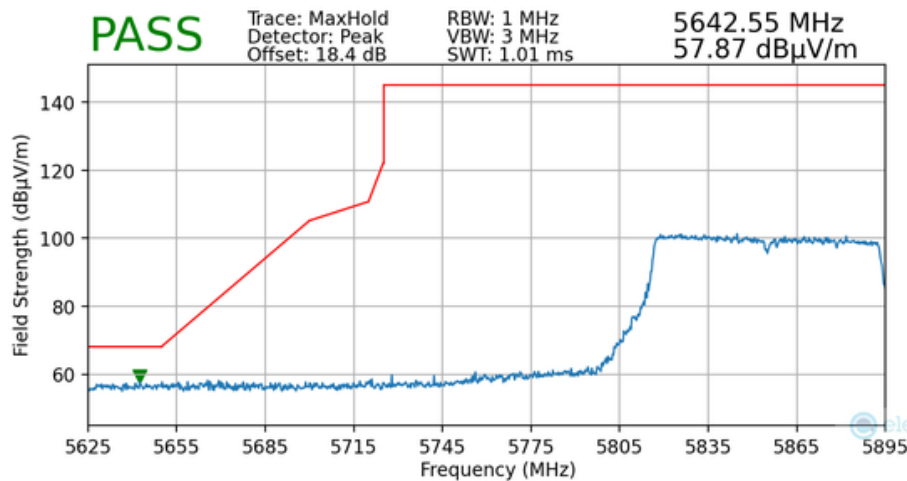
Plot 7-162. Radiated Lower Band Edge Plot MIMO (Peak – UNII Band 4)
