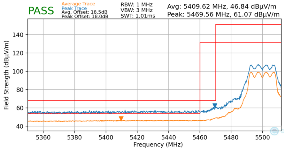
Plot 7-136. Radiated Lower Band Edge Plot MIMO (Average & Peak – UNII Band 2C)
