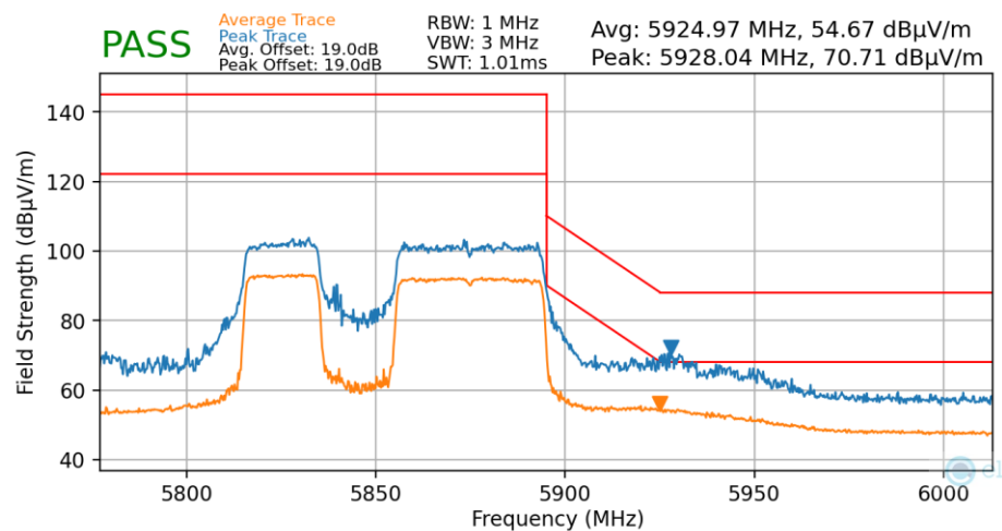
Plot 7-158. Radiated Upper Band Edge Plot MIMO (Average & Peak – UNII Band 4 – Punctured)
