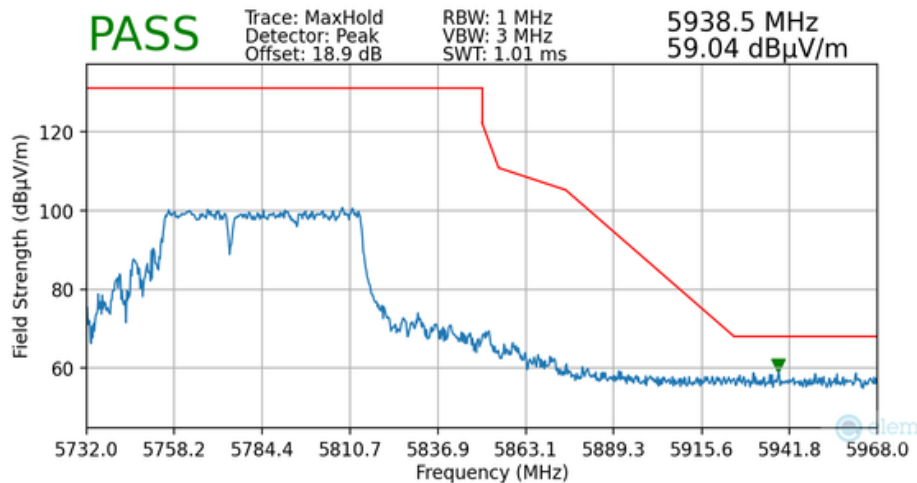
Plot 7-156. Radiated Upper Band Edge Plot MIMO (Peak – UNII Band 3 – Punctured)
