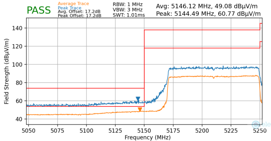
Plot 7-147. Radiated Lower Band Edge Plot MIMO (Average & Peak – UNII Band 1)
