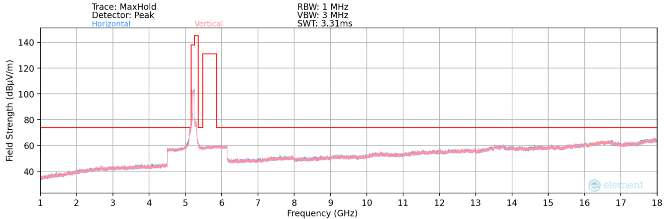
Plot 7-127. Radiated Spurious Plot above 1GHz MIMO (802.11be – UNII Band 1 Ch. 42 – Punctured)
